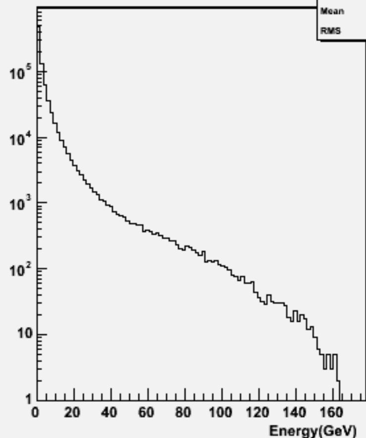
Particle Energy : w102348 uue1e1ss_o
