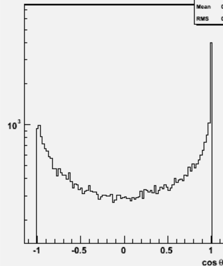
Jet cosθ (All jets)w102348 uue1e1ss_o
