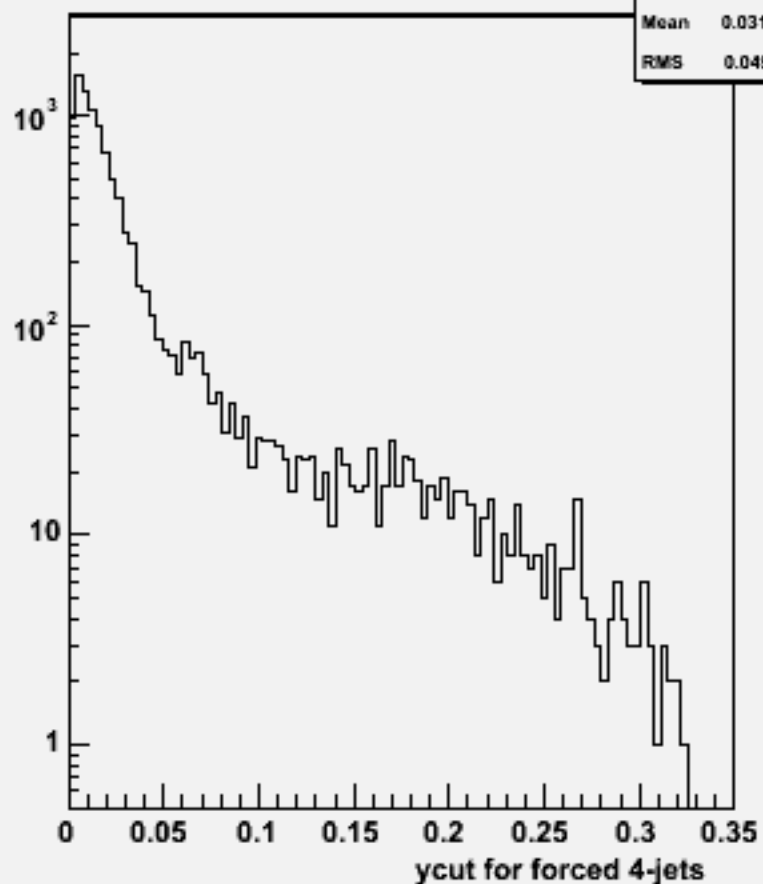
Ycut for 4-jets :w102348 uue1e1ss_o
