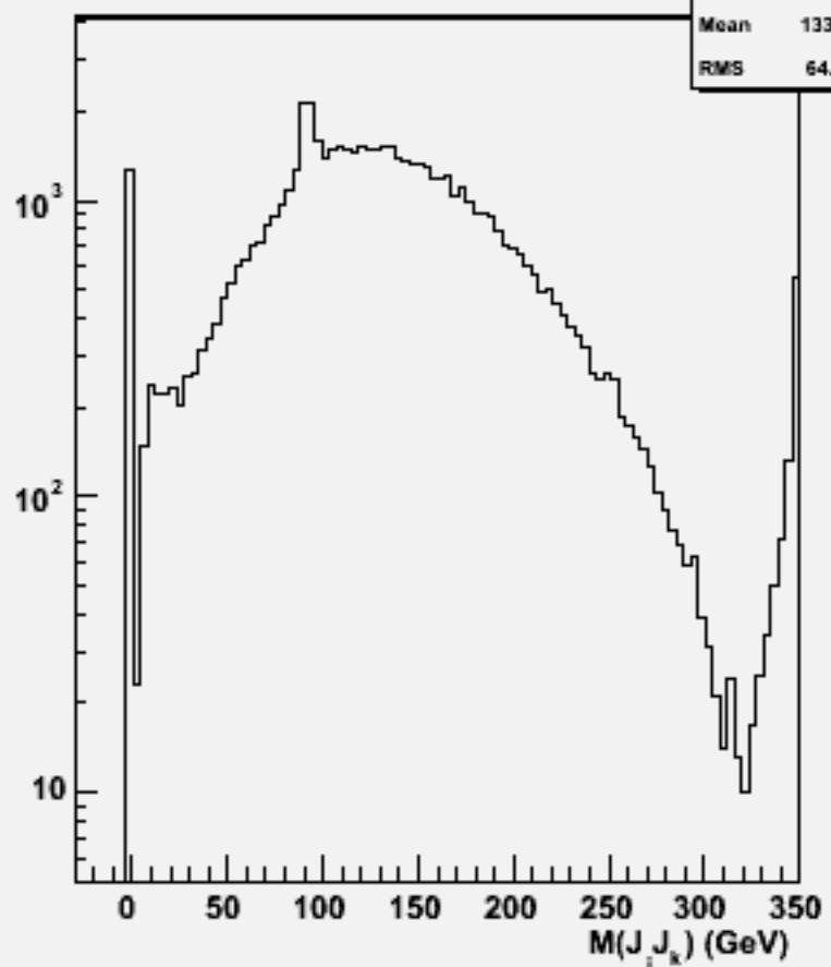
2jets mass(All comb)w102348 uue1e1ss_o
