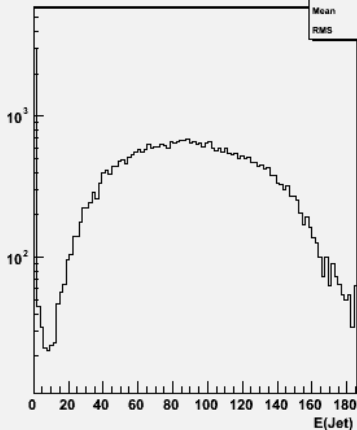
Jet energies(All jets)w102348 uue1e1ss_o
