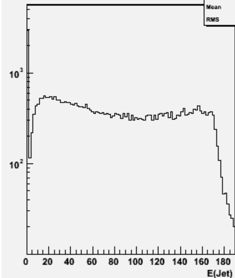
Jet energies(All jets)w102345 uue1e1e3e3_o
