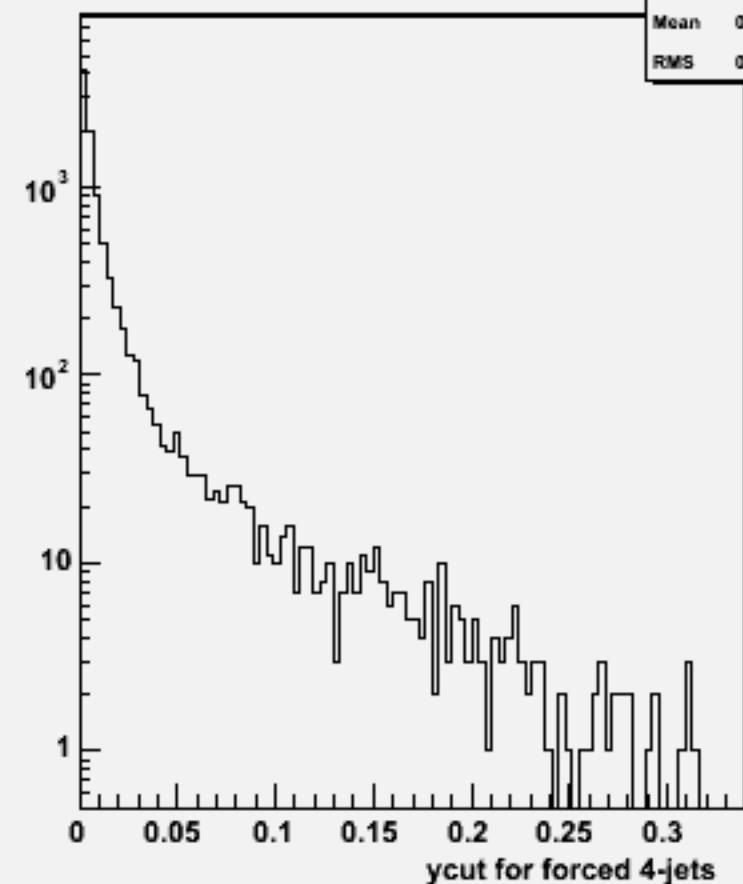
Ycut for 4-jets :w102345 uue1e1e3e3_o
