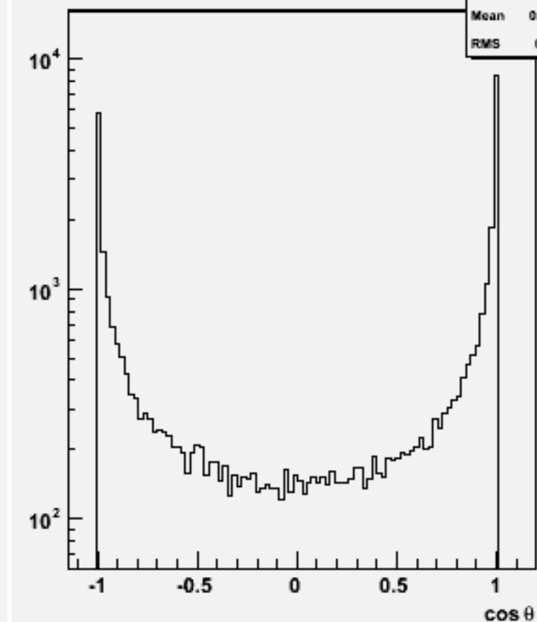
Jet cos \theta (All jets)w102345 uue1e1e3e3_o
