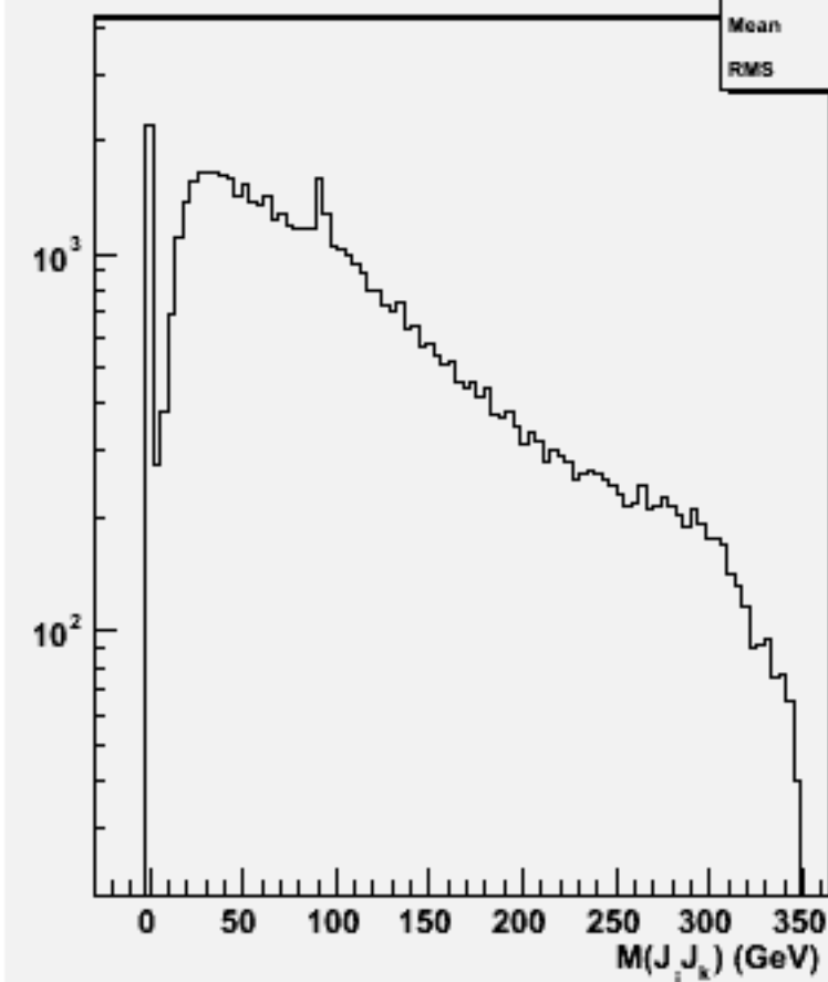
2jets mass(All comb)w102345 uue1e1e3e3_o
