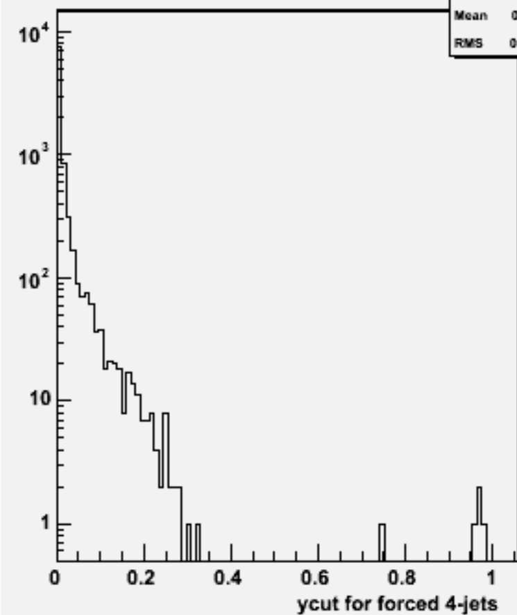
Ycut for 4-jets :w102343 uue1e1e3e3_o
