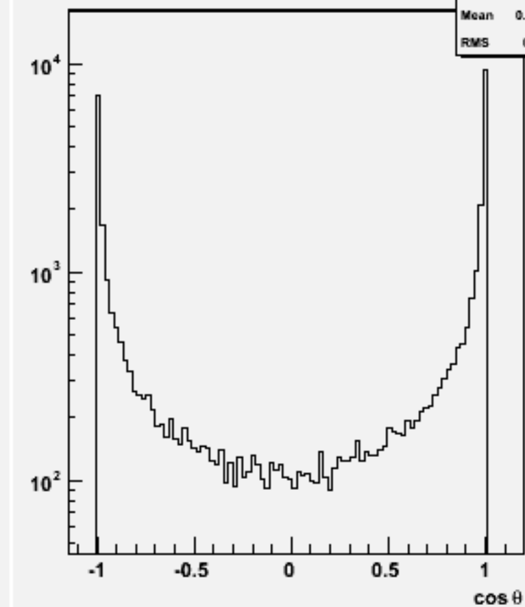
Jet cos \theta (All jets)w102343 uue1e1e3e3_o
