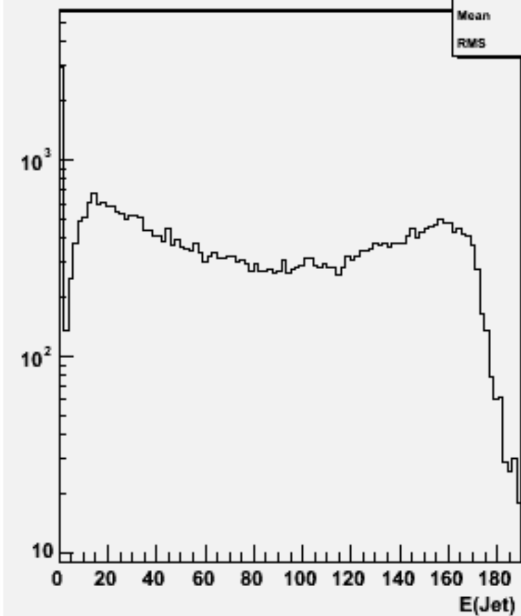
Jet energies(All jets)w102343 uue1e1e3e3_o
