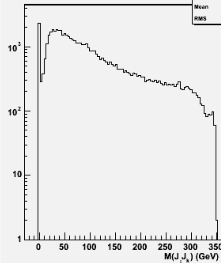
2jets mass(All comb)w102343 uue1e1e3e3_o
