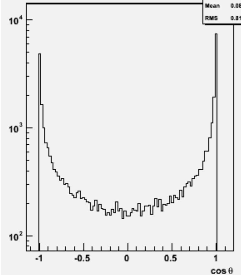
Jet cos \theta (All jets)w102341 uue1e1e2e2_o
