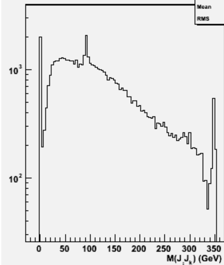
2jets mass(All comb)w102340 uue1e1e2e2_o
