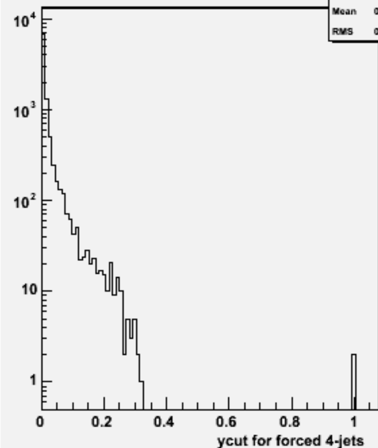
Ycut for 4-jets :w102340 uue1e1e2e2_o
