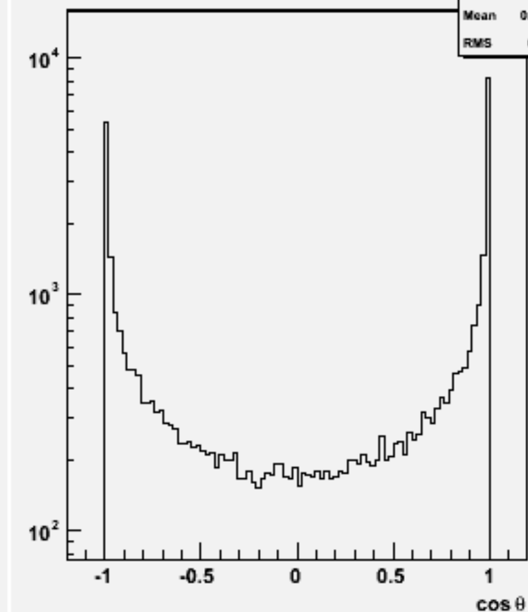
Jet cos \theta (All jets)w102340 uue1e1e2e2_o
