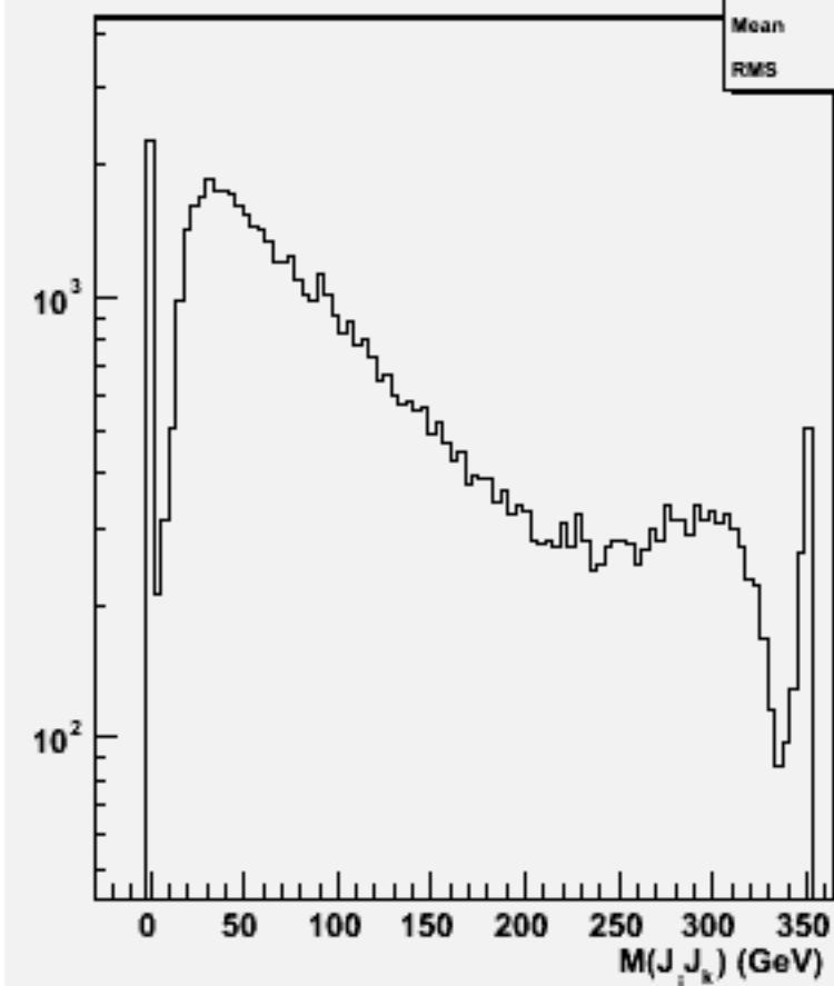
2jets mass(All comb)w102339 uue1e1e2e2_o
