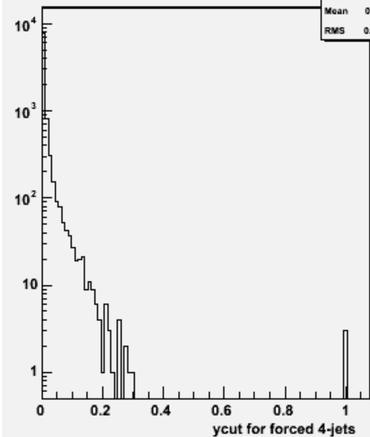
Ycut for 4-jets :w102339 uue1e1e2e2_o
