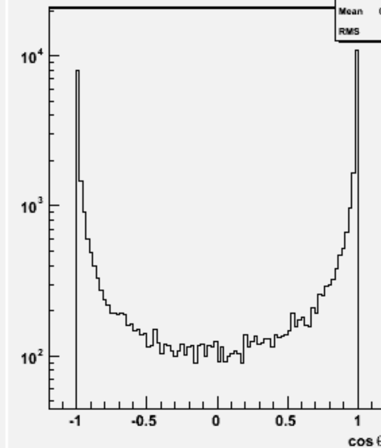
Jet cos \theta (All jets)w102339 uue1e1e2e2_o
