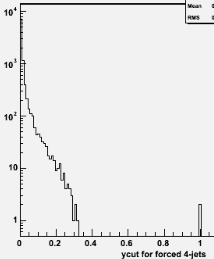
Ycut for 4-jets :w102336 uue1e1e1e1_o
