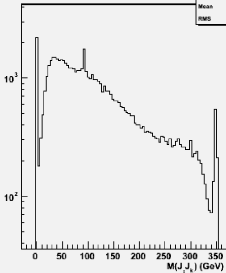
2jets mass(All comb)w102336 uue1e1e1e1_o
