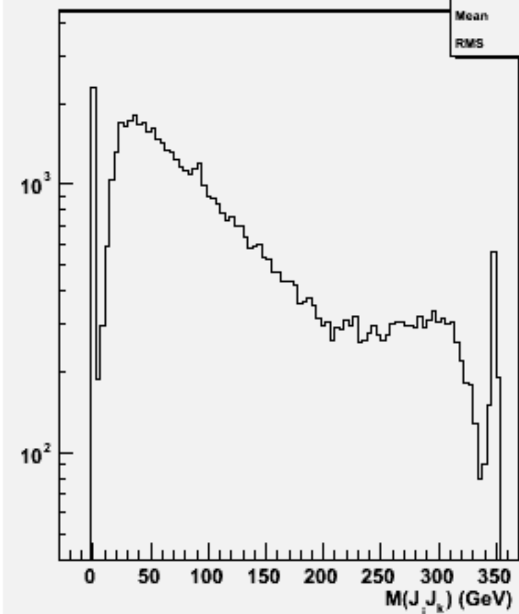
2jets mass(All comb)w102335 uue1e1e1e1_o
