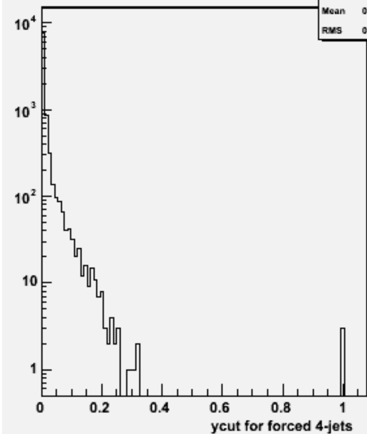
Ycut for 4-jets :w102335 uue1e1e1e1_o
