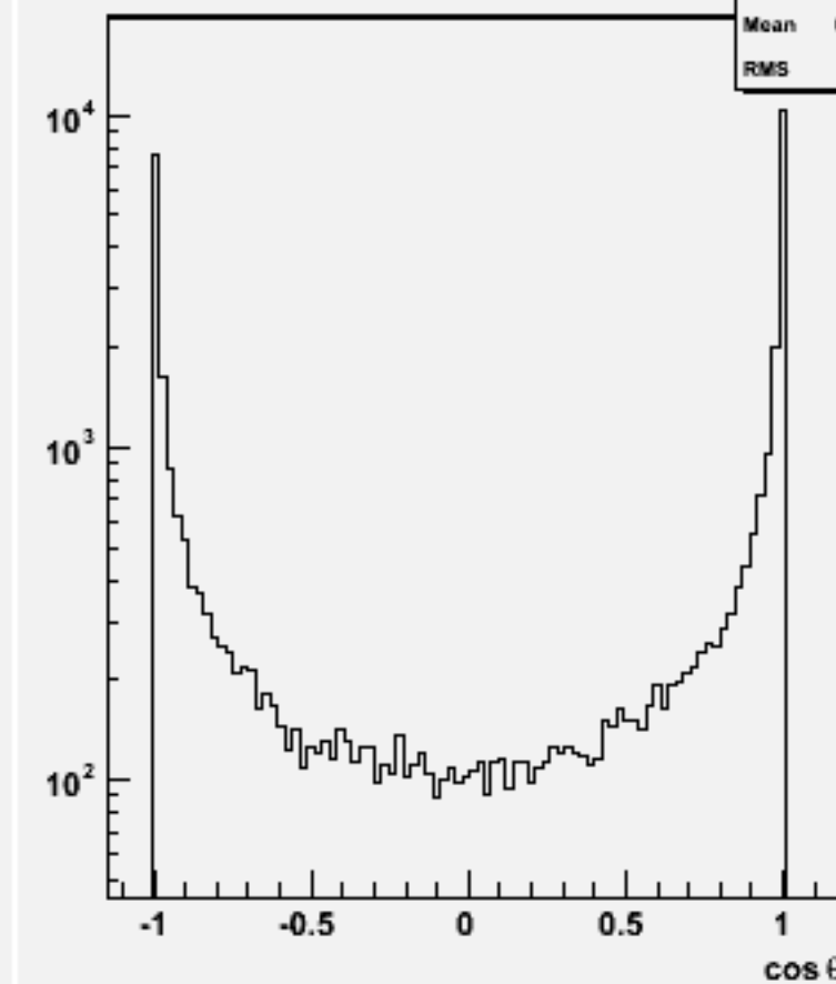
Jet cos \theta (All jets)w102335 uue1e1e1e1_o
