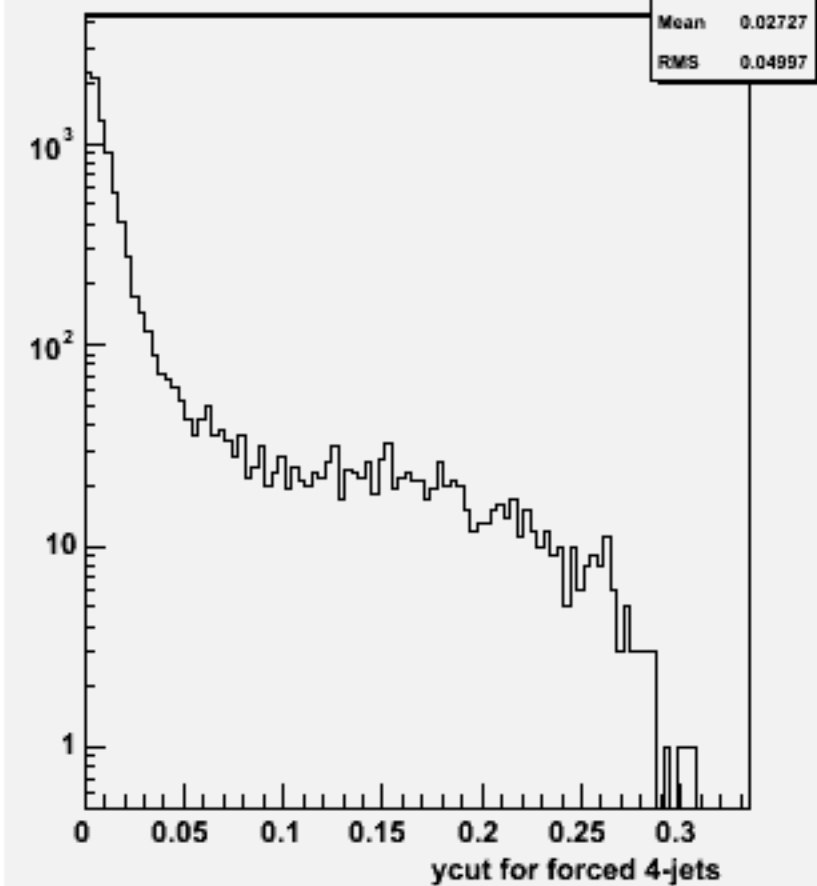
Ycut for 4-jets :w102333 n3n3bbbb_o
