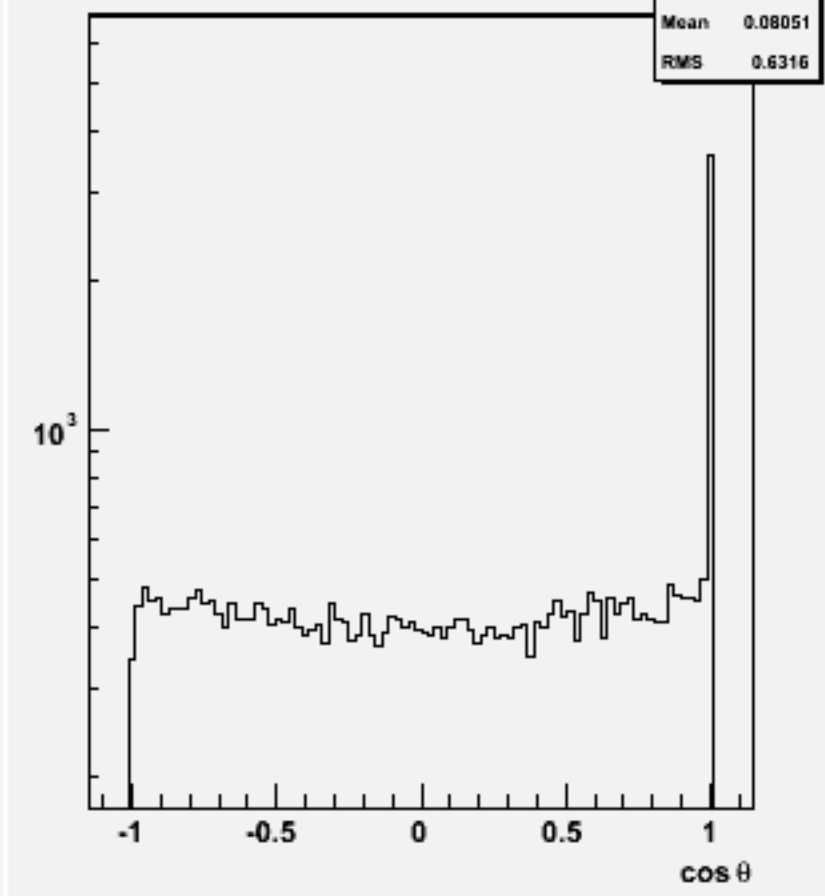
Jet cosθ (All jets)w102332 n3n3bbbb_o
