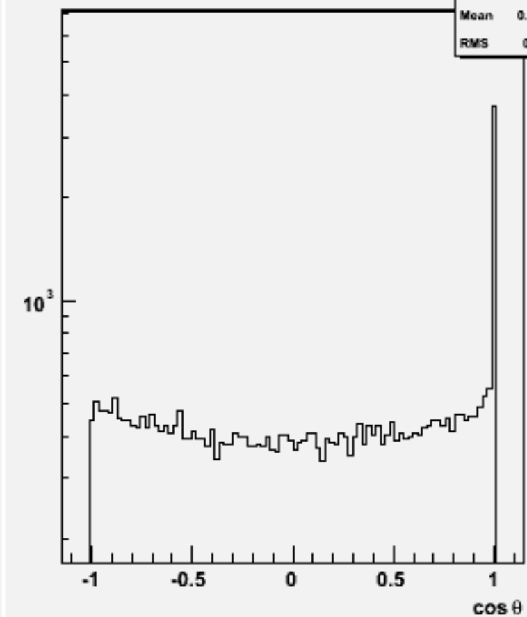
Jet cosθ (All jets)w102329 n3n3ssbb_o
