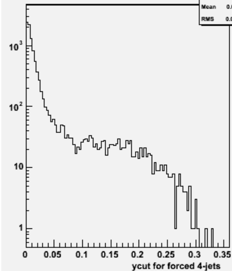
Ycut for 4-jets :w102329 n3n3ssbb_o
