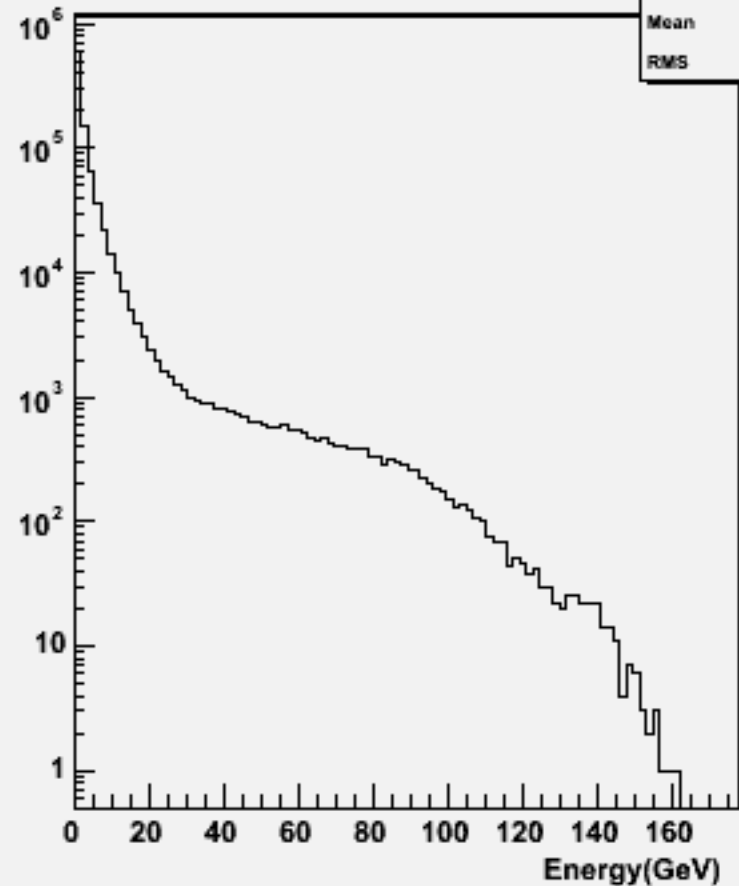
Particle Energy : w102329 n3n3ssbb_o
