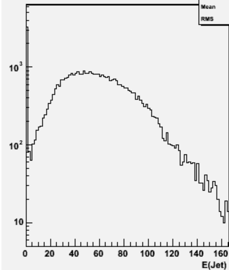
Jet energies(All jets)w102329 n3n3ssbb_o
