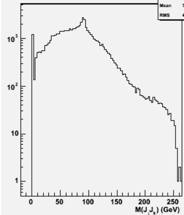
2jets mass(All comb)w102329 n3n3ssbb_o
