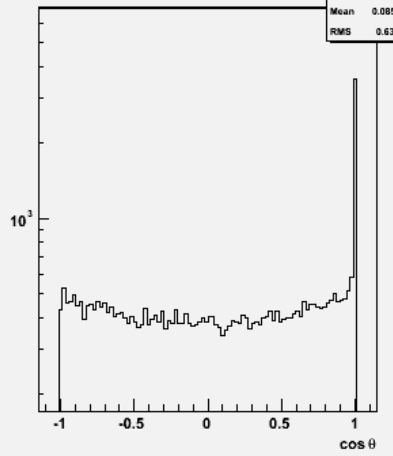
Jet cosθ (All jets)w102321 n3n3ddb_o
