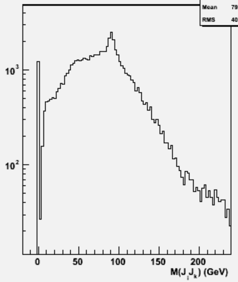
2jets mass(All comb)w102321 n3n3ddb_o
