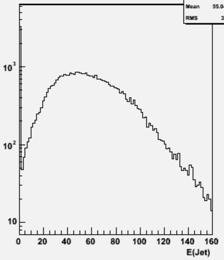
Jet energies(All jets)w102321 n3n3ddb_o
