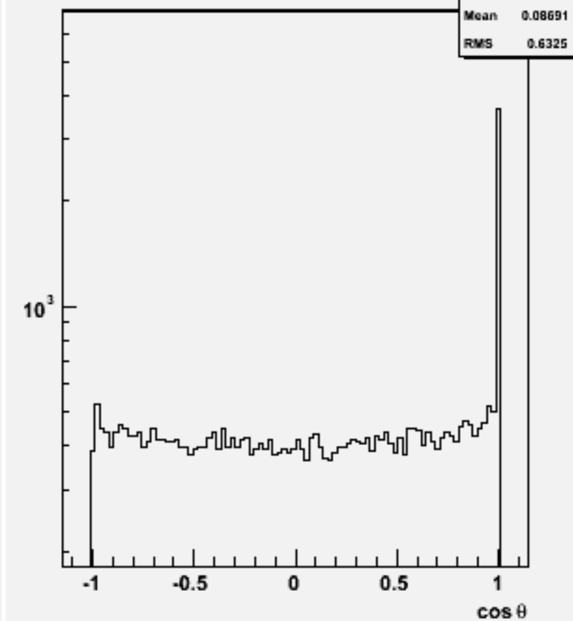
Jet cos \theta (All jets)w102320 n3n3ddb_o
