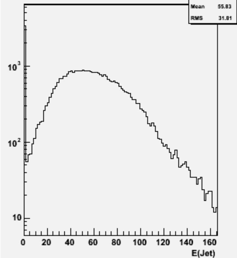
Jet energies(All jets)w102320 n3n3ddb_o
