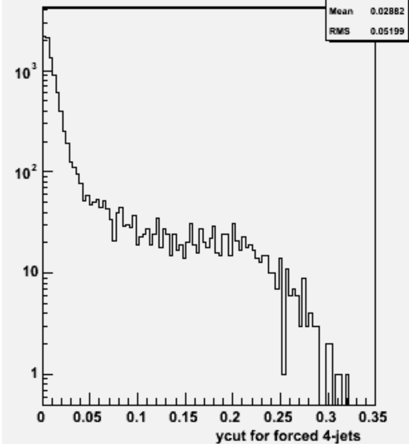
Ycut for 4-jets :w102320 n3n3ddb_o
