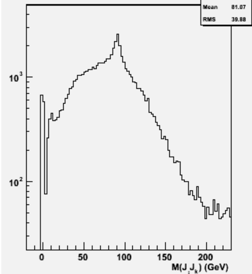
2jets mass(All comb)w102320 n3n3ddb_o
