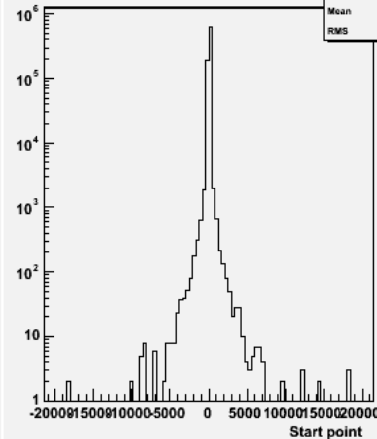
Start point Z : w102313 n3n3dddd_o
