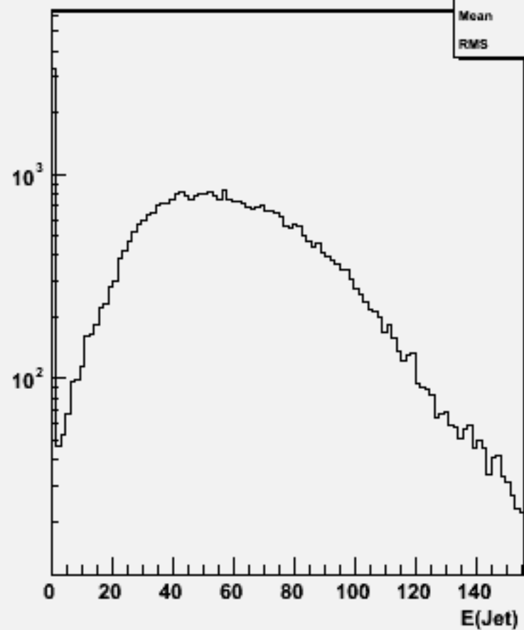
Jet energies(All jets)w102313 n3n3dddd_o
