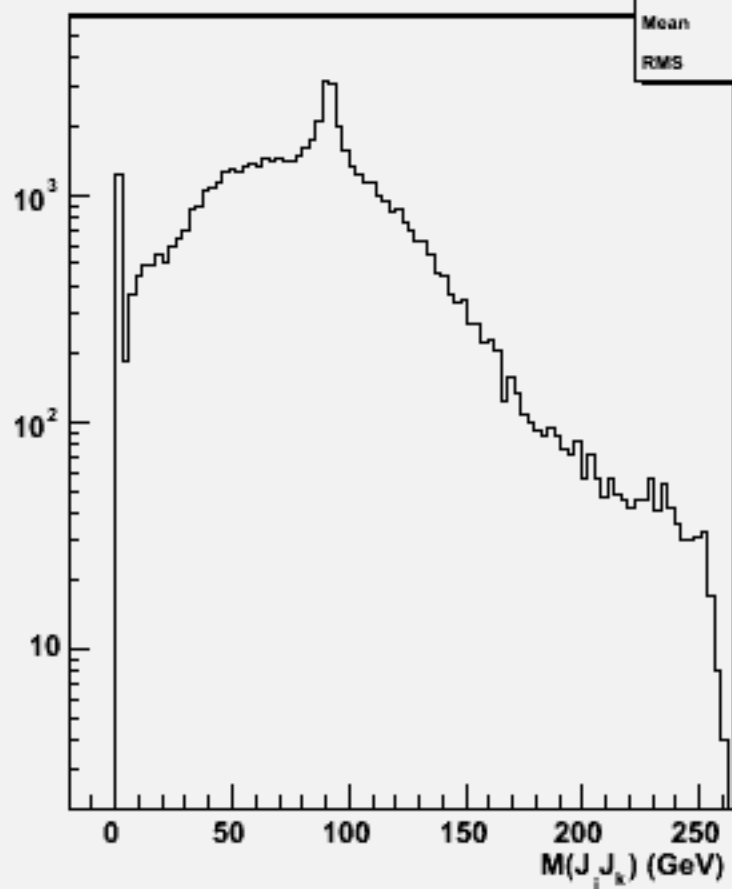
2jets mass(All comb)w102313 n3n3dddd_o
