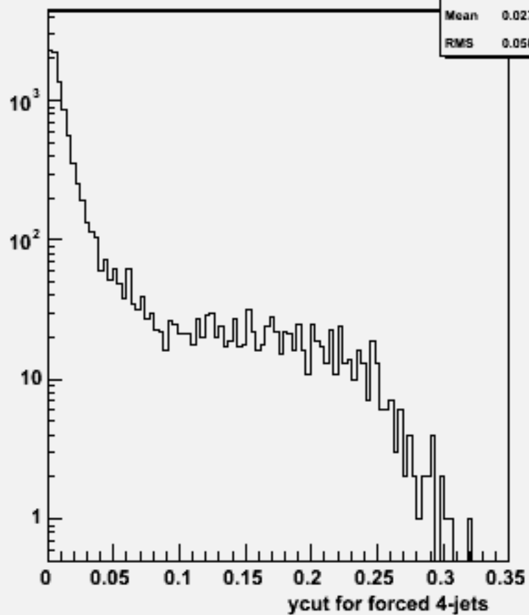
Ycut for 4-jets :w102313 n3n3dddd_o
