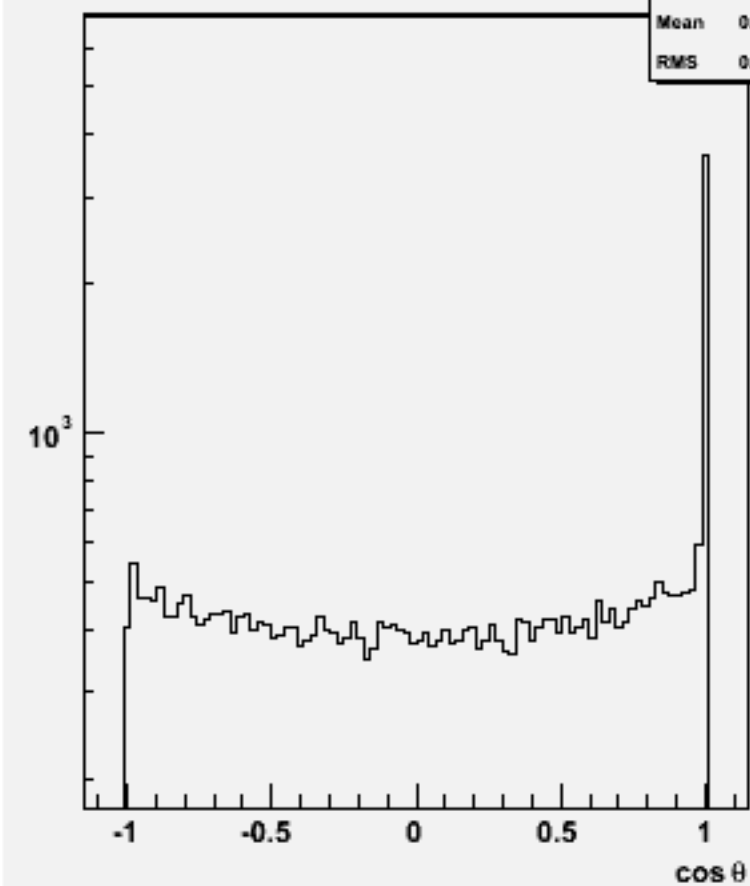
Jet cos \theta (All jets)w102313 n3n3dddd_o
