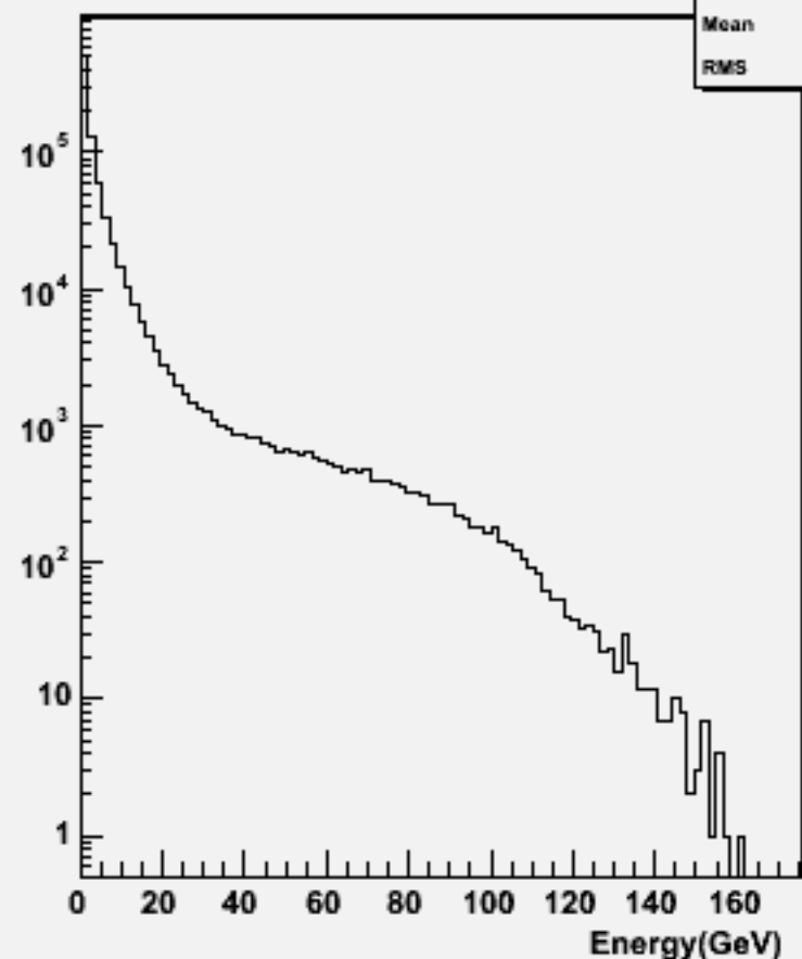
Particle Energy : w102313 n3n3dddd_o
