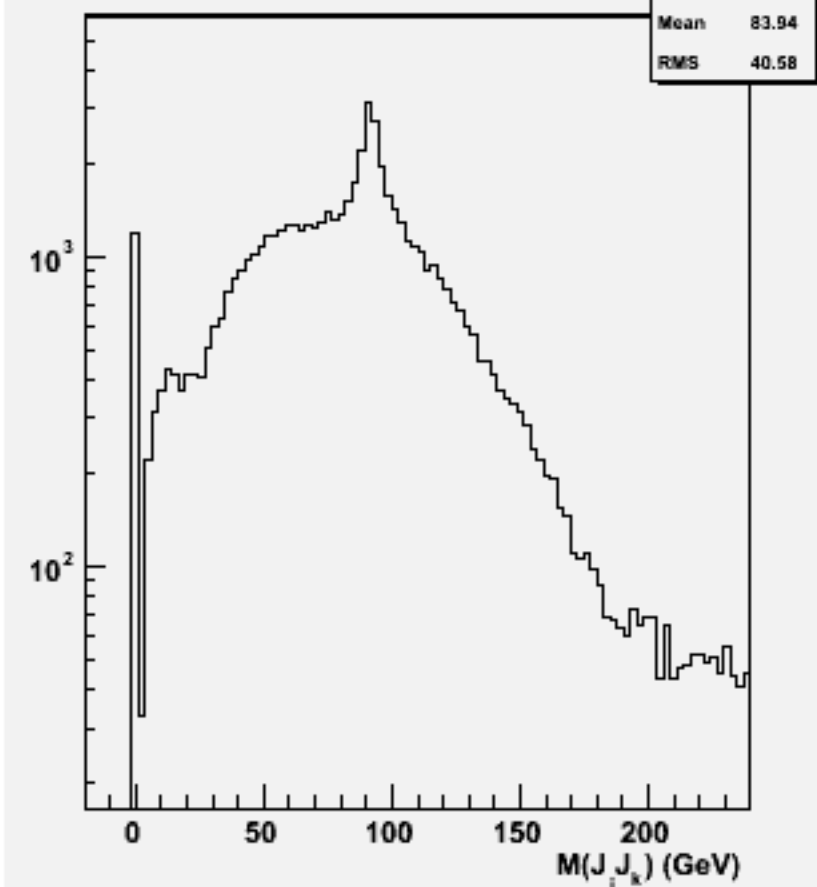
2jets mass(All comb)w102312 n3n3dddd_o
