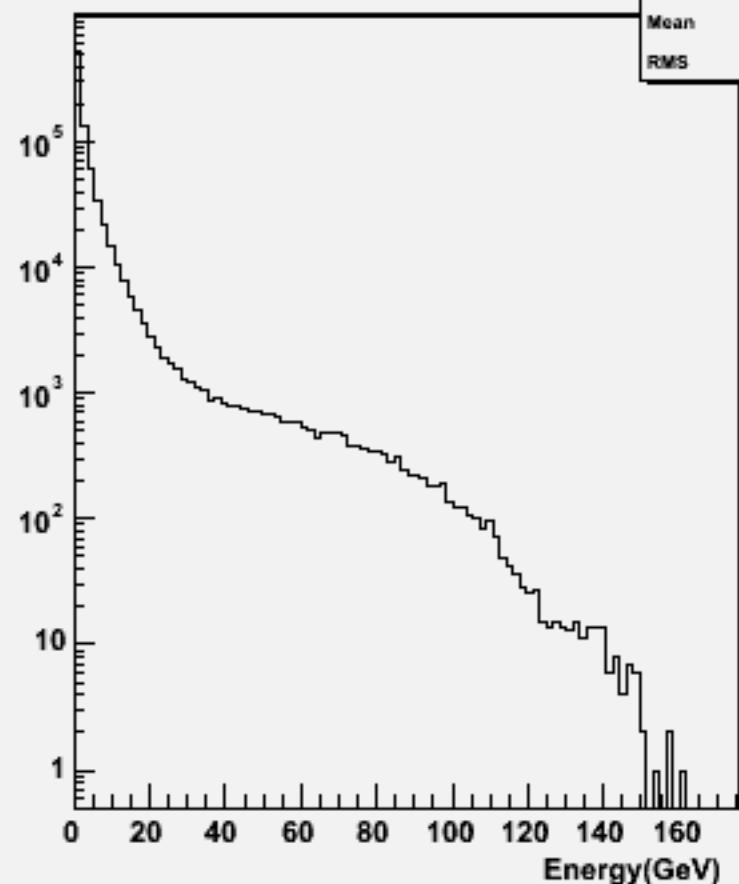
Particle Energy : w102312 n3n3dddd_o
