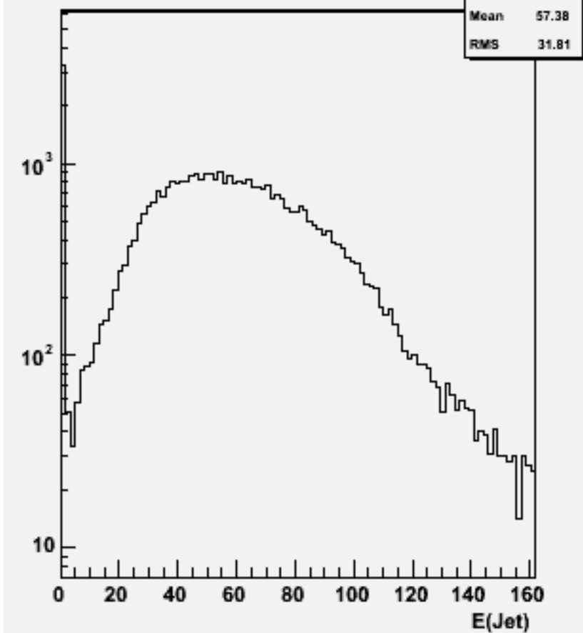
Jet energies(All jets)w102312 n3n3dddd_o
