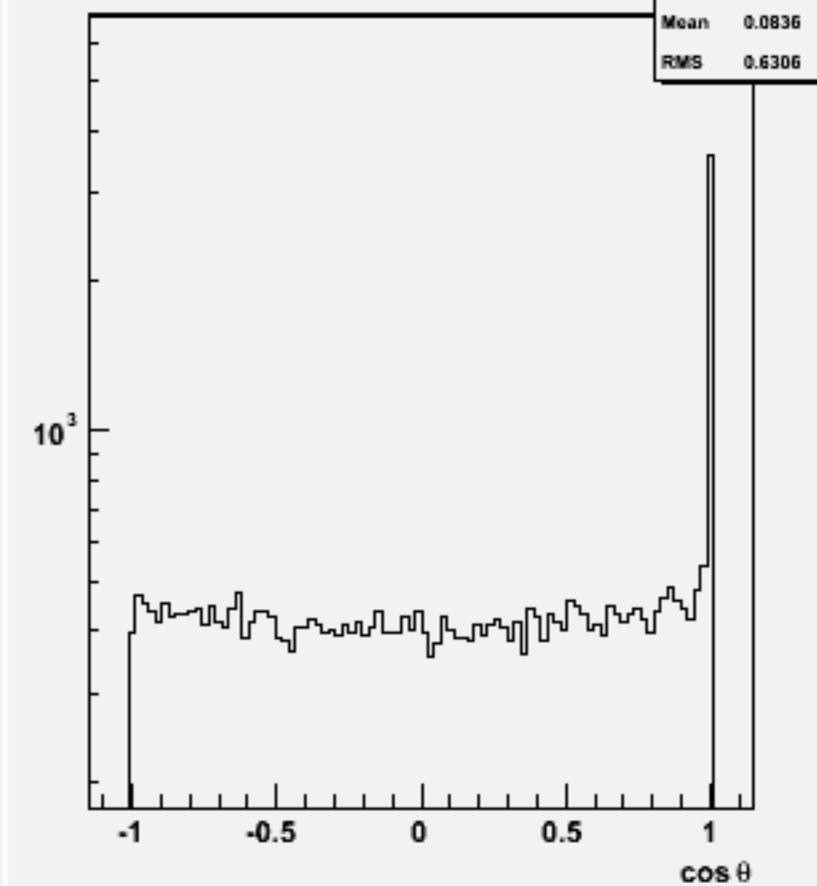
Jet cosθ (All jets)w102312 n3n3dddd_o
