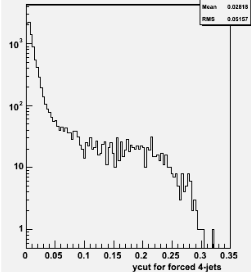
Ycut for 4-jets :w102312 n3n3dddd_o
