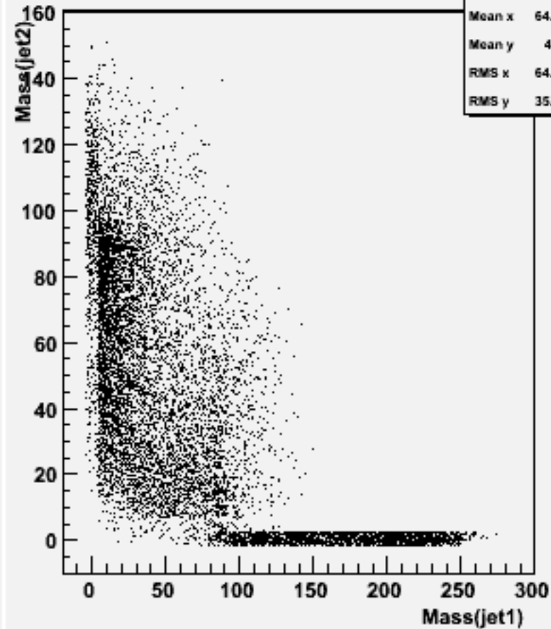
Jet mass for forced 2-jets : w102309 n3n3e2e2bb_o
