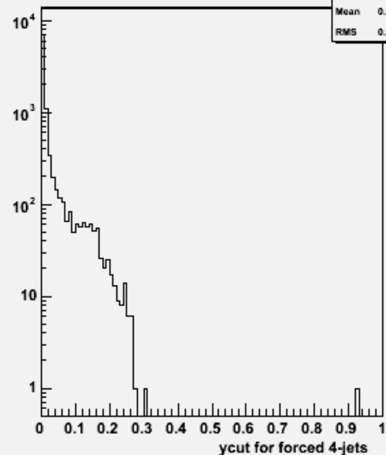
Ycut for 4-jets :w102309 n3n3e2e2bb_o
