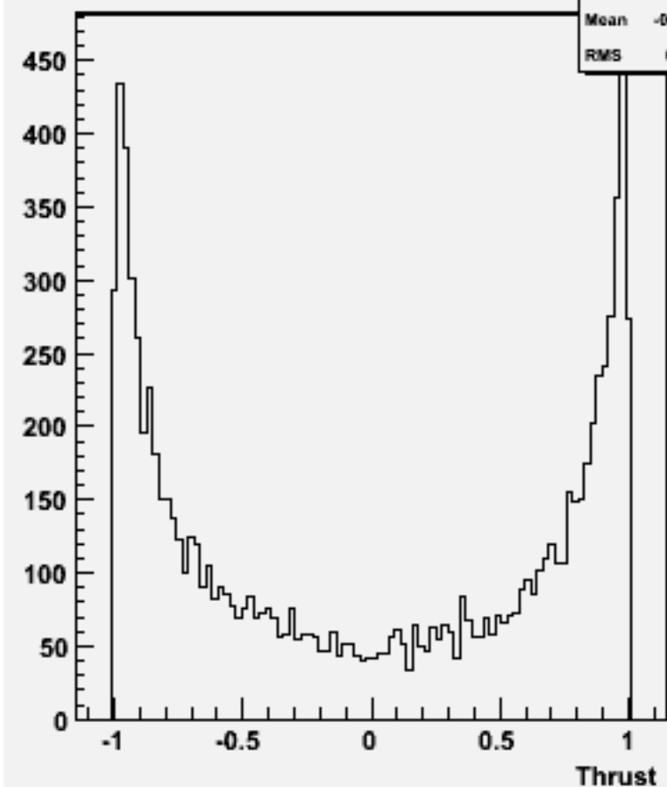
cos \Theta (thrust) w102309 n3n3e2e2bb_o
