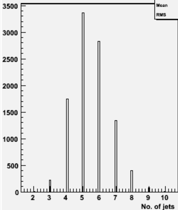
No. jets (ycut=0.001) : w102309 n3n3e2e2bb_o
