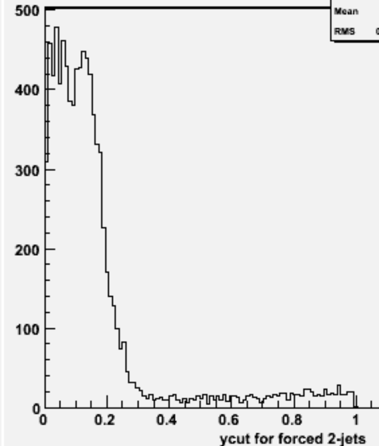
Ycut for 2-jets :w102309 n3n3e2e2bb_o
