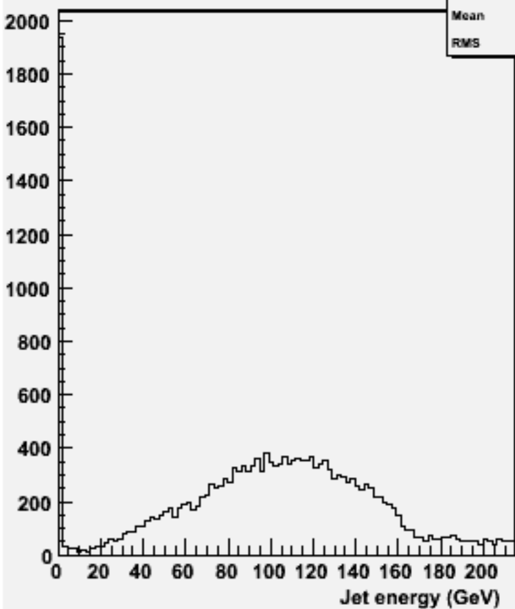
energy for 2-jets :w102309 n3n3e2e2bb_o
