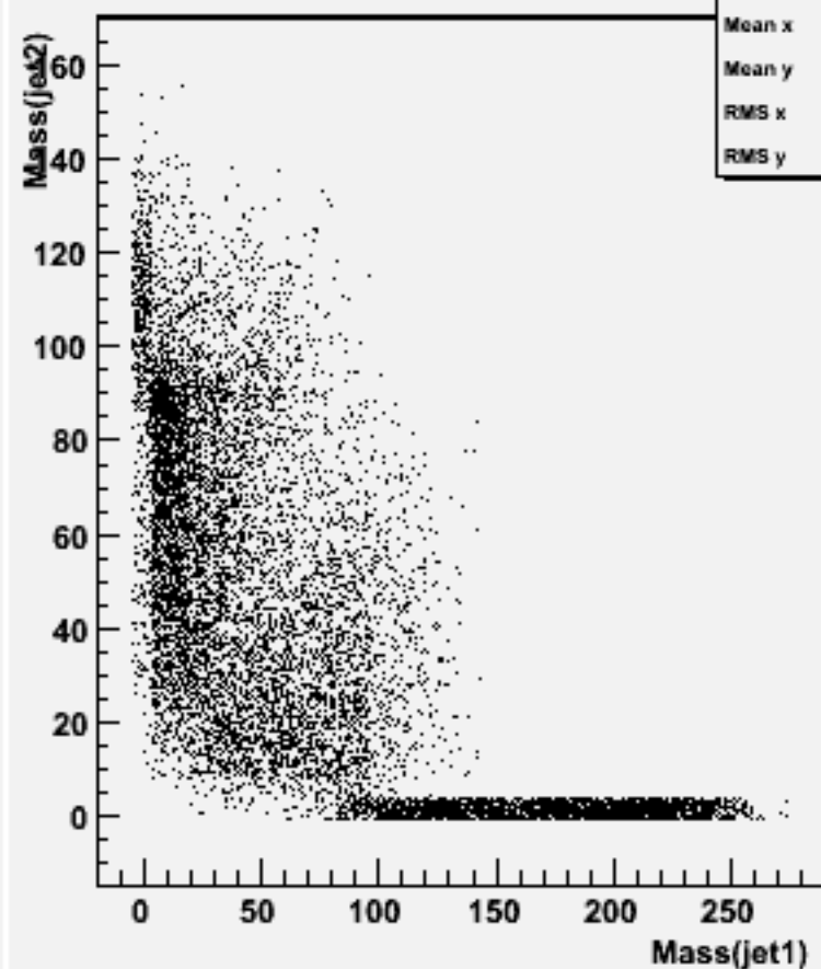
Jet mass for forced 2-jets : w102308 n3n3e2e2bb_o
