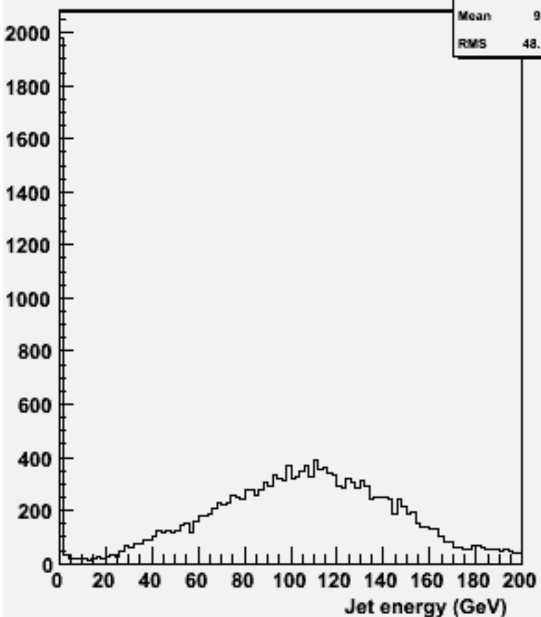
energy for 2-jets :w102308 n3n3e2e2bb_o
