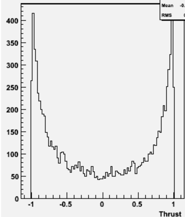
cos \Theta (thrust) w102308 n3n3e2e2bb_o
