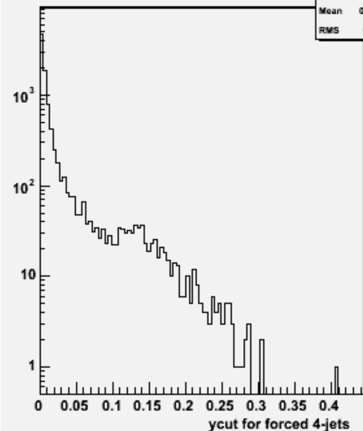
Ycut for 4-jets :w102308 n3n3e2e2bb_o
