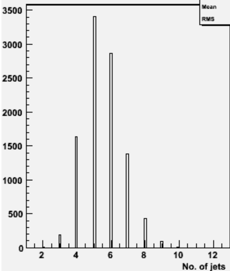
No. jets (ycut=0.001) : w102308 n3n3e2e2bb_o
