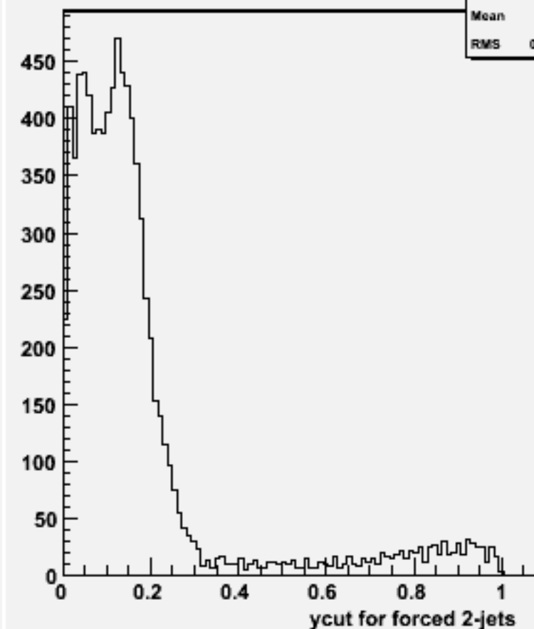
Ycut for 2-jets :w102308 n3n3e2e2bb_o
