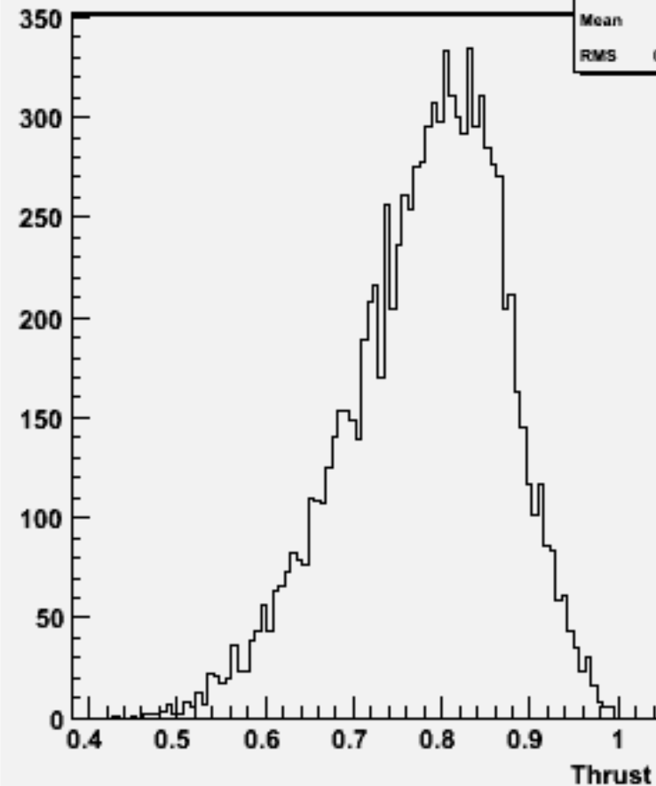
Thrust w102308 n3n3e2e2bb_o
