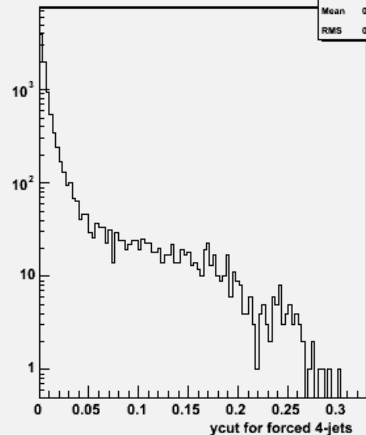
Ycut for 4-jets :w102304 n3n3e2e2ss_o
