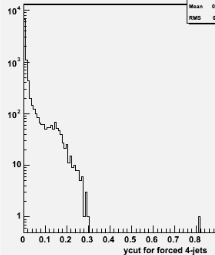
Ycut for 4-jets :w102301 n3n3e2e2dd_o
