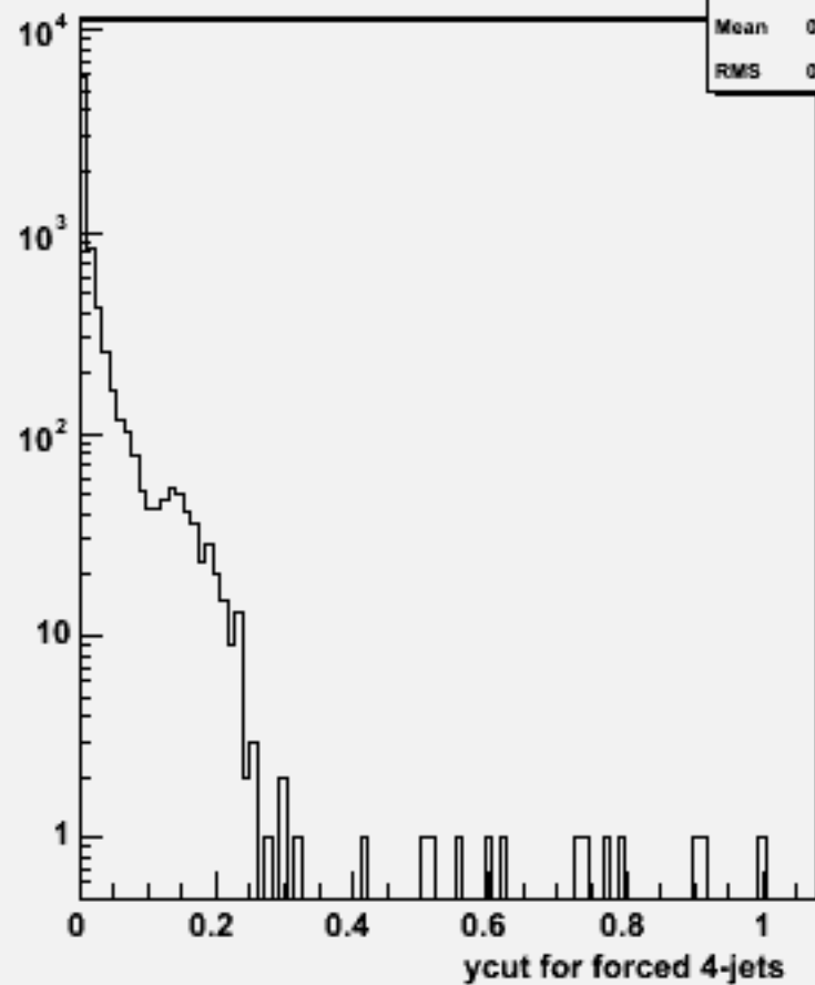
Ycut for 4-jets :w102296 n3n3e2e2e2e2_o
