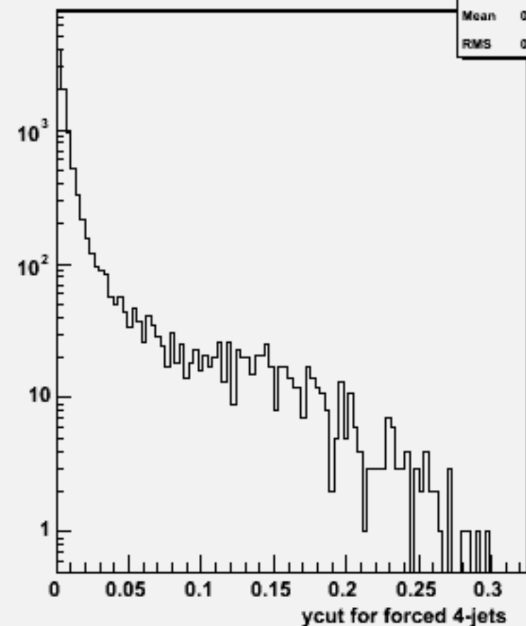
Ycut for 4-jets :w102293 n3n3e1e1bb_o
