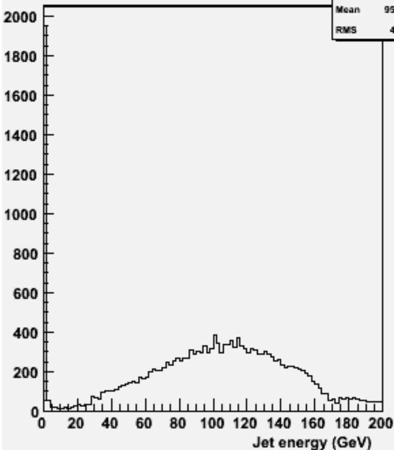
energy for 2-jets :w102293 n3n3e1e1bb_o
