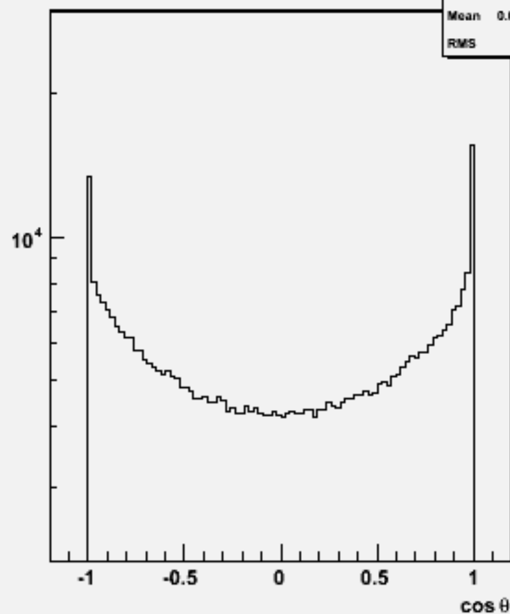
Particle cosθ : w102289 n3n3e1e1ss_o
