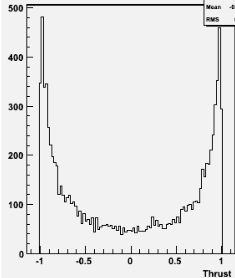
cos \Theta (thrust) w102289 n3n3e1e1ss_o
