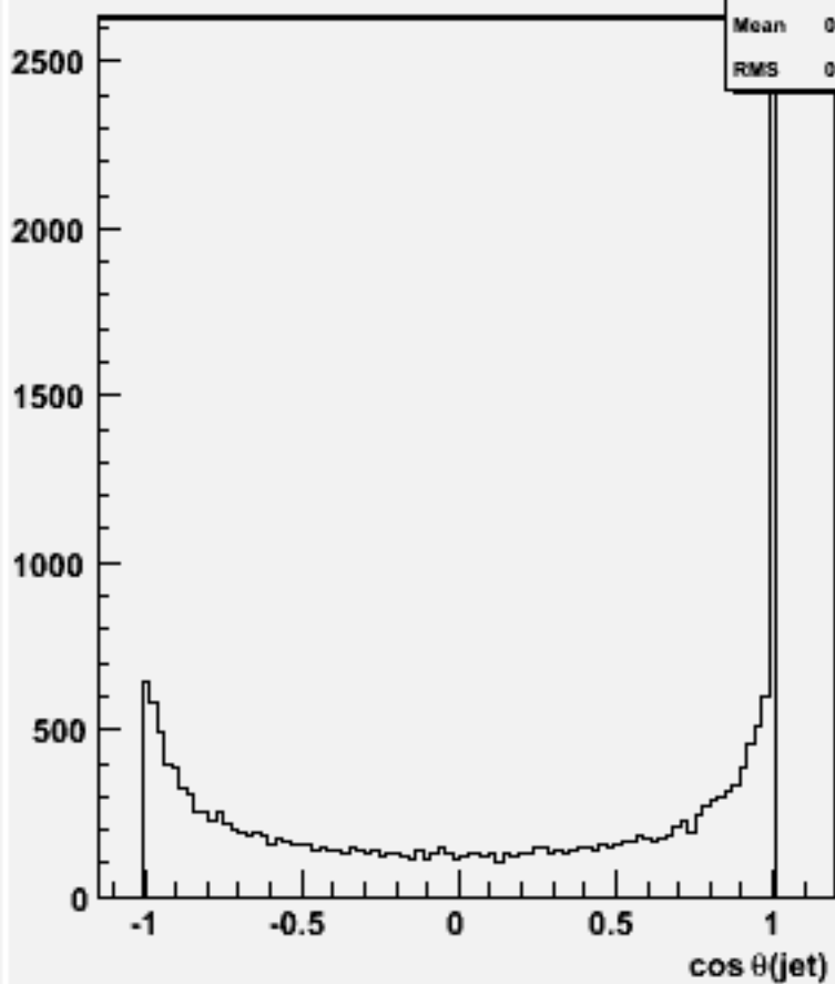
cos \theta for 2-jets :w102289 n3n3e1e1ss_o
