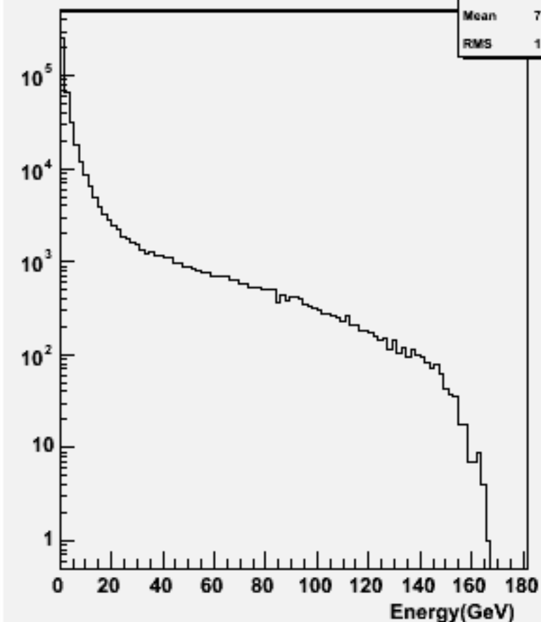
Particle Energy : w102289 n3n3e1e1ss_o
