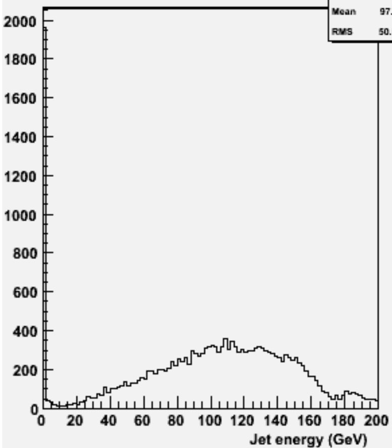
energy for 2-jets :w102289 n3n3e1e1ss_o
