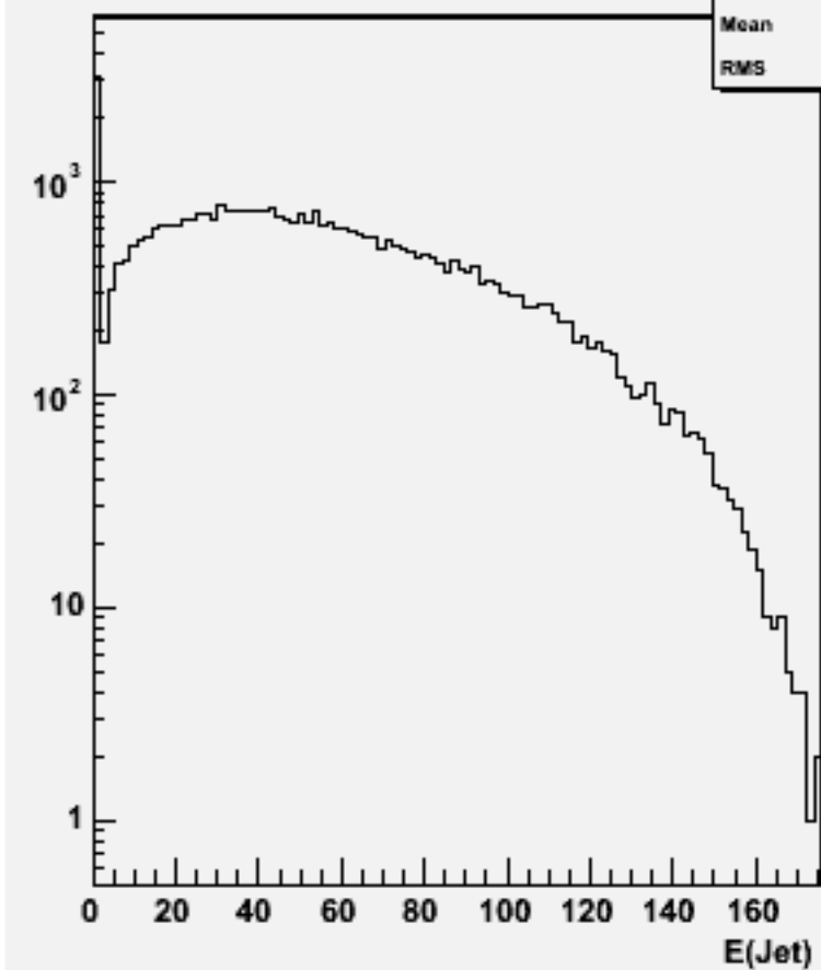
Jet energies(All jets)w102289 n3n3e1e1ss_o
