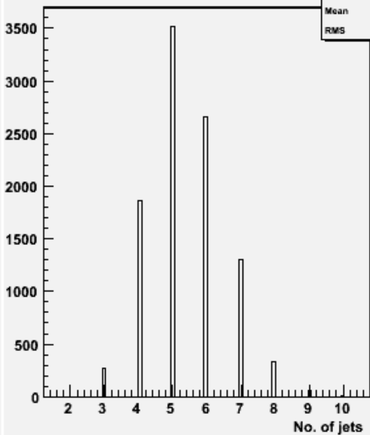
No. jets (ycut=0.001) : w102289 n3n3e1e1ss_o
