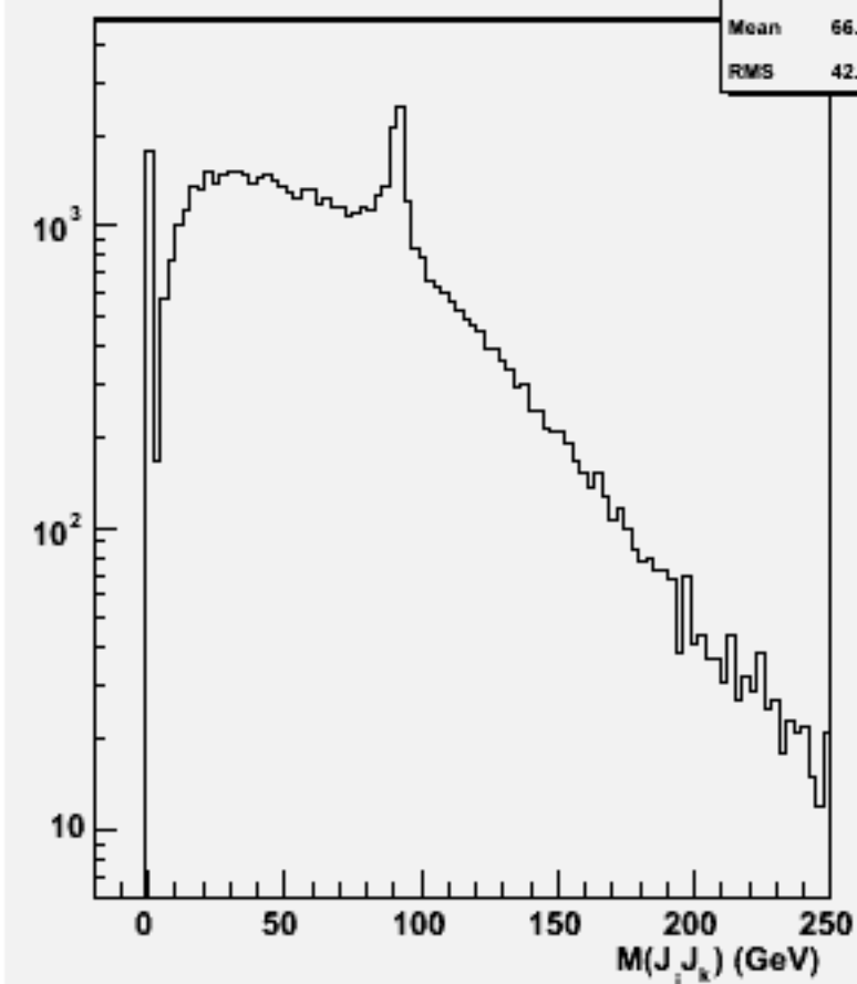
2jets mass(All comb)w102289 n3n3e1e1ss_o
