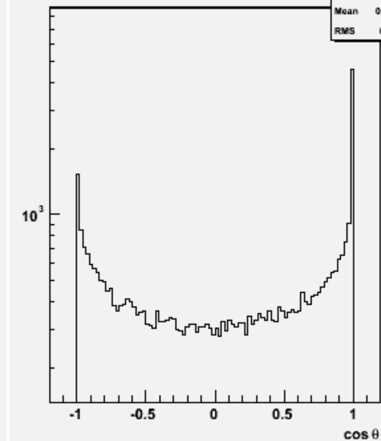
Jet cos \theta (All jets)w102289 n3n3e1e1ss_o
