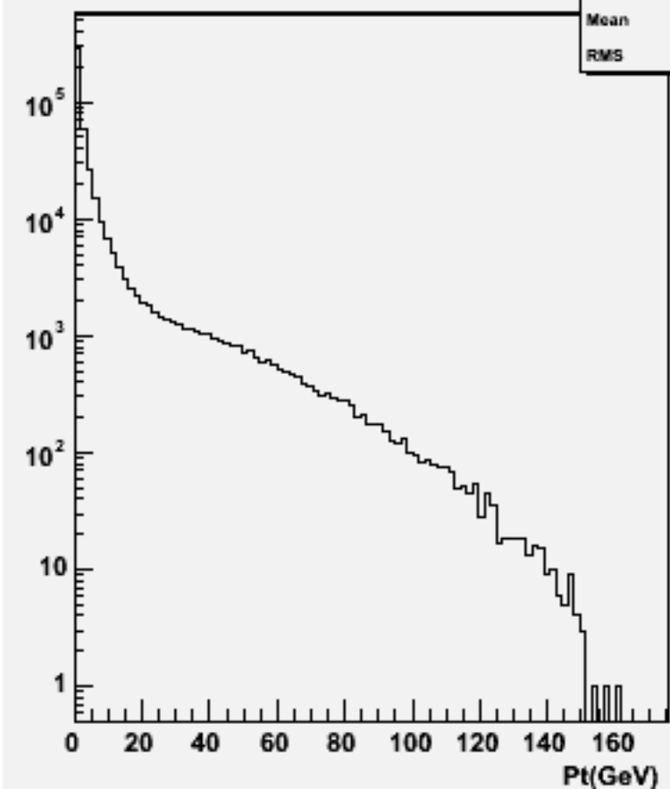
Particle Pt : w102289 n3n3e1e1ss_o
