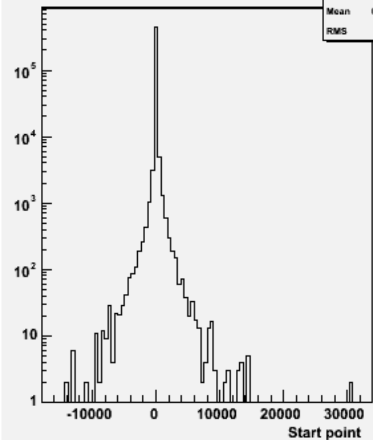
Start point Z : w102289 n3n3e1e1ss_o
