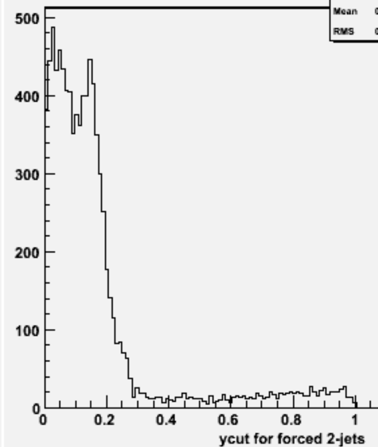
Ycut for 2-jets :w102289 n3n3e1e1ss_o
