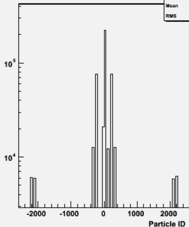
Particle ID : w102289 n3n3e1e1ss_o
