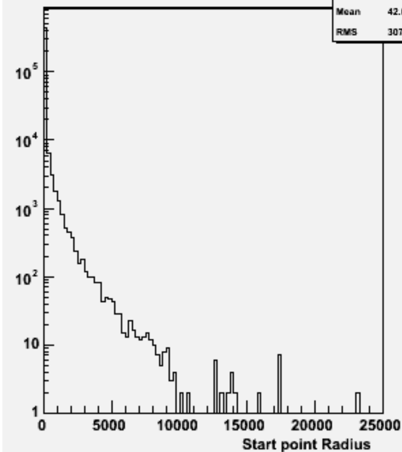
Start point R : w102289 n3n3e1e1ss_o
