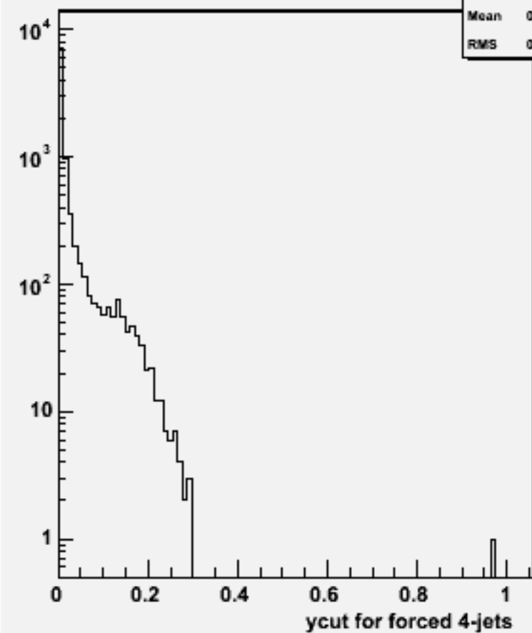
Ycut for 4-jets :w102289 n3n3e1e1ss_o
