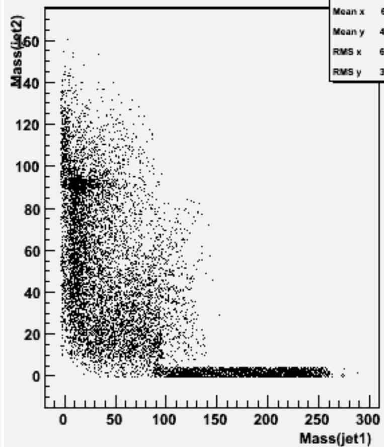
Jet mass for forced 2-jets : w102289 n3n3e1e1ss_o
