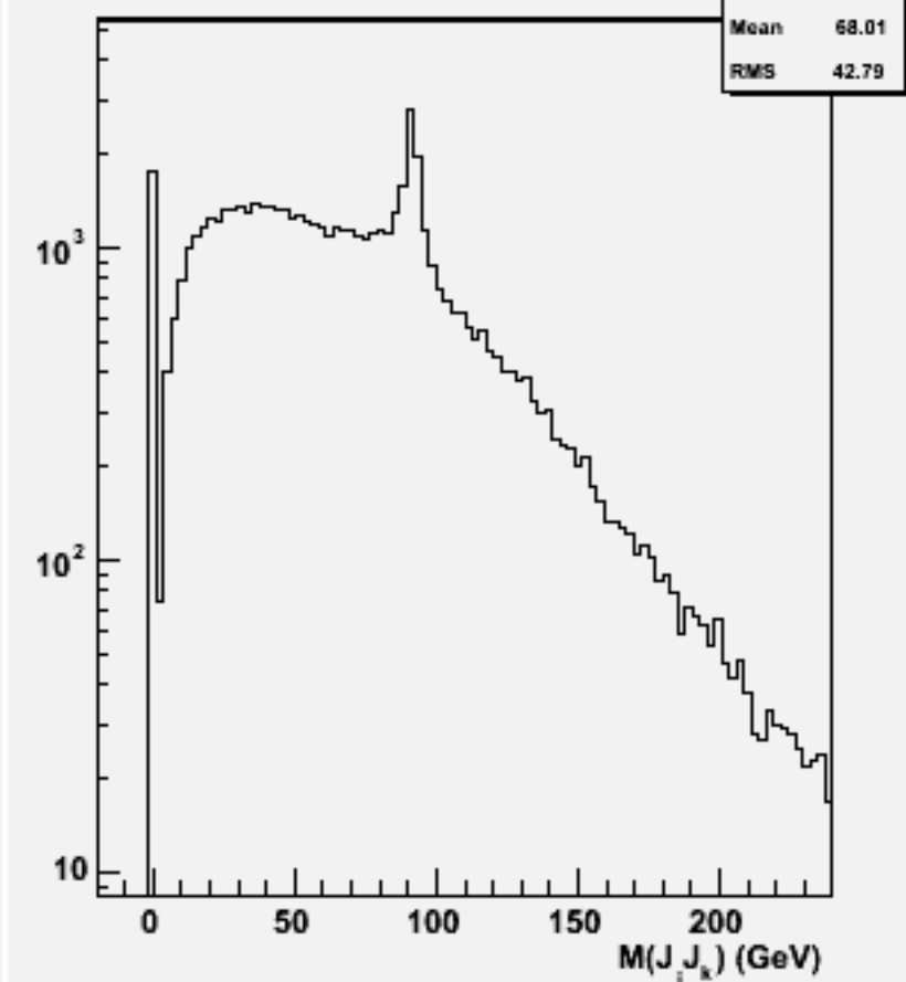
2jets mass(All comb)w102288 n3n3e1e1ss_o
