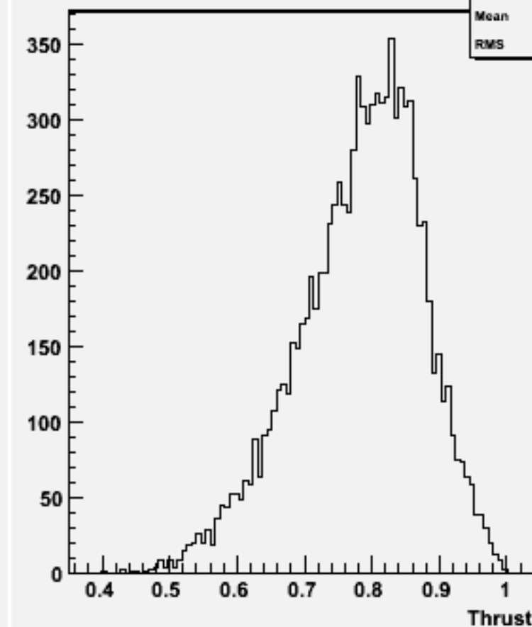
Thrust w102288 n3n3e1e1ss_o
