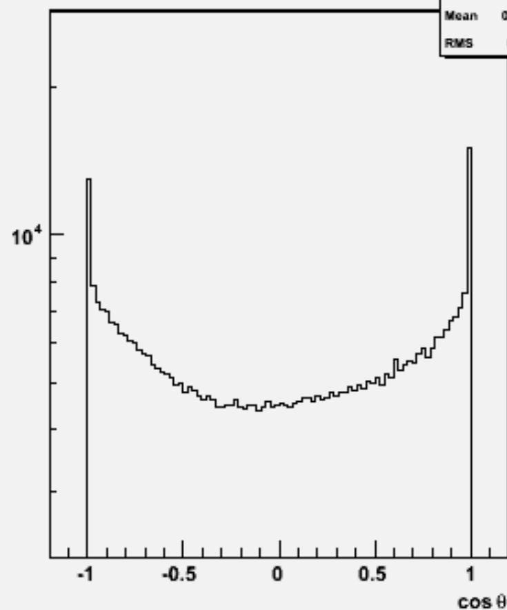
Particle cosθ : w102288 n3n3e1e1ss_o
