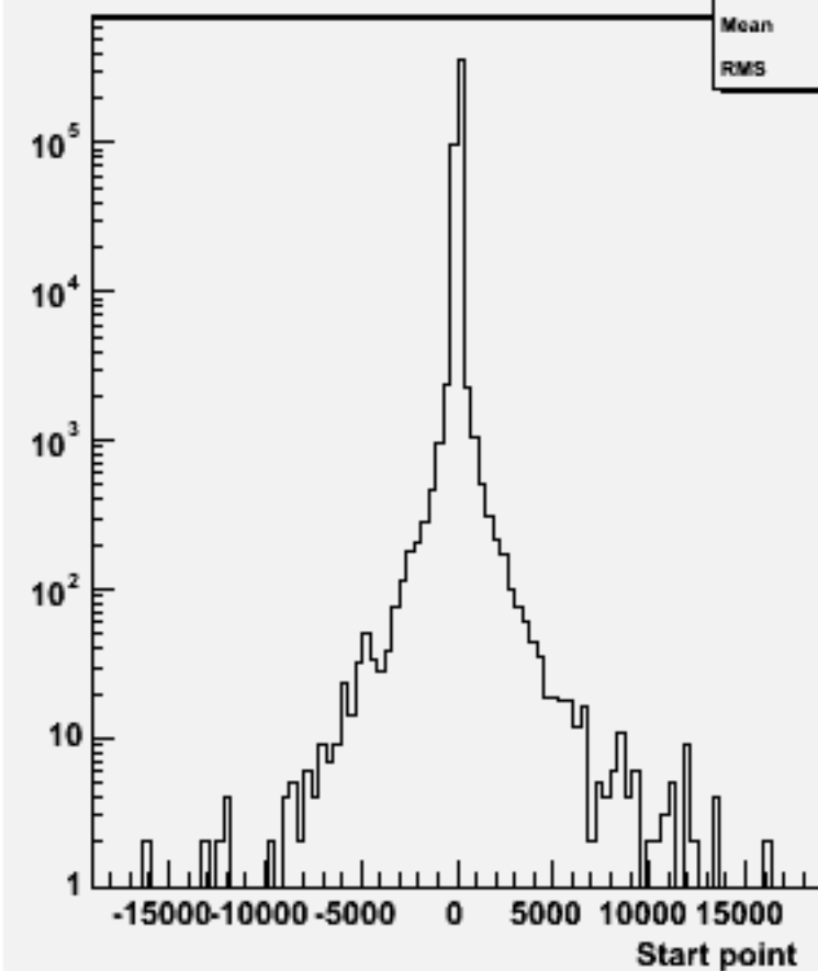
Start point Z : w102288 n3n3e1e1ss_o
