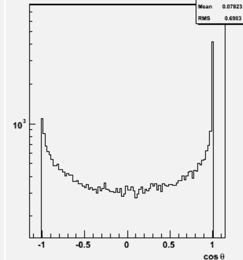
Jet cos \theta (All jets)w102288 n3n3e1e1ss_o
