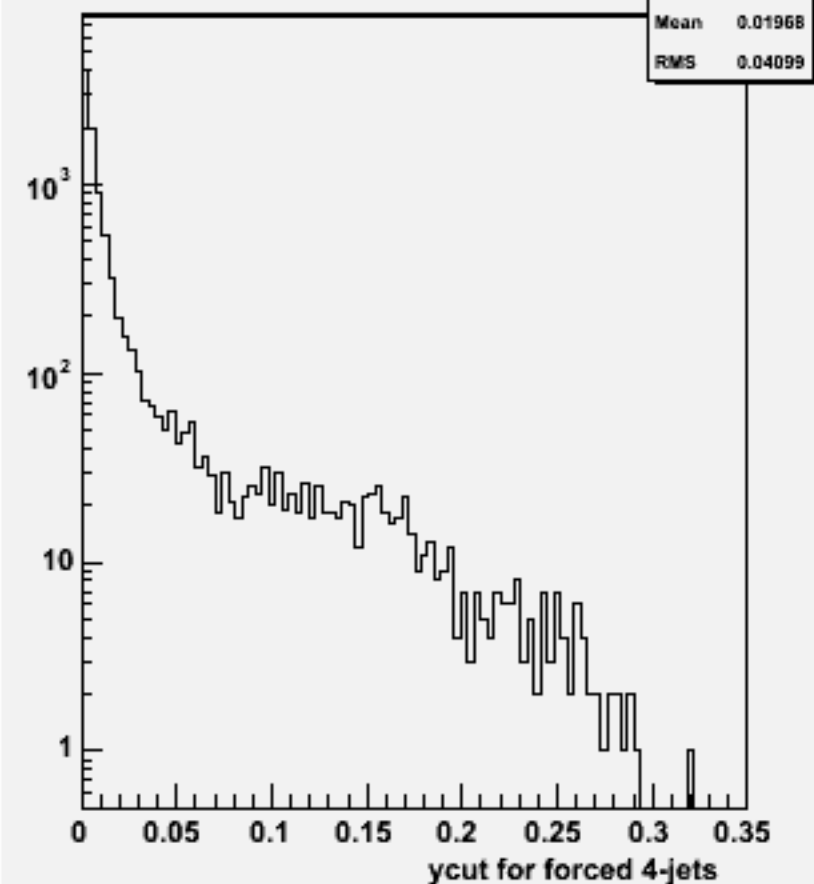
Ycut for 4-jets :w102288 n3n3e1e1ss_o
