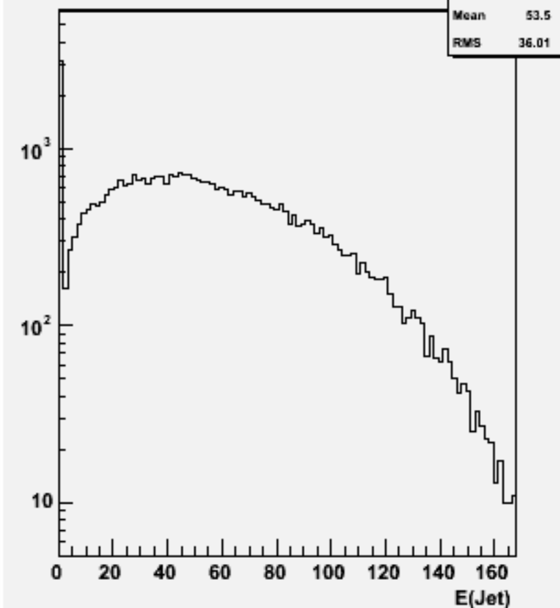
Jet energies(All jets)w102288 n3n3e1e1ss_o
