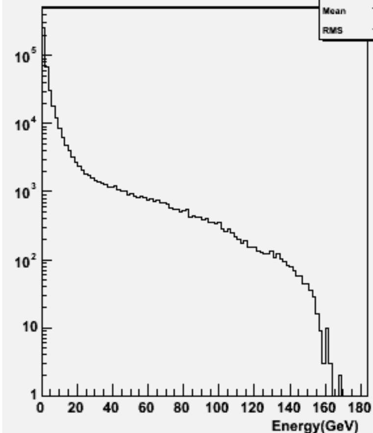
Particle Energy : w102288 n3n3e1e1ss_o
