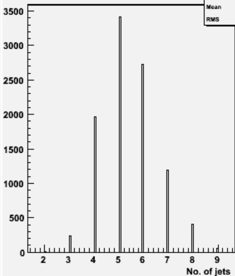
No. jets (ycut=0.001) : w102285 n3n3e1e1dd_o
