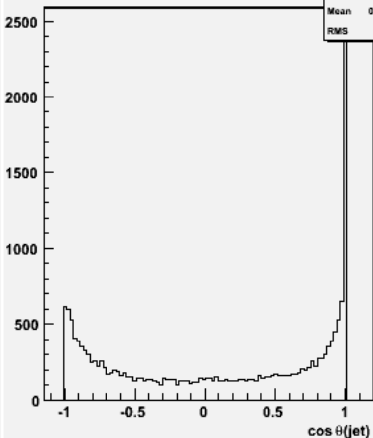
cos \theta for 2-jets :w102285 n3n3e1e1dd_o
