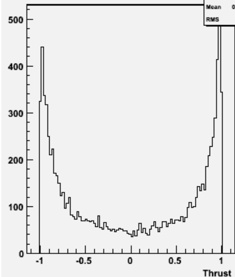
cos \Theta (thrust) w102285 n3n3e1e1dd_o
