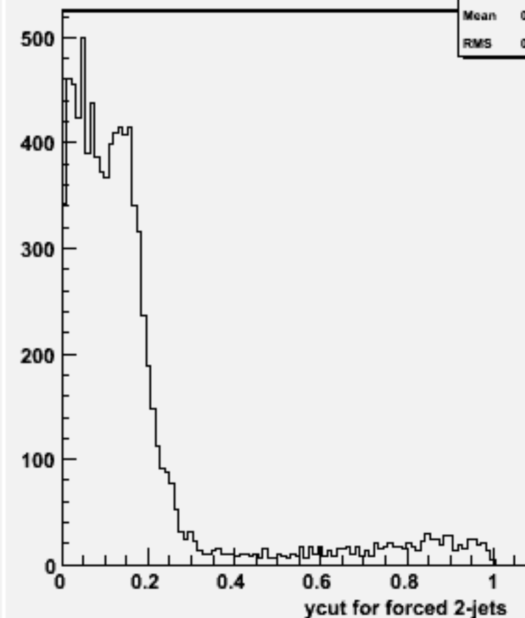
Ycut for 2-jets :w102285 n3n3e1e1dd_o
