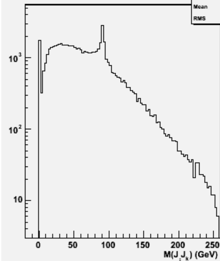
2jets mass(All comb)w102285 n3n3e1e1dd_o
