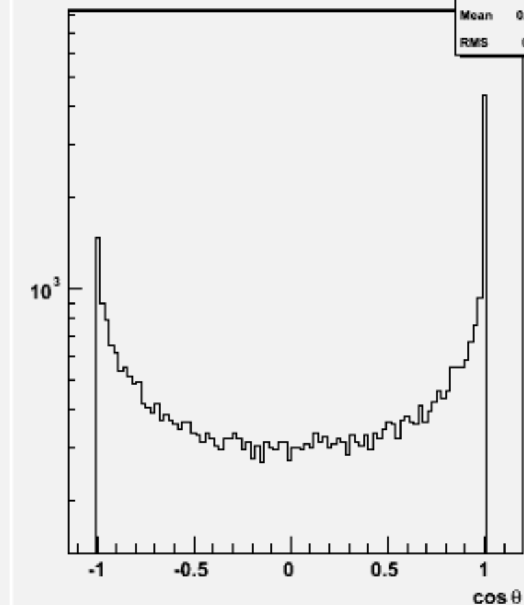
Jet cos \theta (All jets)w102285 n3n3e1e1dd_o
