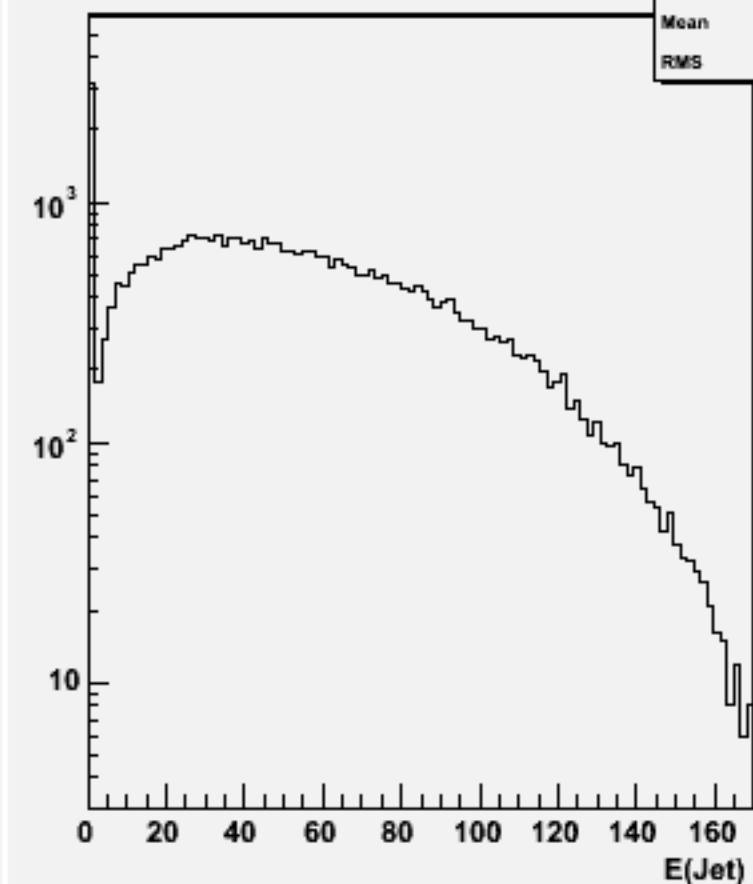
Jet energies(All jets)w102285 n3n3e1e1dd_o
