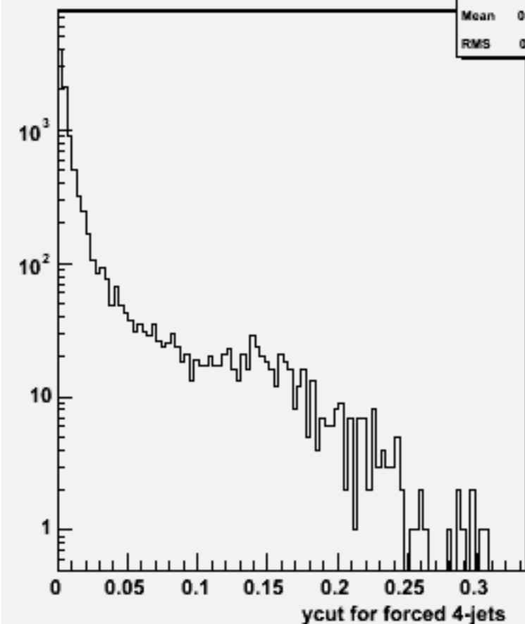
Ycut for 4-jets :w102285 n3n3e1e1dd_o
