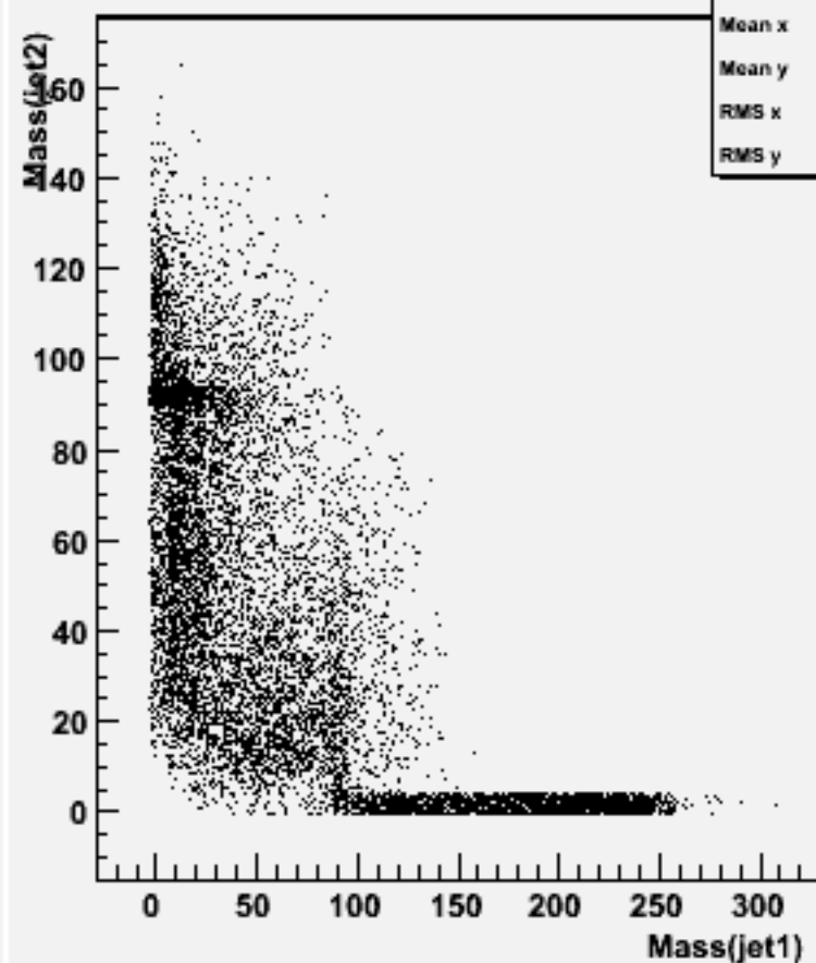
Jet mass for forced 2-jets : w102285 n3n3e1e1dd_o
