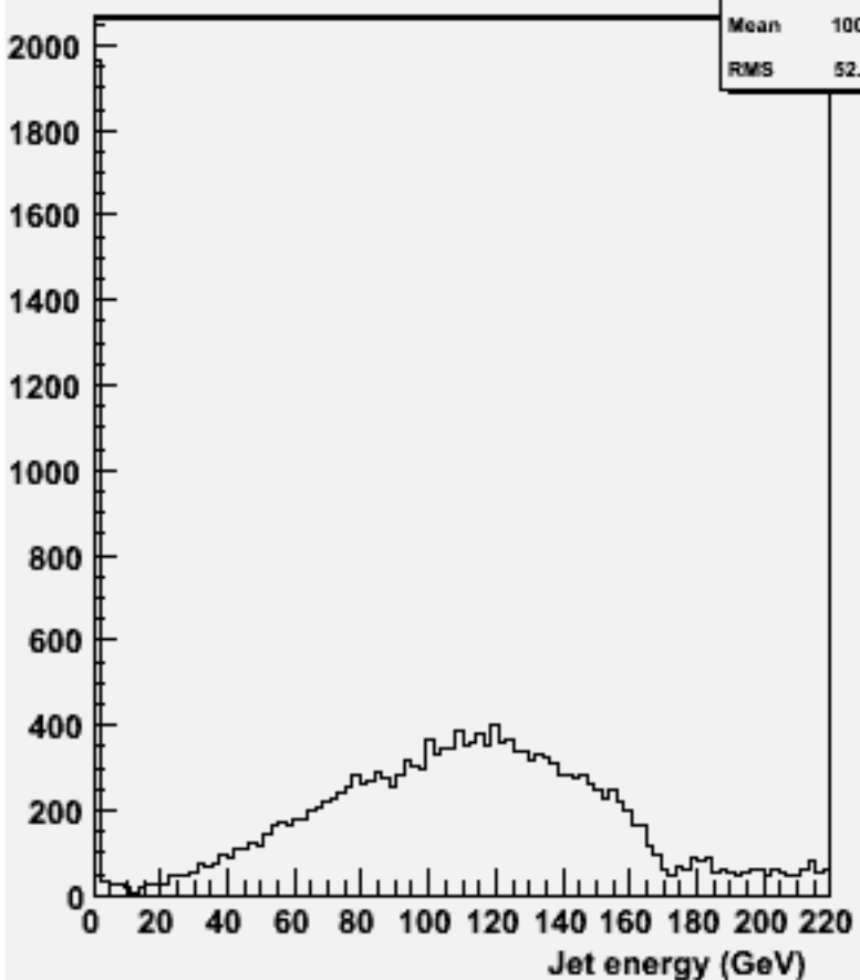
energy for 2-jets :w102285 n3n3e1e1dd_o
