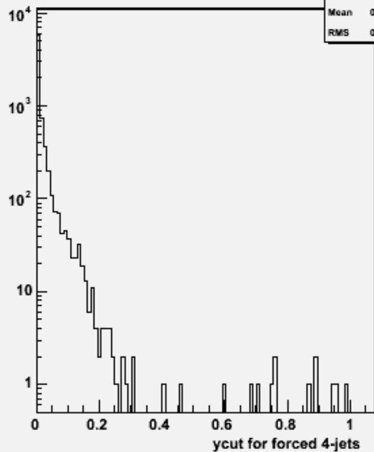
Ycut for 4-jets :w102282 n3n3e1e1e2e2_o
