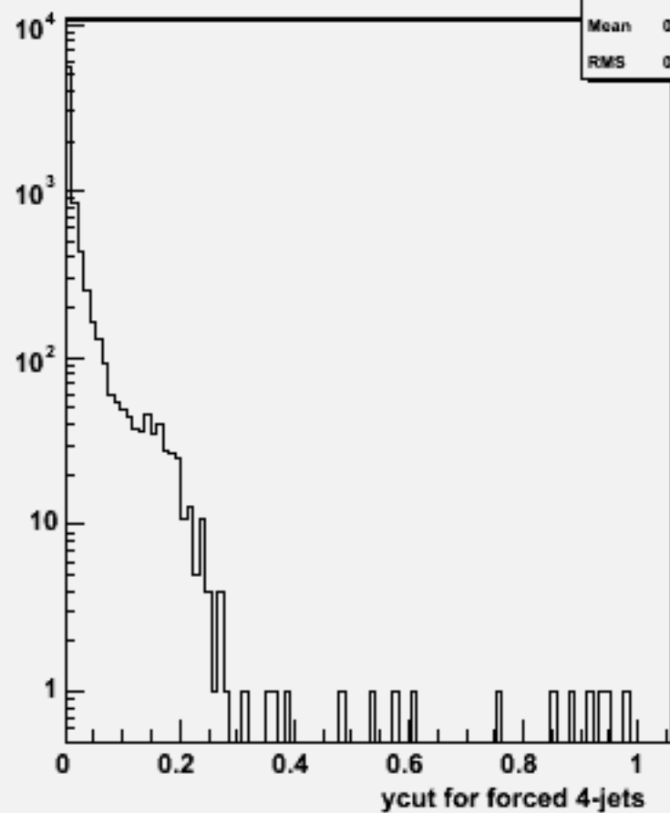
Ycut for 4-jets :w102280 n3n3e1e1e2e2_o
