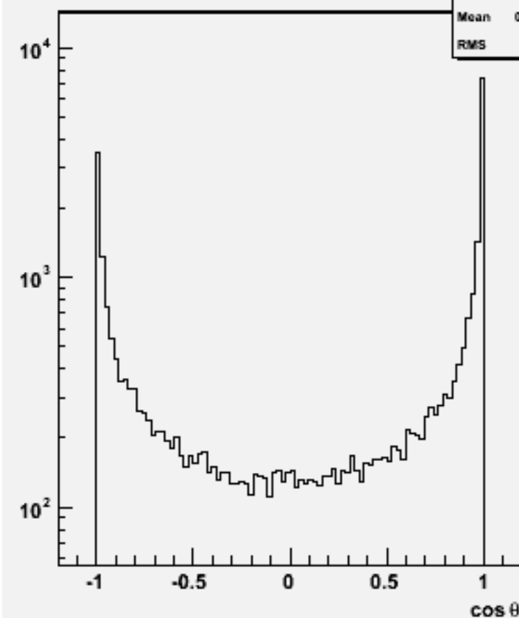
Jet cos \theta (All jets)w102278 n3n3e1e1e1e1_o
