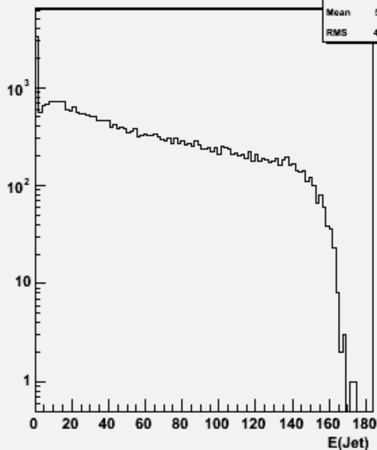
Jet energies(All jets)w102278 n3n3e1e1e1e1_o
