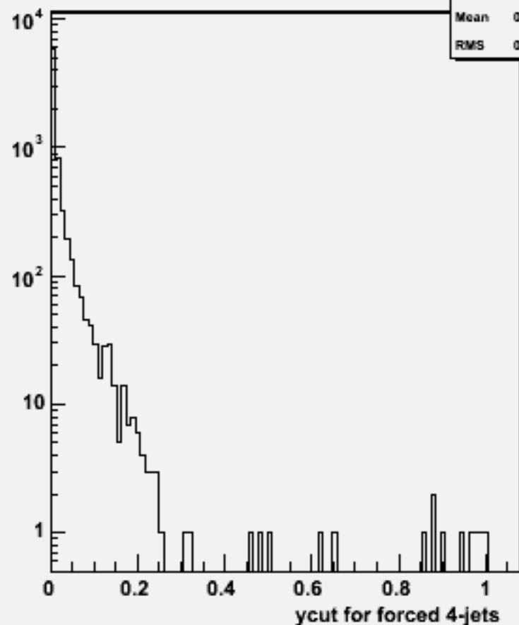
Ycut for 4-jets :w102278 n3n3e1e1e1e1_o
