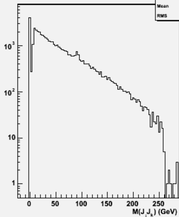
2jets mass(All comb)w102278 n3n3e1e1e1e1_o
