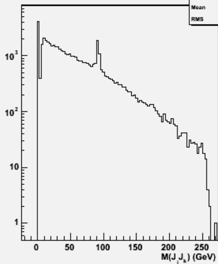
2jets mass(All comb)w102277 n3n3e1e1e1e1_o
