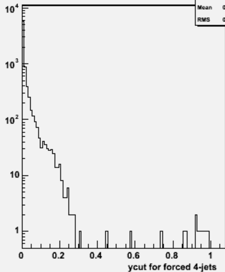
Ycut for 4-jets :w102277 n3n3e1e1e1e1_o
