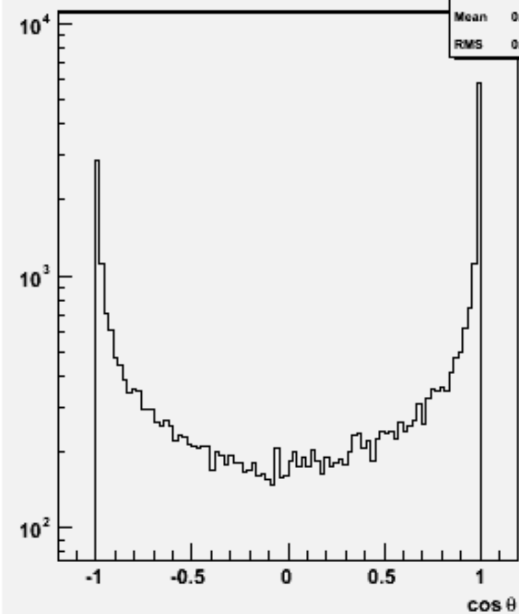
Jet cos \theta (All jets)w102277 n3n3e1e1e1e1_o
