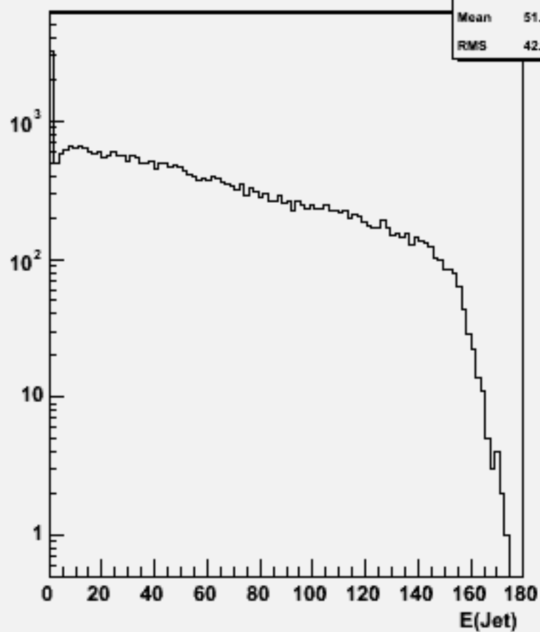
Jet energies(All jets)w102277 n3n3e1e1e1e1_o
