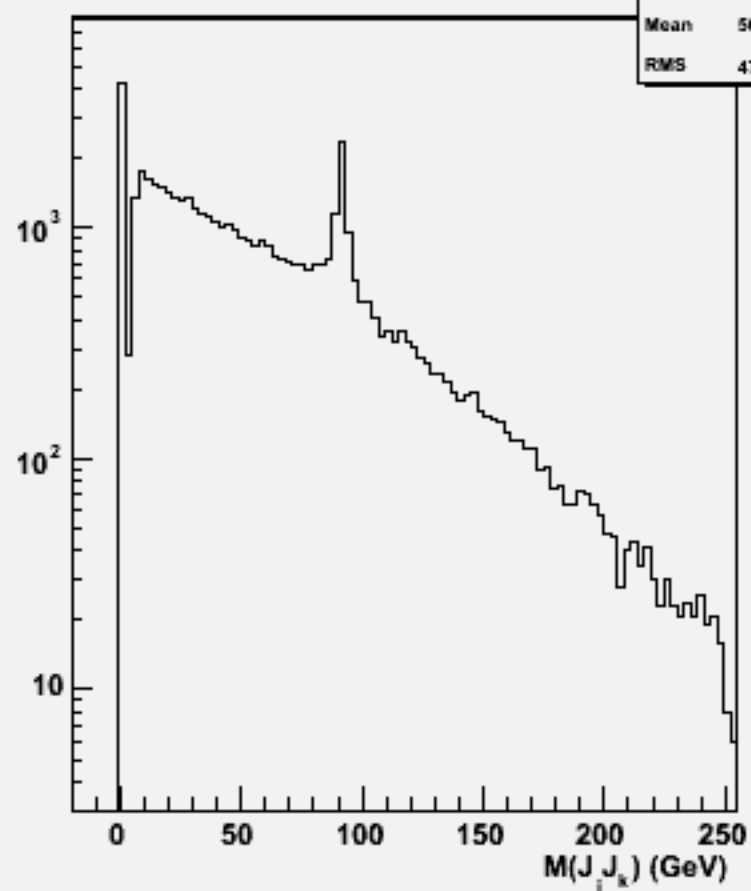
2jets mass(All comb)w102276 n3n3e1e1e1e1_o
