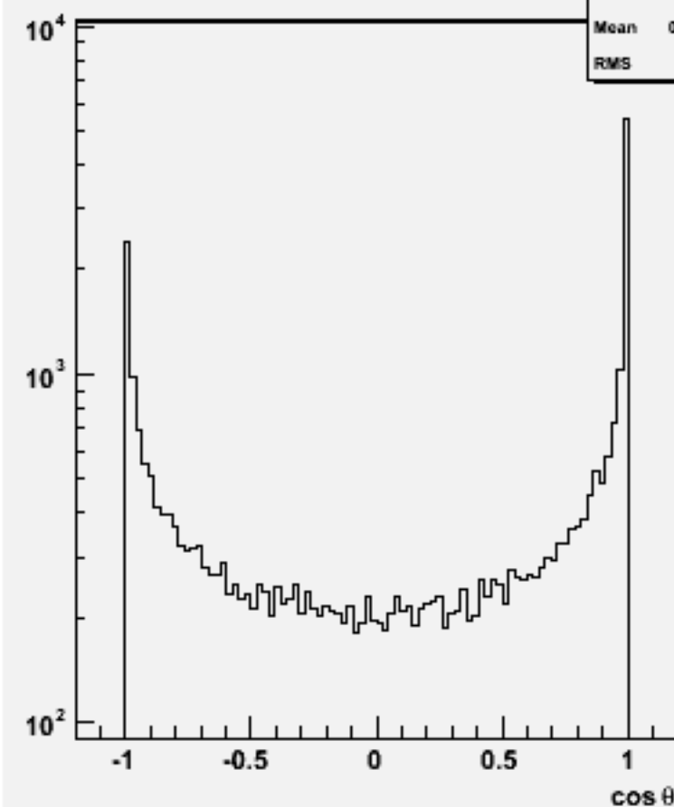
Jet cos \theta (All jets)w102276 n3n3e1e1e1e1_o
