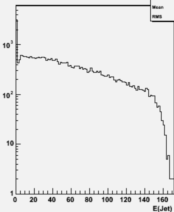
Jet energies(All jets)w102276 n3n3e1e1e1e1_o
