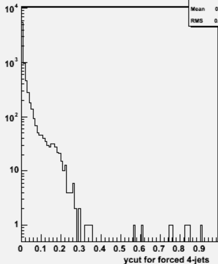
Ycut for 4-jets :w102276 n3n3e1e1e1e1_o
