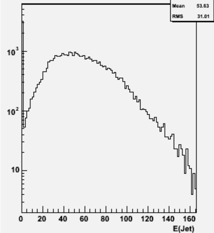
Jet energies(All jets)w102273 n2n2bbbb_o
