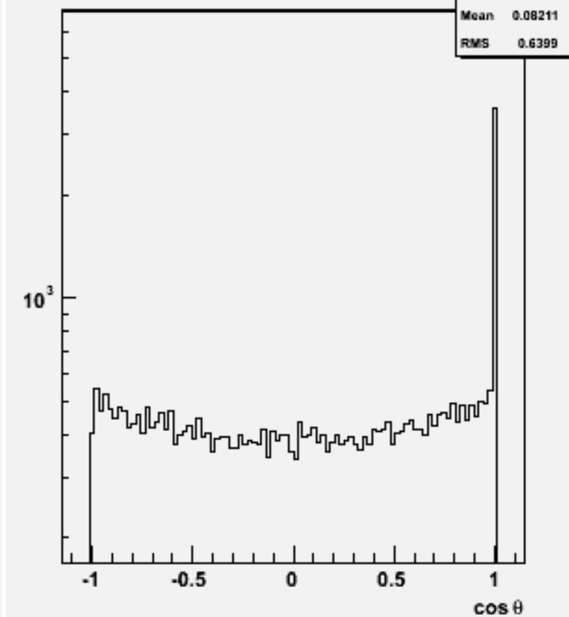
Jet cos \theta (All jets)w102273 n2n2bbbb_o
