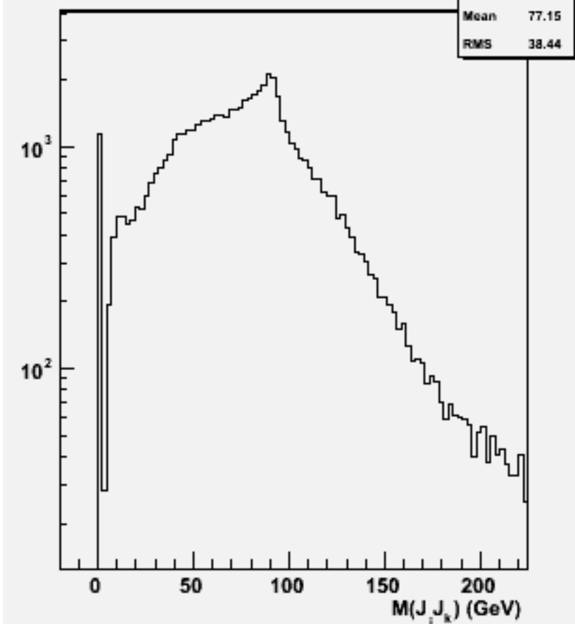
2jets mass(All comb)w102273 n2n2bbbb_o
