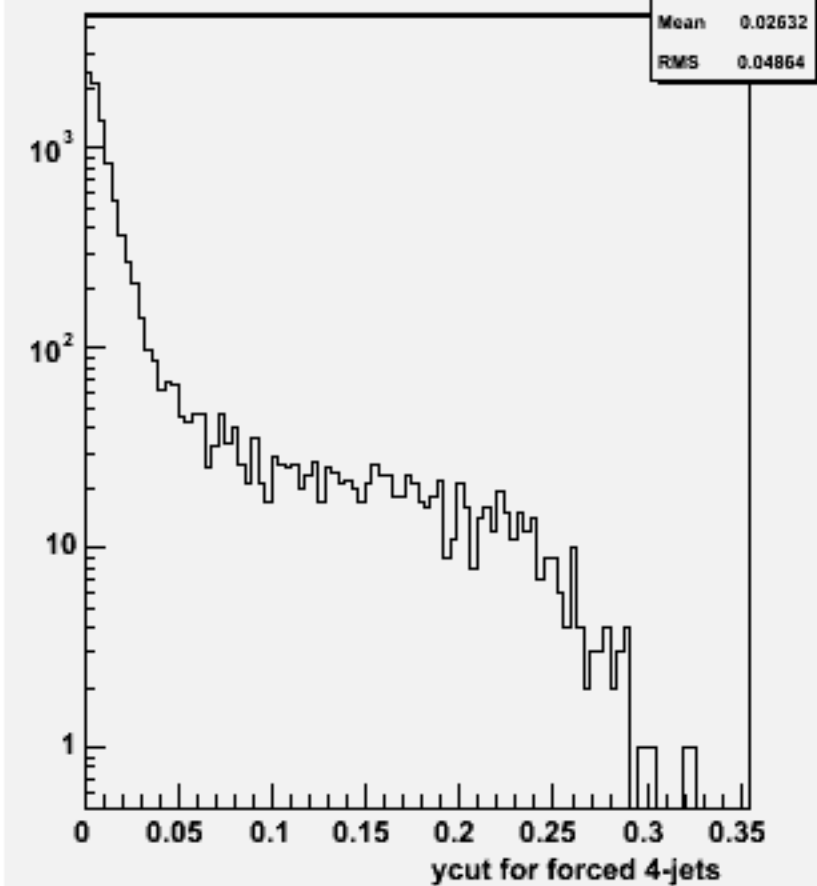
Ycut for 4-jets :w102273 n2n2bbbb_o
