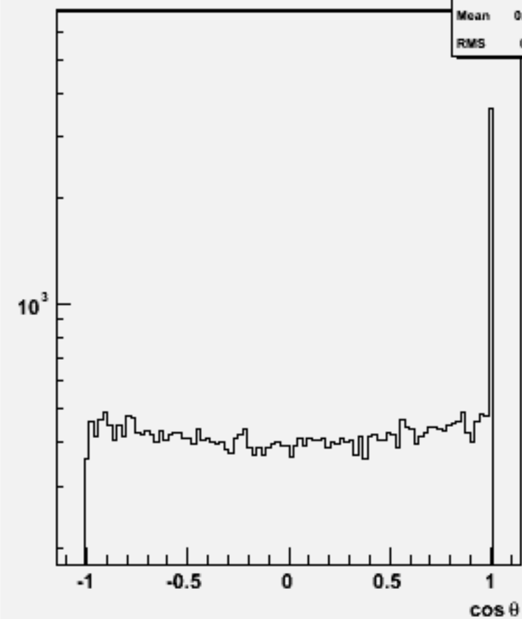
Jet cos \theta (All jets)w102272 n2n2bbbb_o
