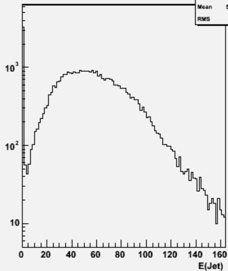
Jet energies(All jets)w102272 n2n2bbbb_o
