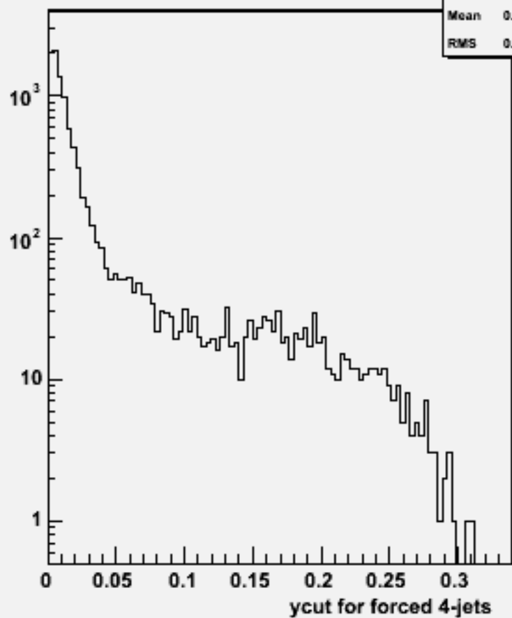
Ycut for 4-jets :w102272 n2n2bbbb_o
