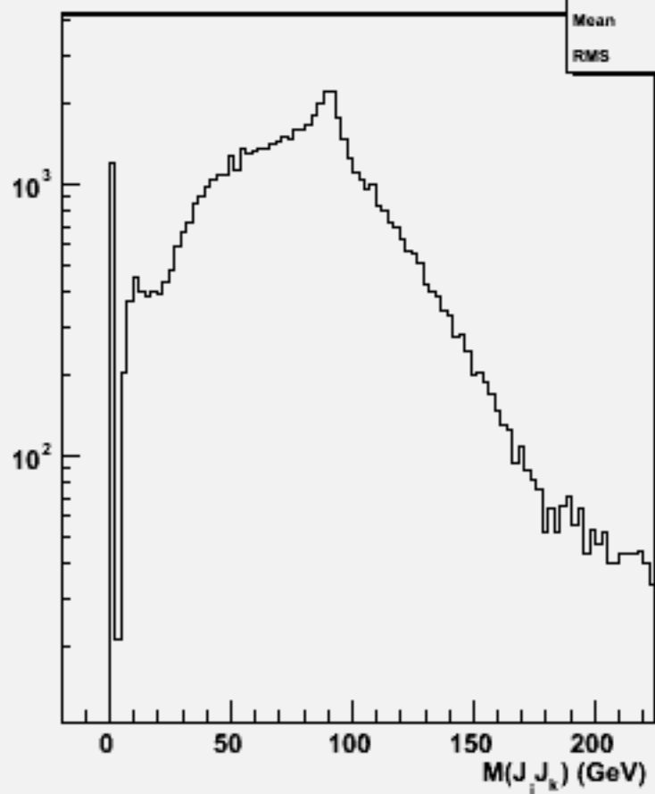
2jets mass(All comb)w102272 n2n2bbbb_o
