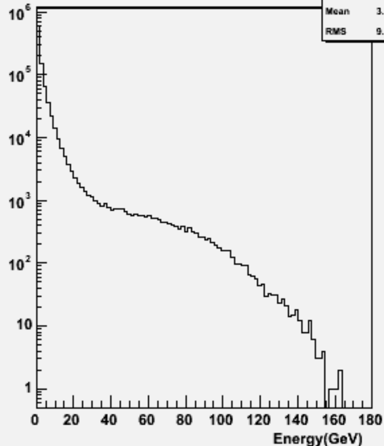
Particle Energy : w102269 n2n2ssbb_o
