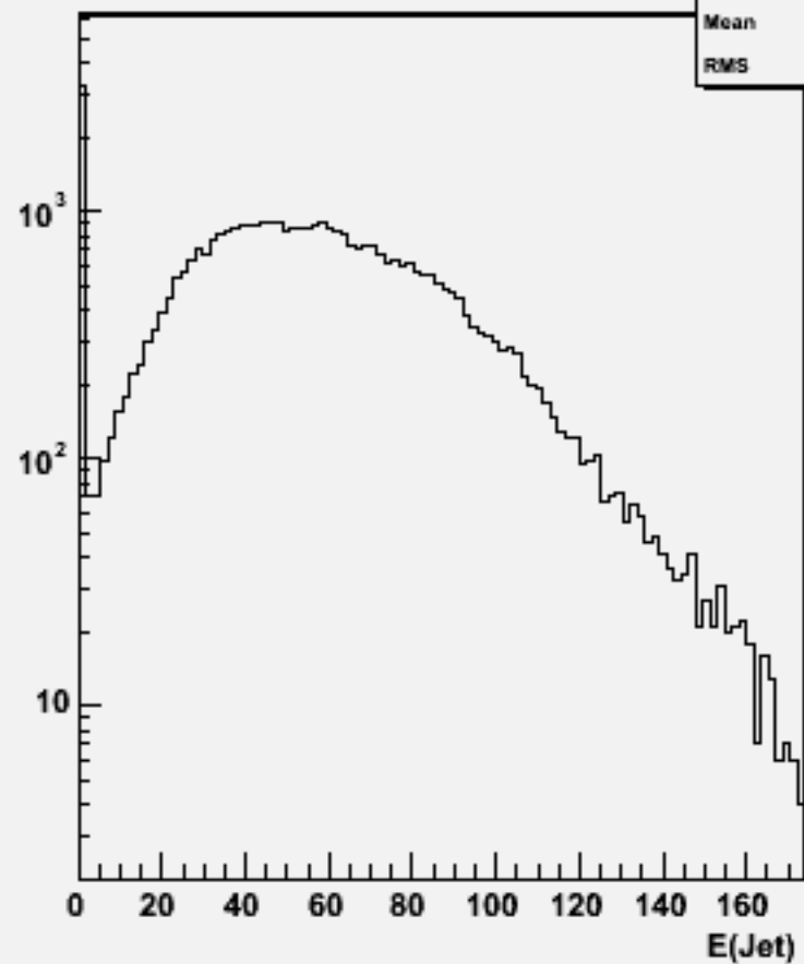
Jet energies(All jets)w102269 n2n2ssbb_o
