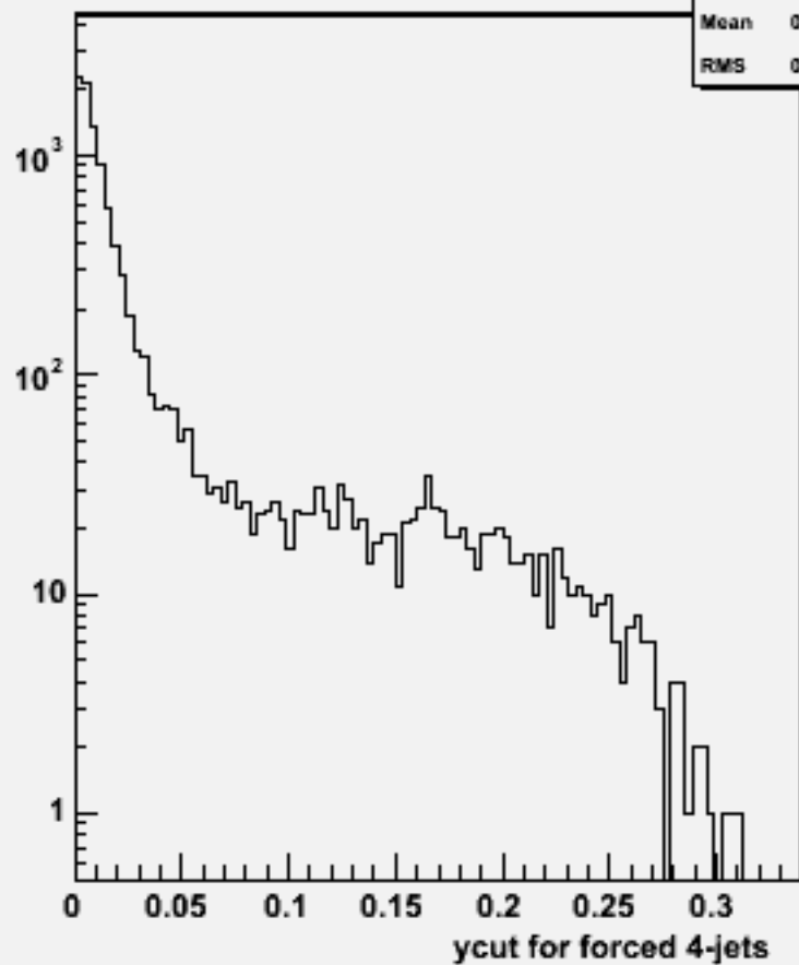
Ycut for 4-jets :w102269 n2n2ssbb_o
