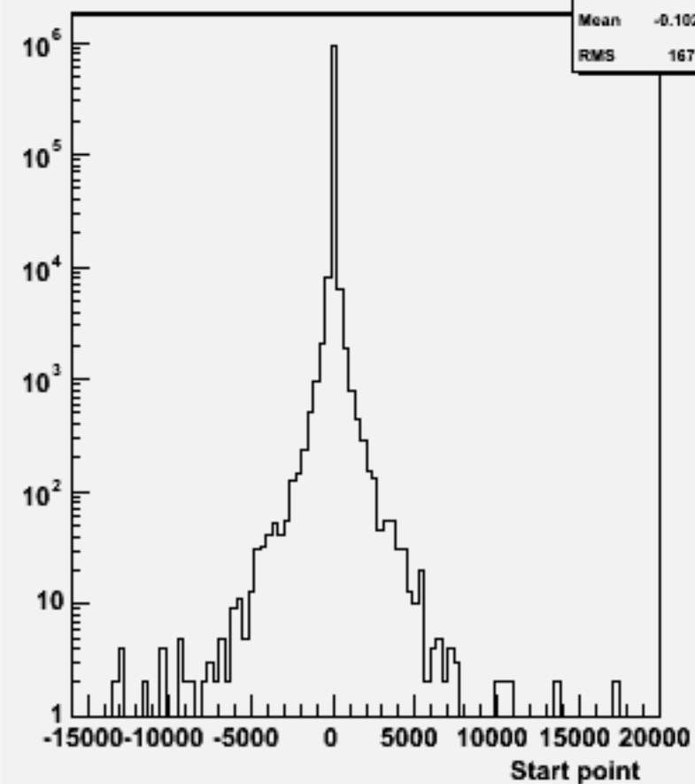
Start point Z : w102269 n2n2ssbb_o
