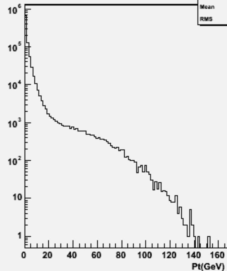
Particle Pt : w102269 n2n2ssbb_o
