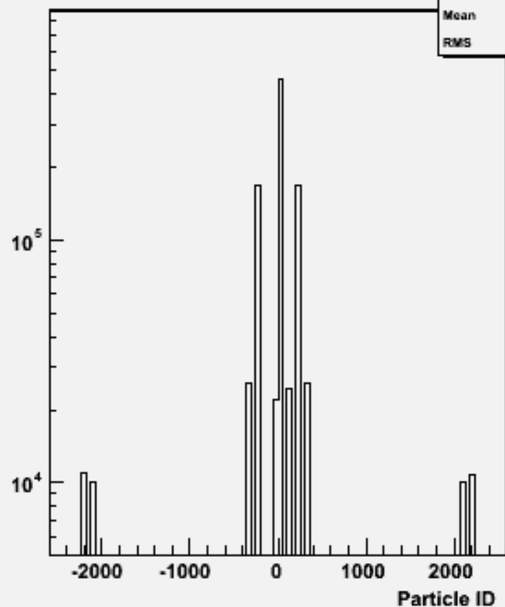
Particle ID : w102269 n2n2ssbb_o
