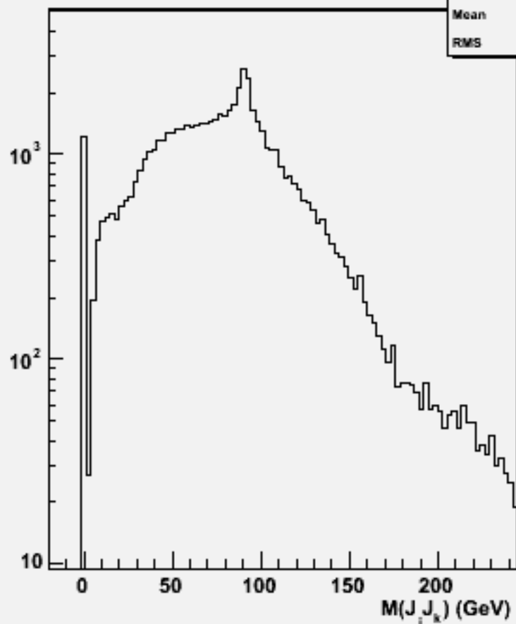
2jets mass(All comb)w102269 n2n2ssbb_o
