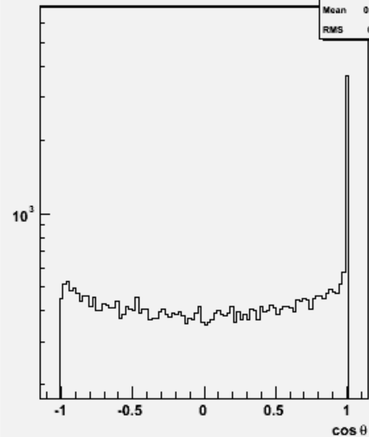
Jet cosθ (All jets)w102269 n2n2ssbb_o
