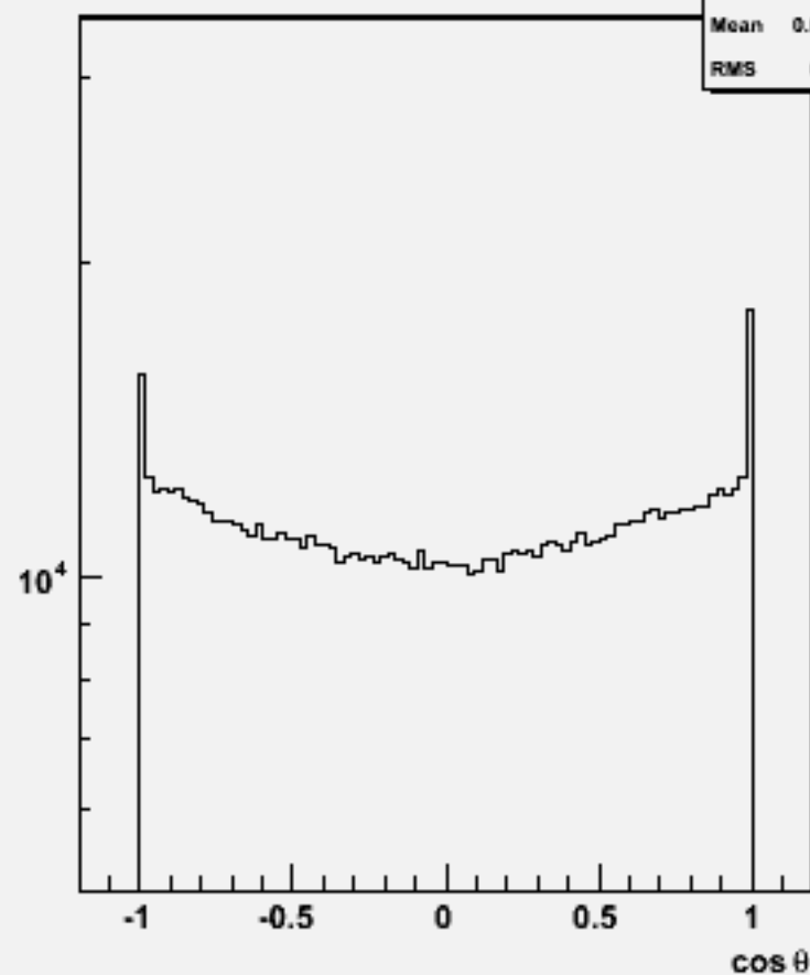
Particle cos \theta : w102269 n2n2ssbb_o
