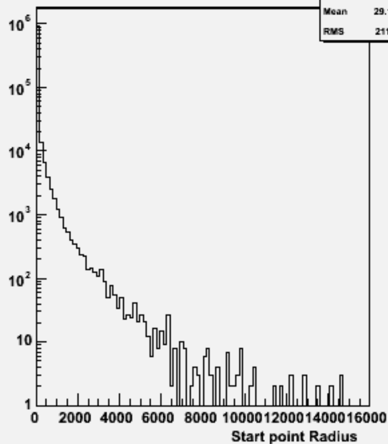
Start point R : w102269 n2n2ssbb_o
