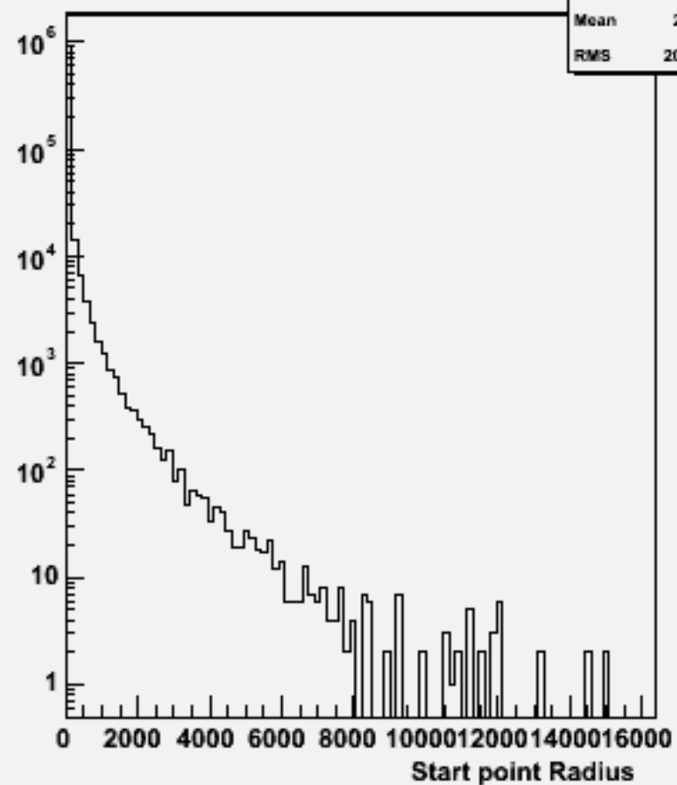
Start point R : w102268 n2n2ssbb_o
