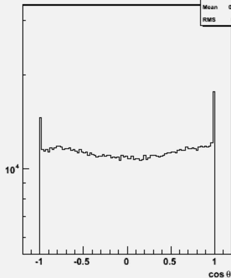
Particle cos \theta : w102268 n2n2ssbb_o
