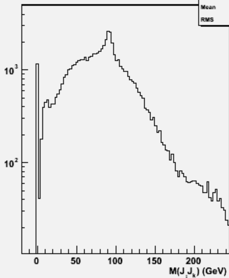
2jets mass(All comb)w102268 n2n2ssbb_o
