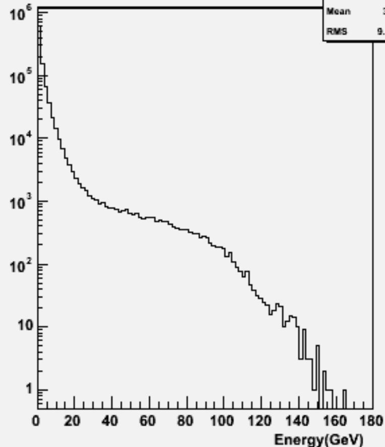
Particle Energy : w102268 n2n2ssbb_o
