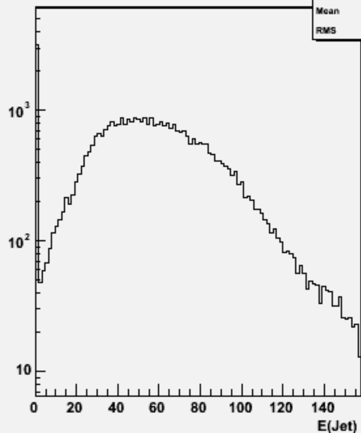
Jet energies(All jets)w102268 n2n2ssbb_o
