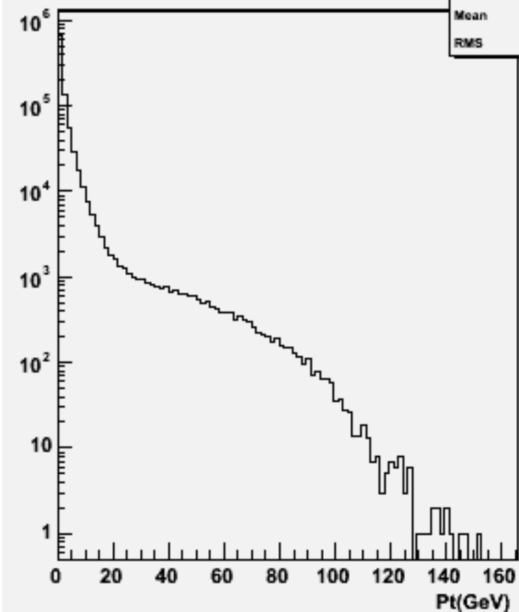
Particle Pt : w102268 n2n2ssbb_o
