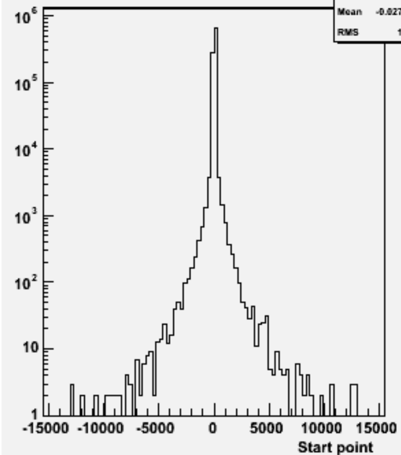
Start point Z : w102268 n2n2ssbb_o
