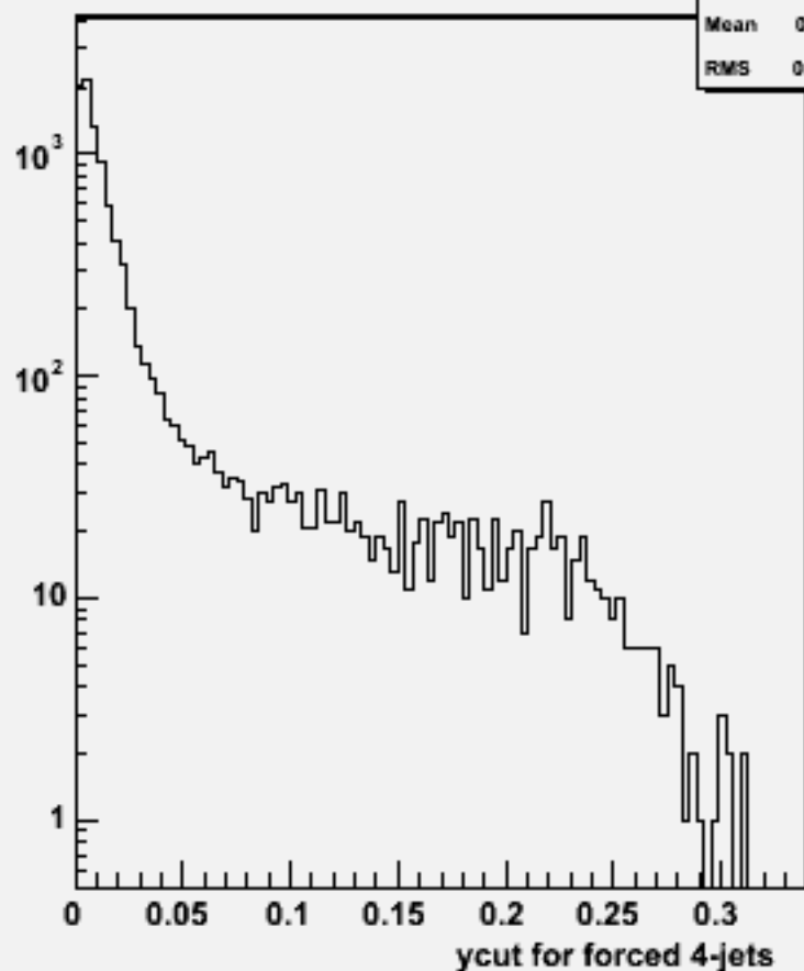
Ycut for 4-jets :w102268 n2n2ssbb_o
