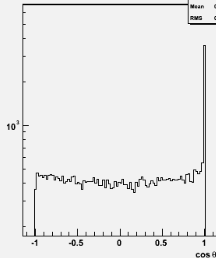
Jet cos \theta (All jets)w102268 n2n2ssbb_o
