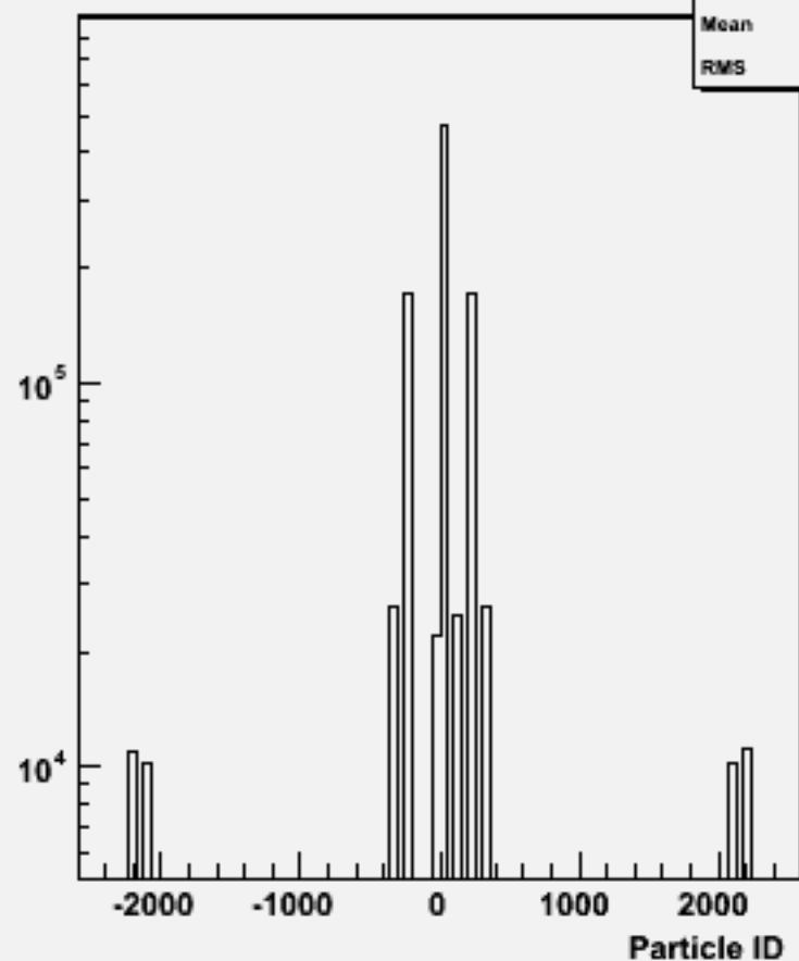
Particle ID : w102268 n2n2ssbb_o
