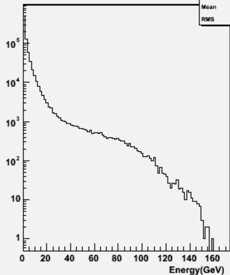
Particle Energy : w102265 n2n2ssss_o
