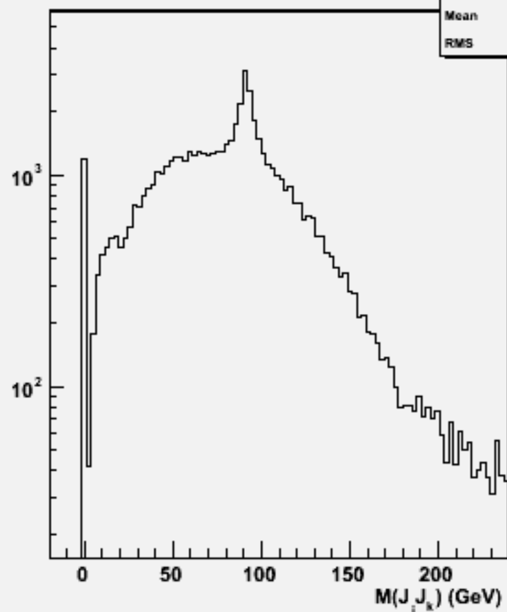
2jets mass(All comb)w102265 n2n2ssss_o
