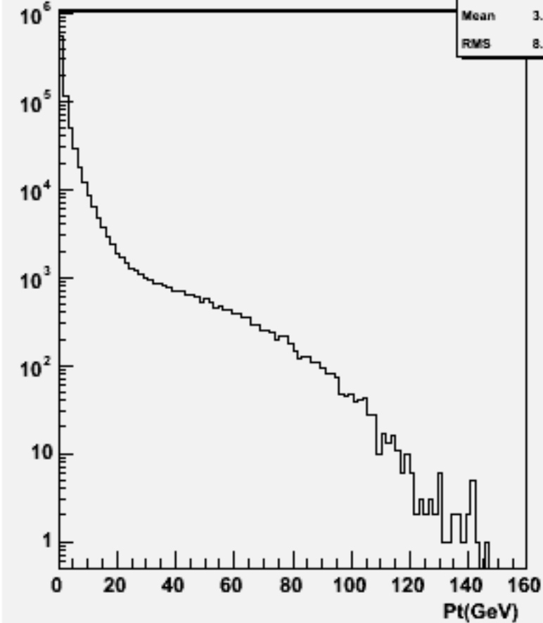
Particle Pt : w102265 n2n2ssss_o
