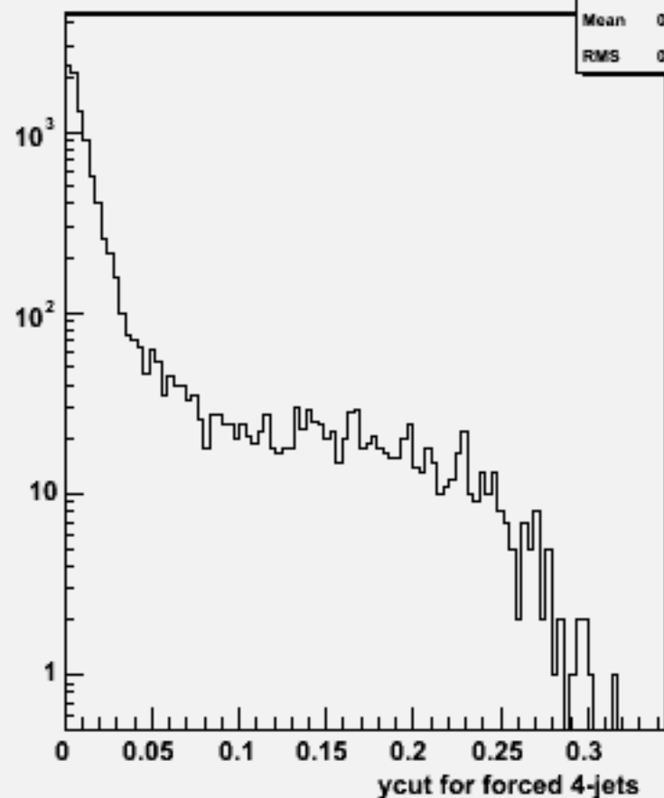
Ycut for 4-jets :w102265 n2n2ssss_o
