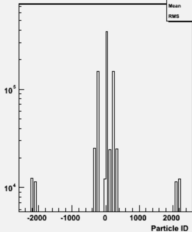
Particle ID : w102265 n2n2ssss_o
