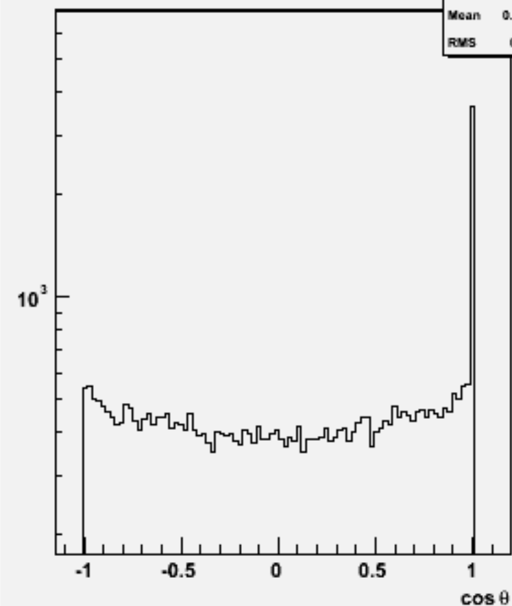
Jet cosθ (All jets)w102265 n2n2ssss_o
