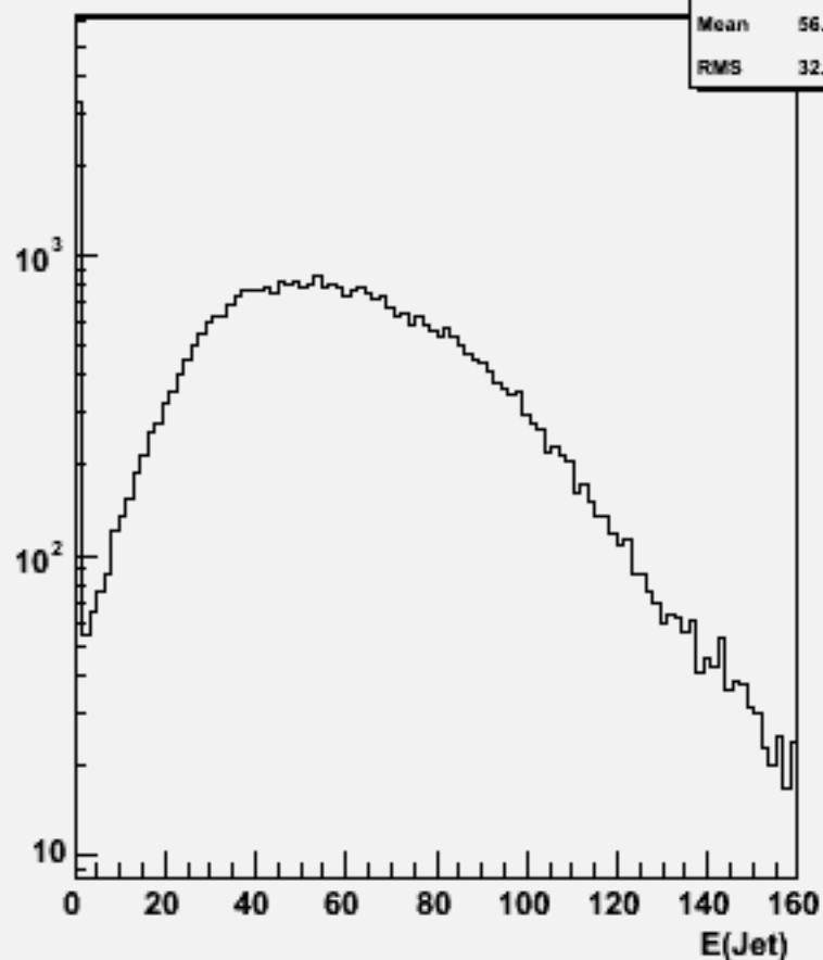
Jet energies(All jets)w102265 n2n2ssss_o
