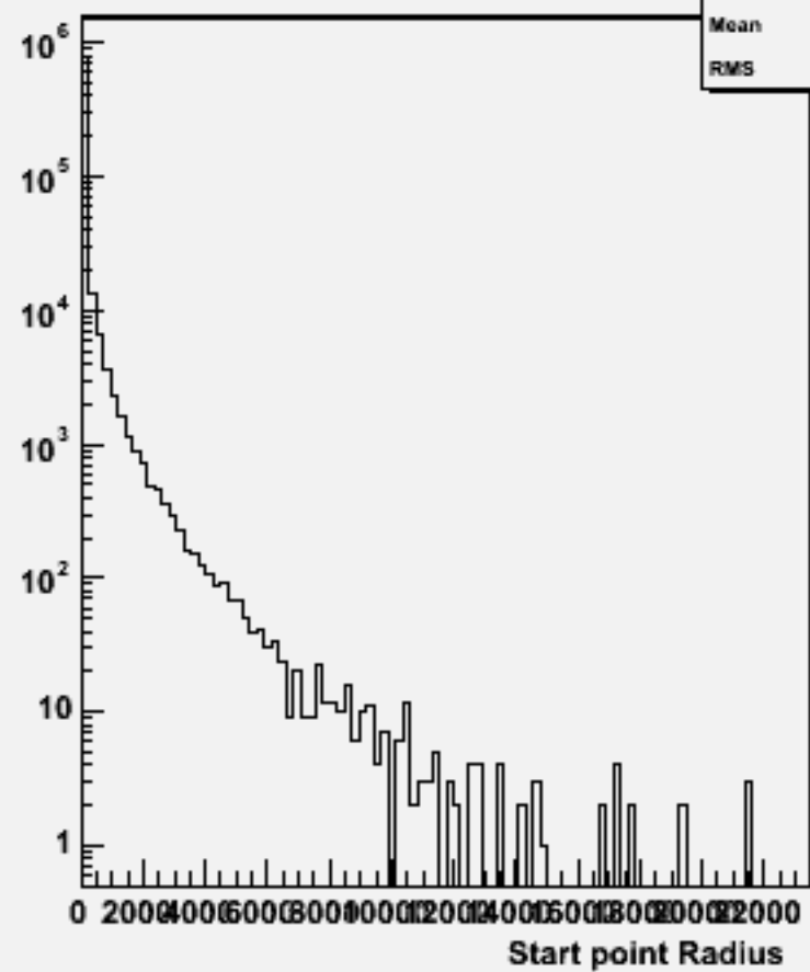
Start point R : w102265 n2n2ssss_o
