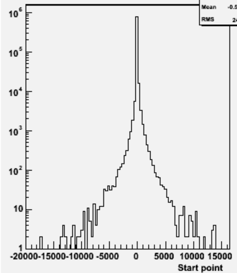
Start point Z : w102265 n2n2ssss_o
