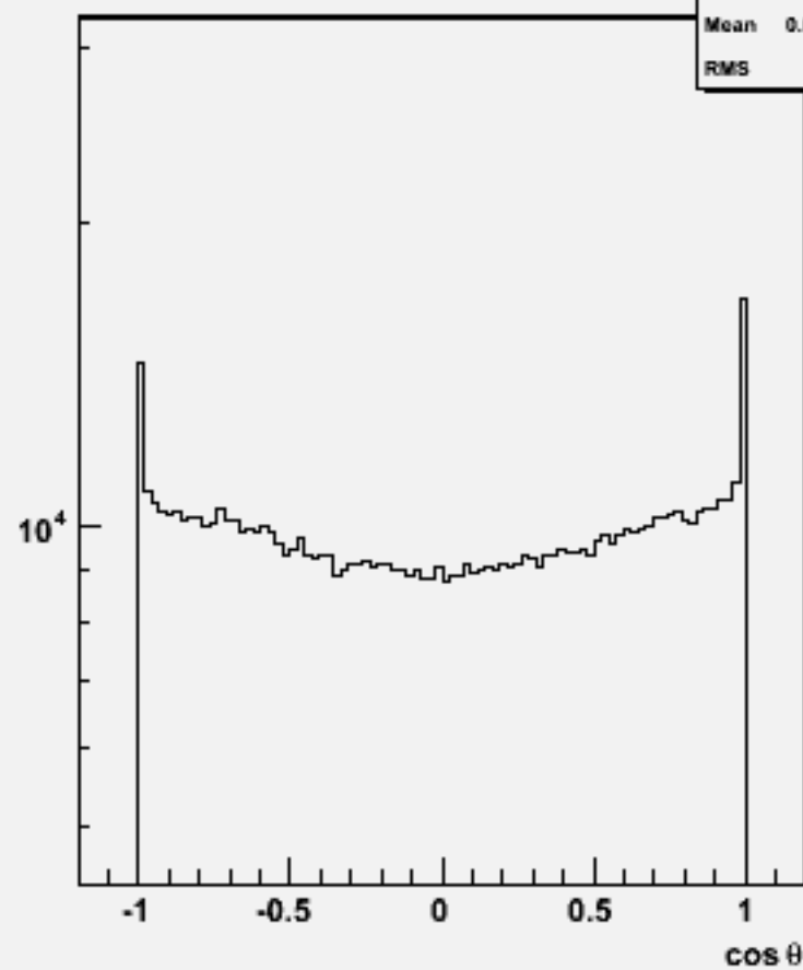
Particle cos \theta : w102265 n2n2ssss_o
