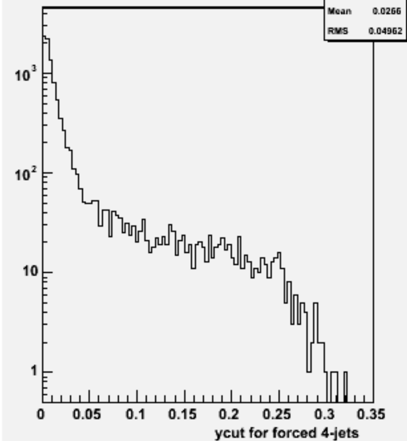
Ycut for 4-jets :w102261 n2n2ddbb_o
