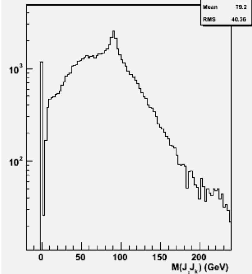
2jets mass(All comb)w102261 n2n2ddbb_o
