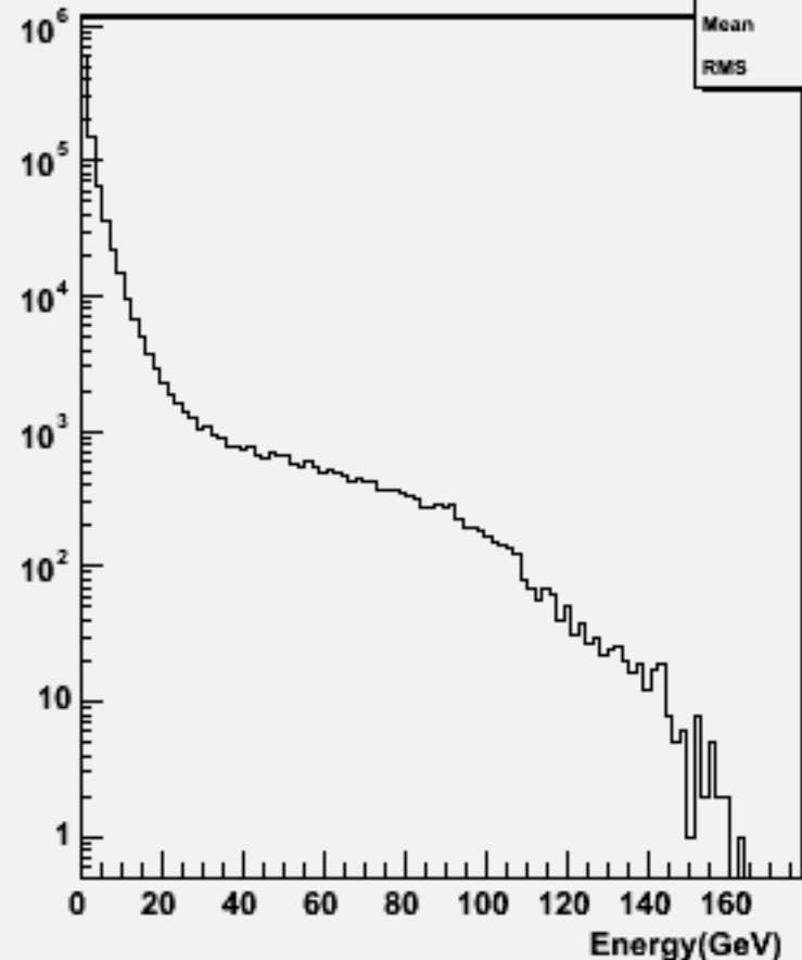
Particle Energy : w102261 n2n2ddbb_o
