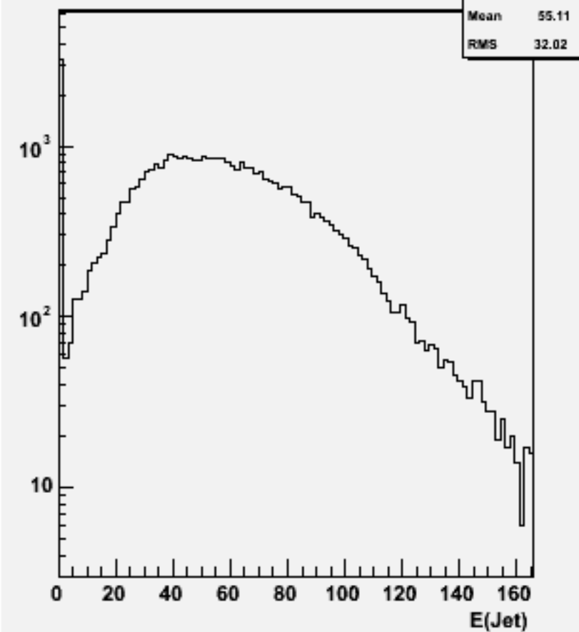
Jet energies(All jets)w102261 n2n2ddbb_o
