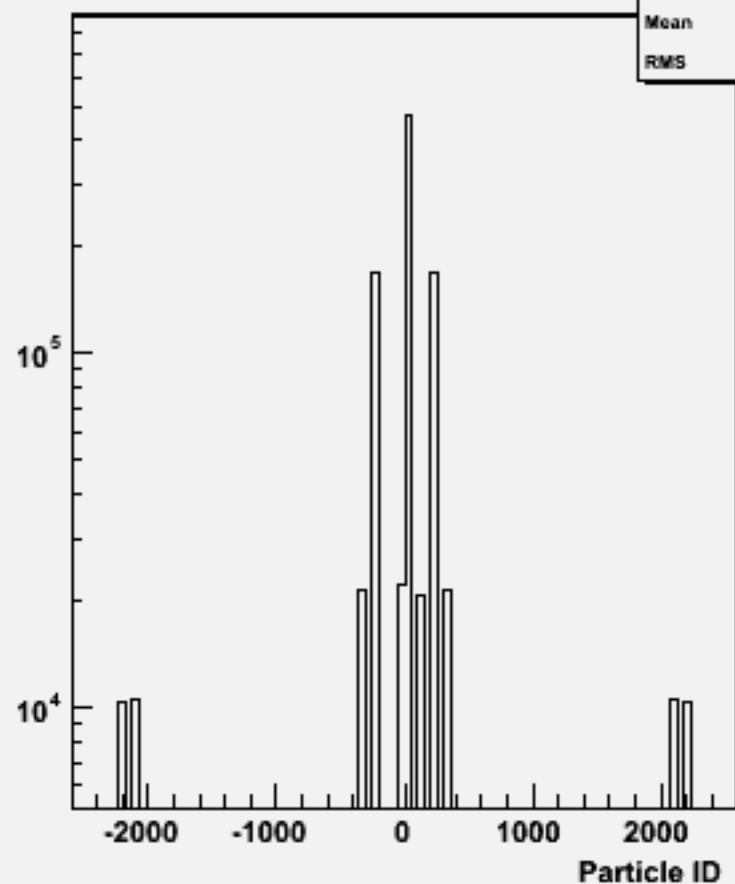
Particle ID : w102261 n2n2ddbb_o
