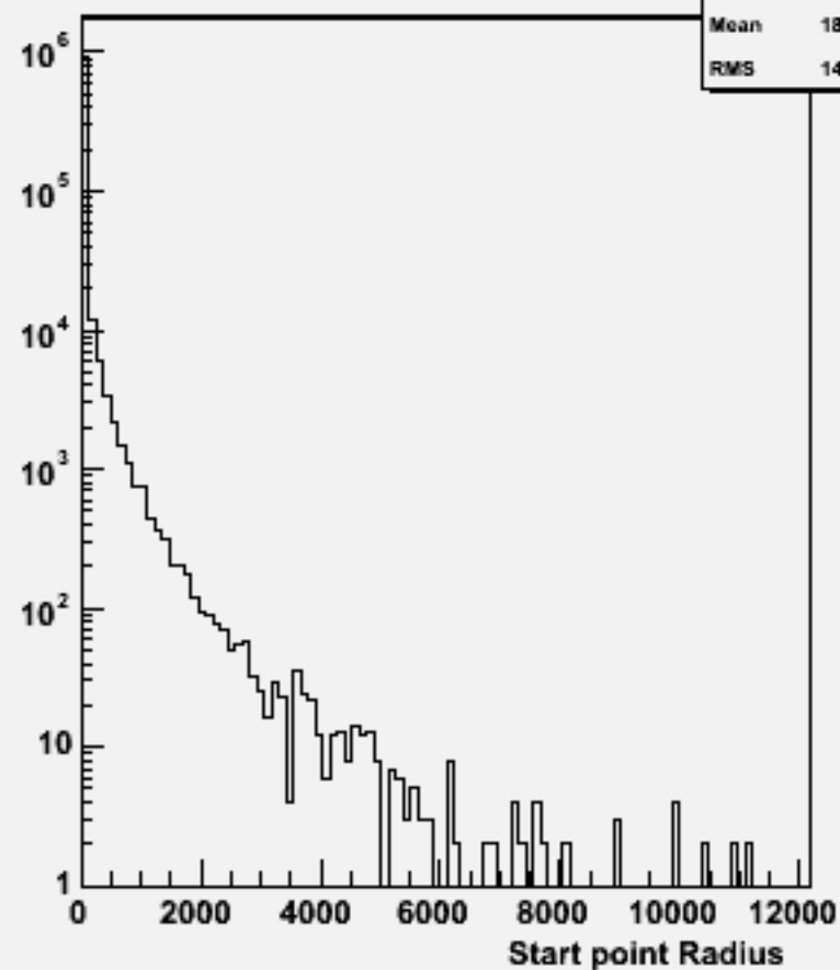
Start point R : w102261 n2n2ddbb_o
