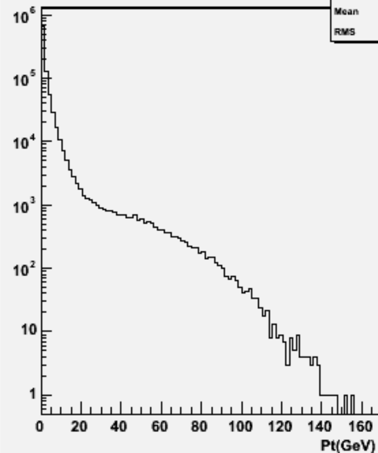
Particle Pt : w102261 n2n2ddbb_o
