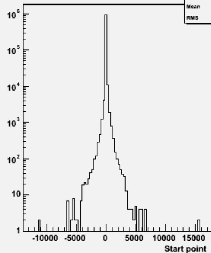
Start point Z : w102261 n2n2ddbb_o
