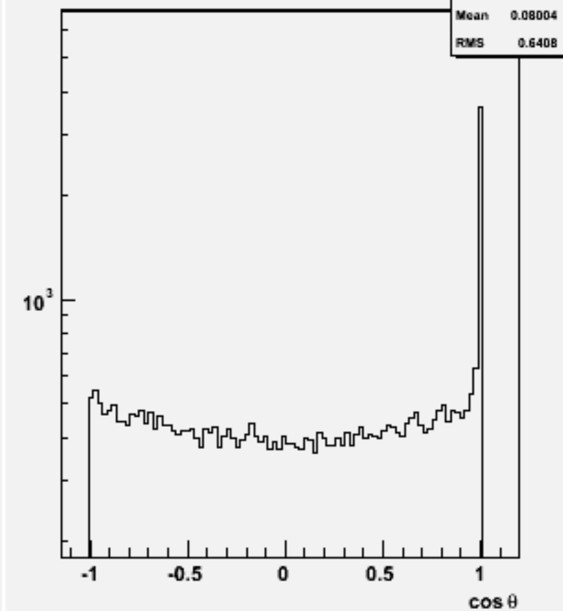
Jet cosθ (All jets)w102261 n2n2ddbb_o
