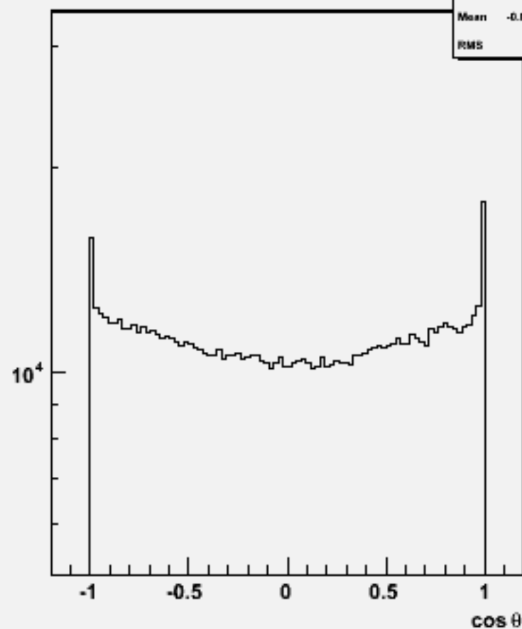
Particle cos \theta : w102261 n2n2ddbb_o
