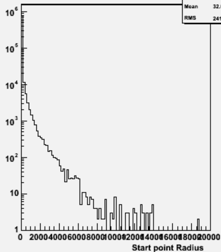
Start point R : w102257 n2n2ddss_o
