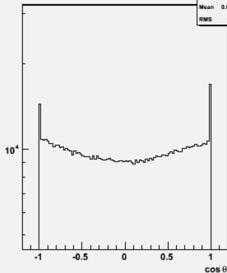
Particle cos \theta : w102257 n2n2ddss_o
