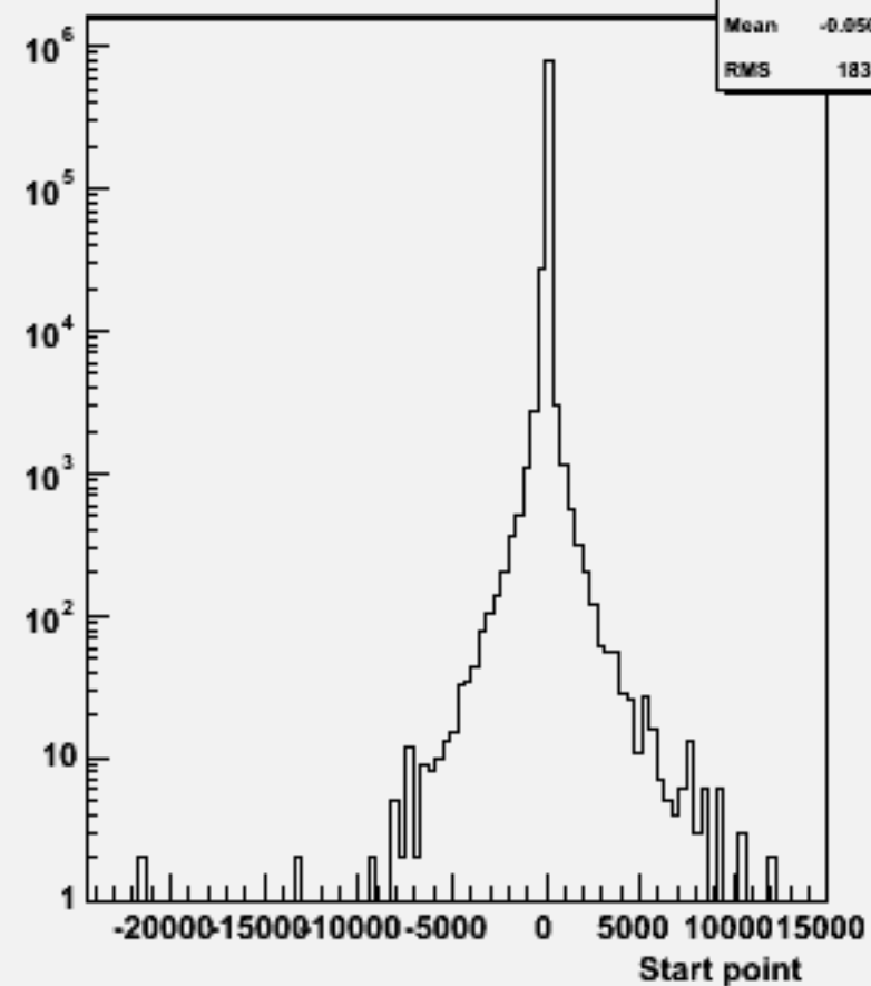
Start point Z : w102256 n2n2ddss_o
