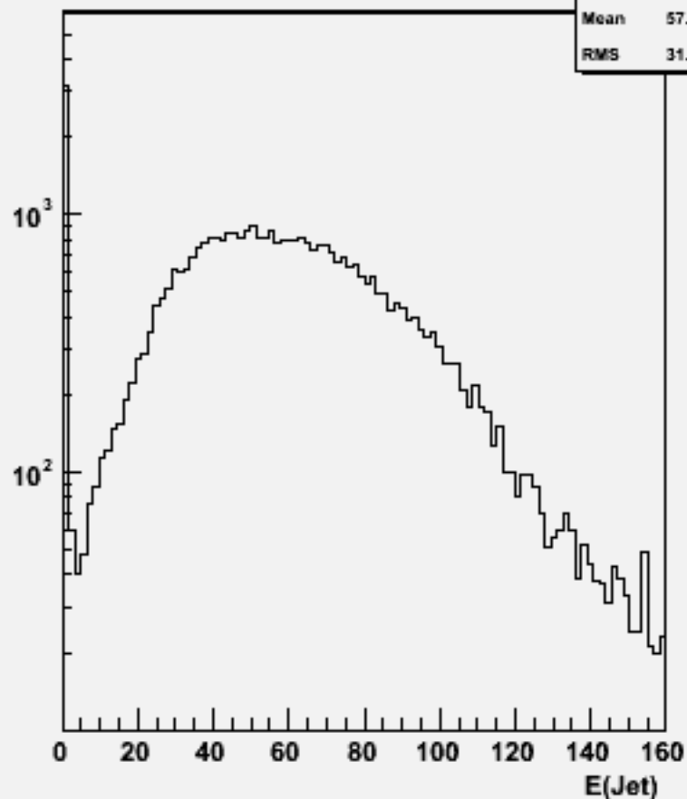
Jet energies(All jets)w102256 n2n2ddss_o
