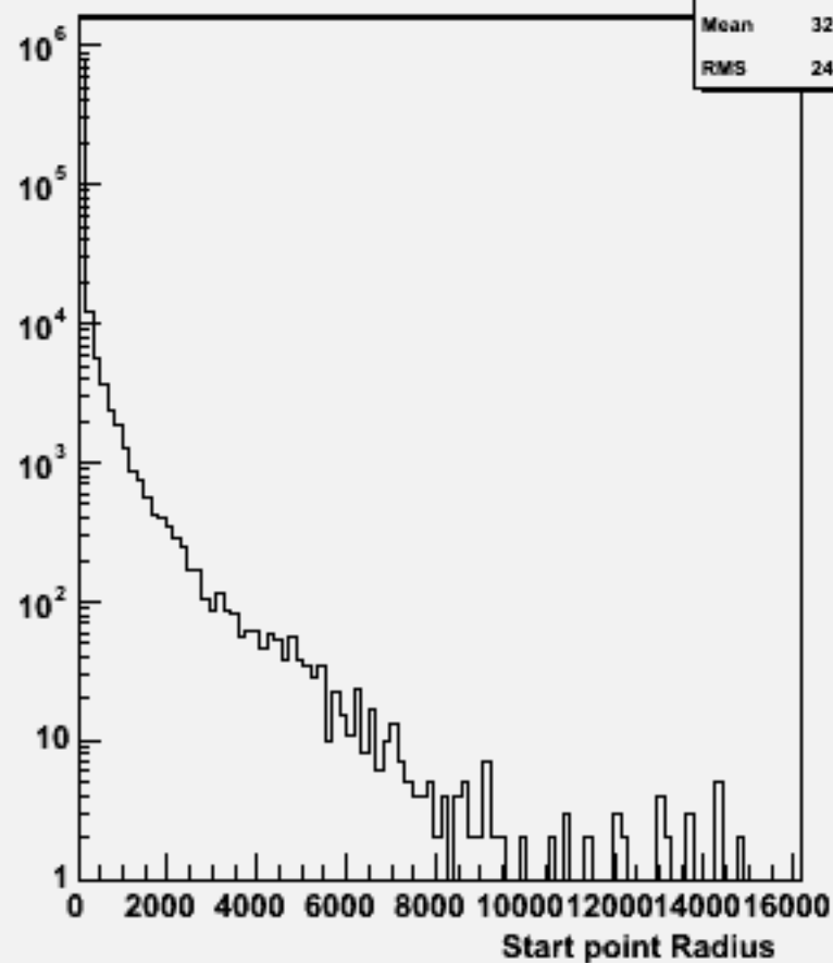
Start point R : w102256 n2n2ddss_o
