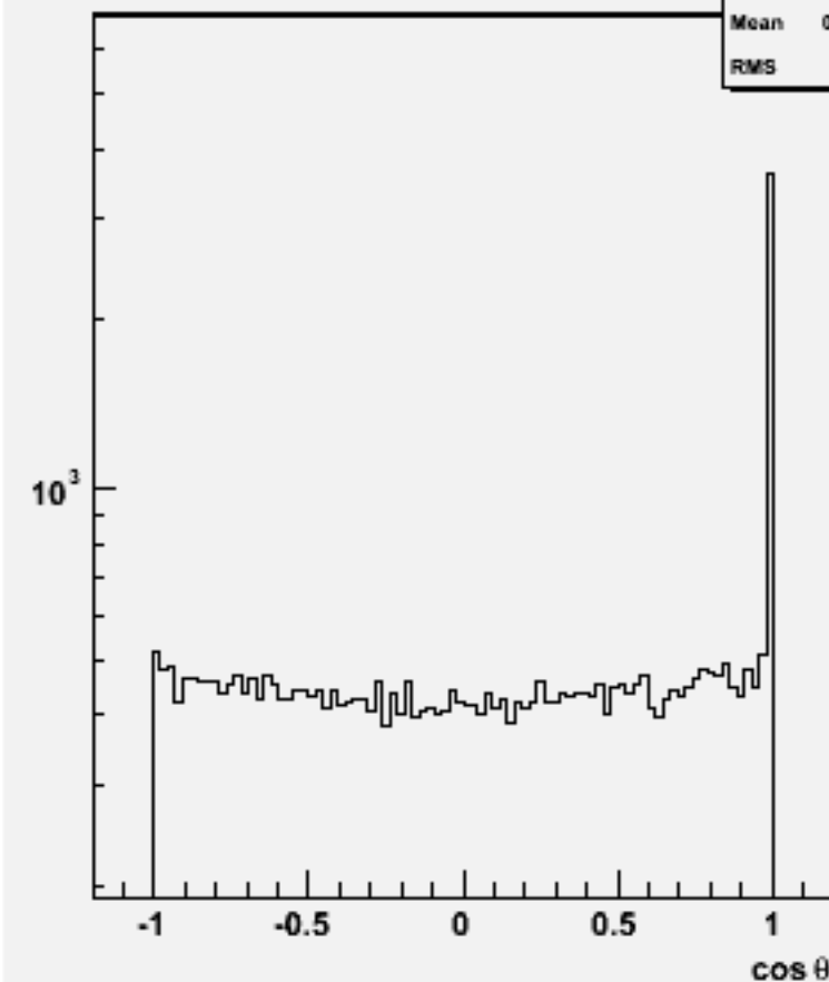
Jet cos \theta (All jets)w102256 n2n2ddss_o
