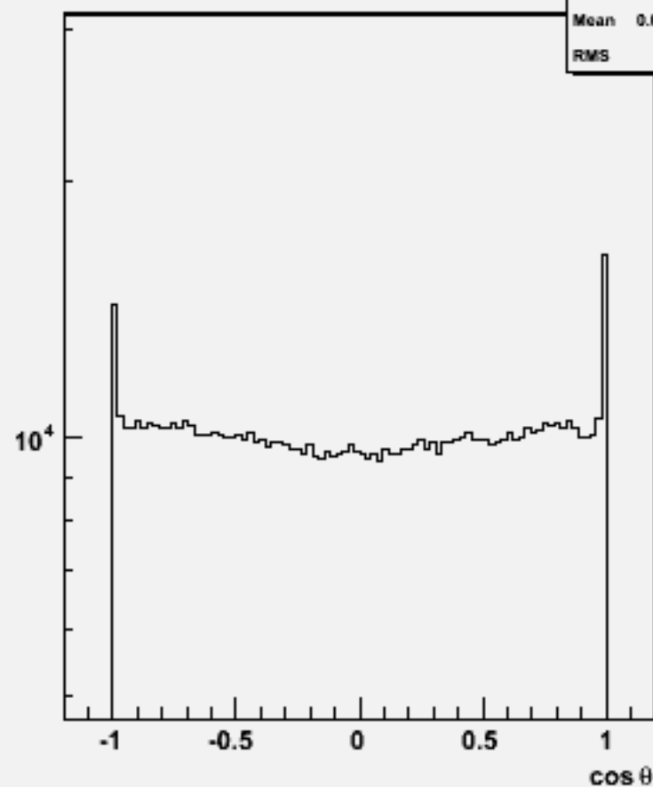
Particle cos \theta : w102256 n2n2ddss_o
