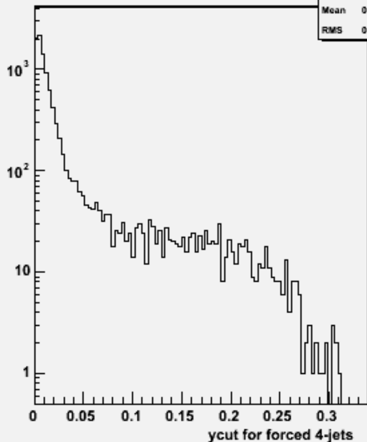
Ycut for 4-jets :w102256 n2n2ddss_o
