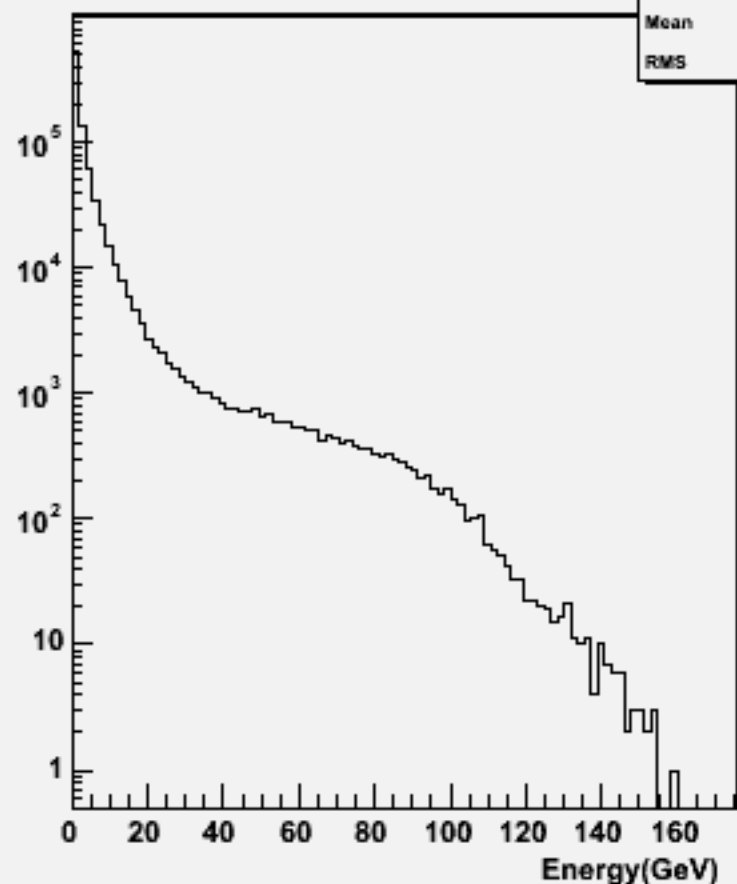
Particle Energy : w102256 n2n2ddss_o
