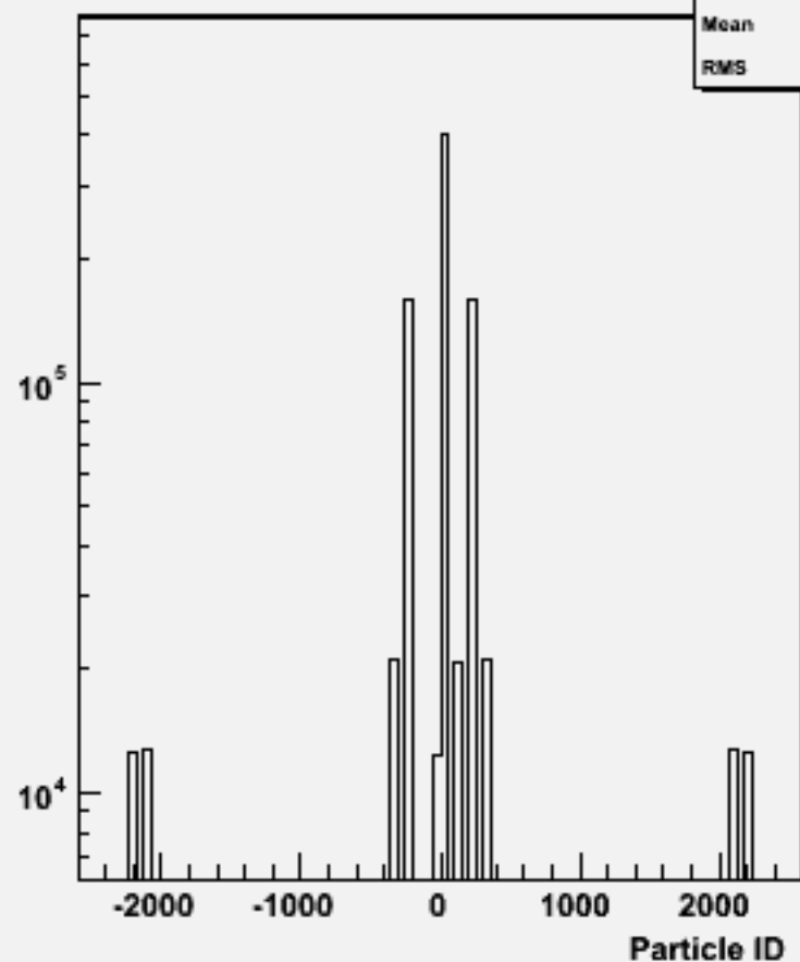
Particle ID : w102256 n2n2ddss_o
