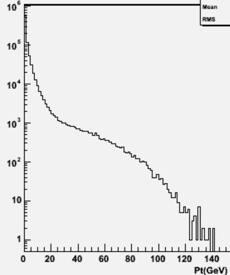
Particle Pt : w102256 n2n2ddss_o
