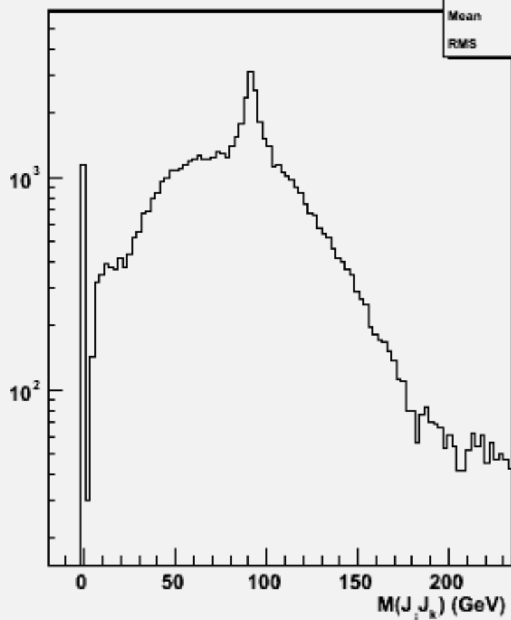
2jets mass(All comb)w102256 n2n2ddss_o
