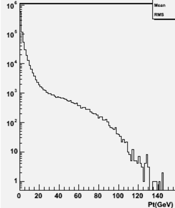
Particle Pt : w102252 n2n2dddd_o
