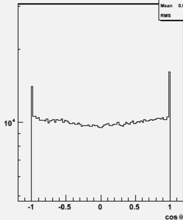
Particle cos \theta : w102252 n2n2dddd_o
