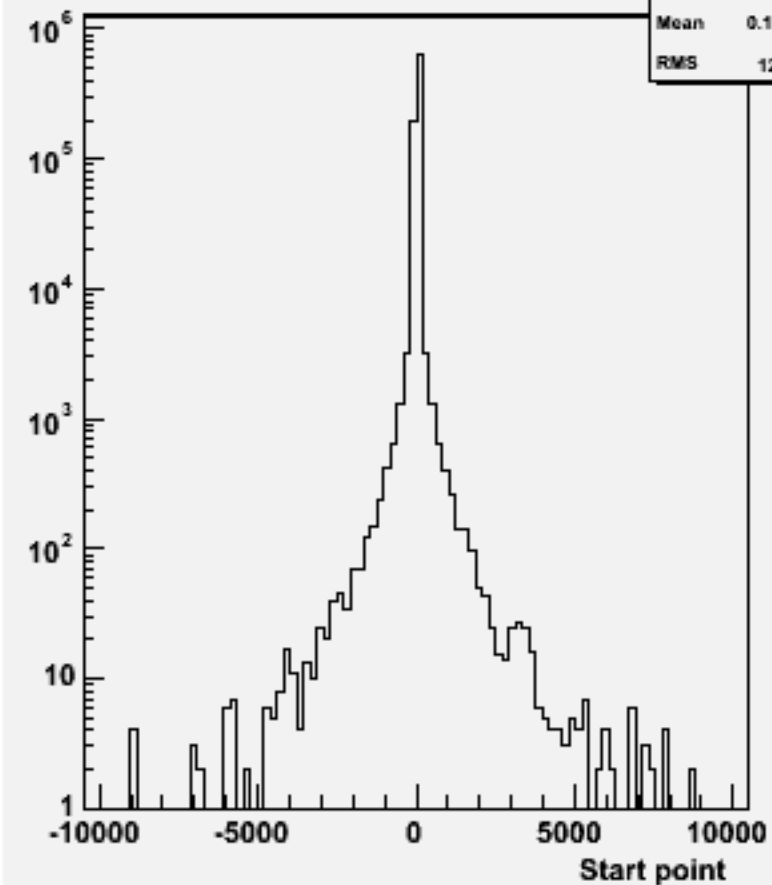
Start point Z : w102252 n2n2dddd_o
