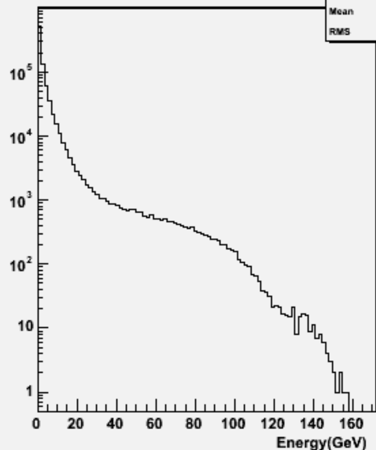
Particle Energy : w102252 n2n2dddd_o
