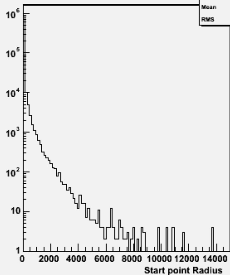
Start point R : w102252 n2n2dddd_o
