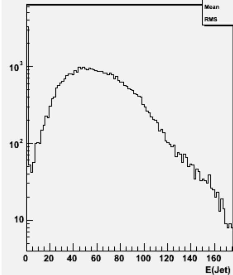
Jet energies(All jets)w102252 n2n2dddd_o
