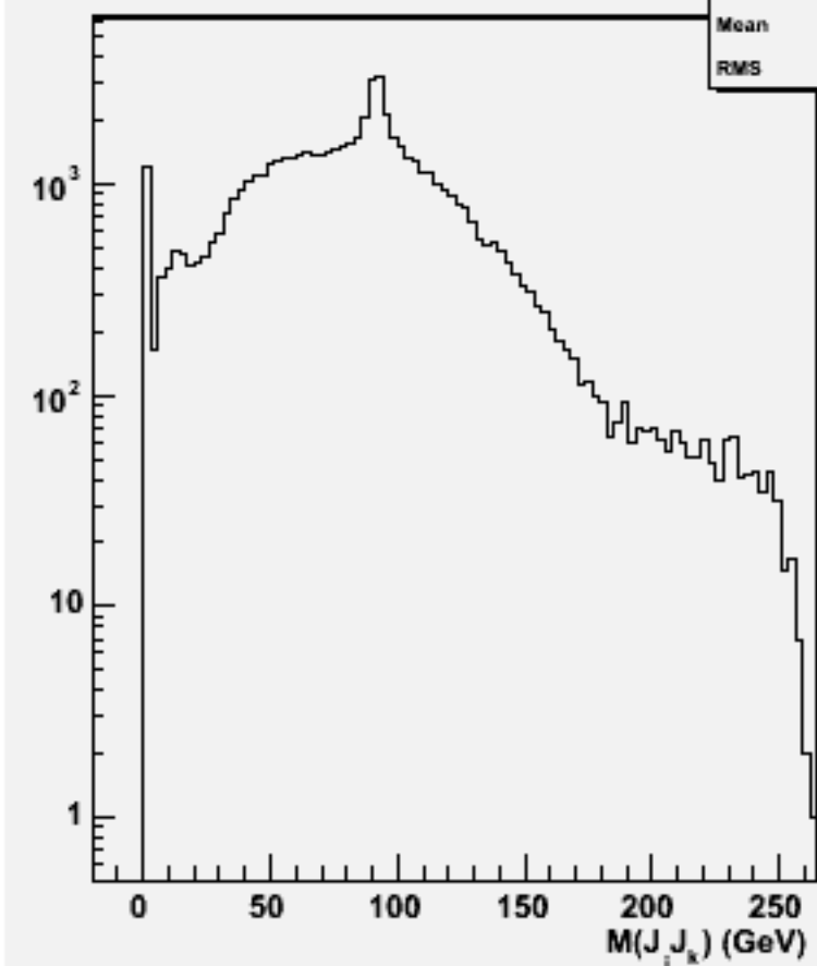
2jets mass(All comb)w102252 n2n2dddd_o
