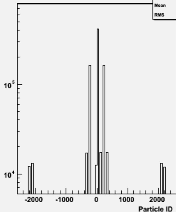
Particle ID : w102252 n2n2dddd_o
