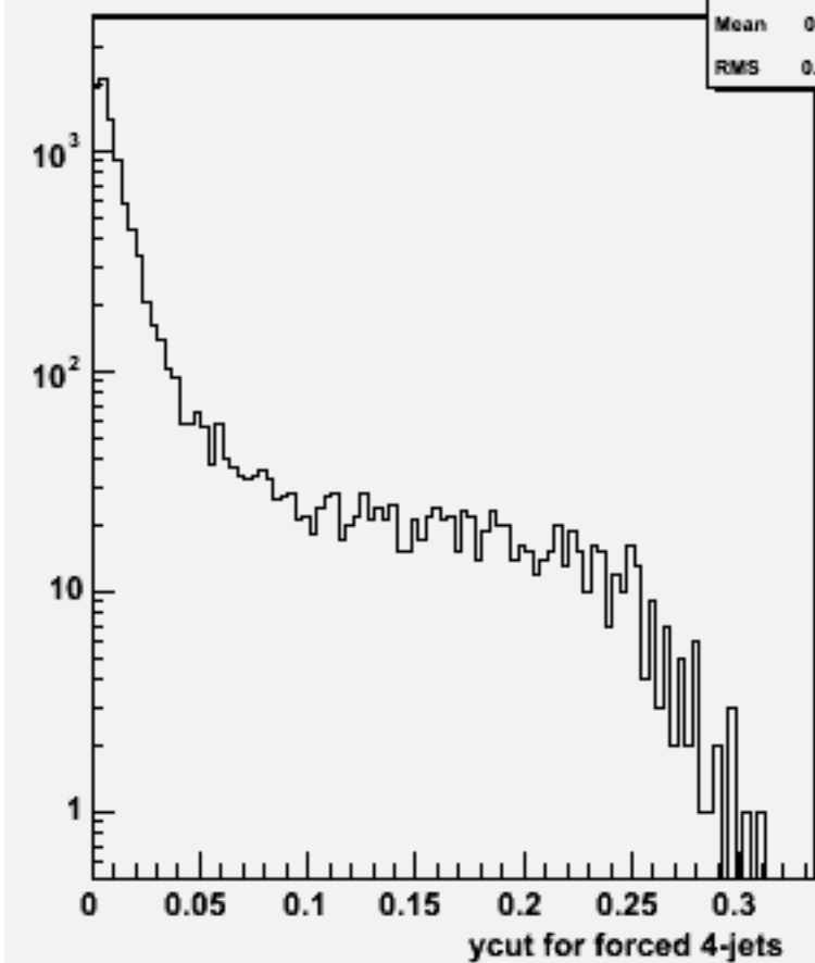
Ycut for 4-jets :w102252 n2n2dddd_o
