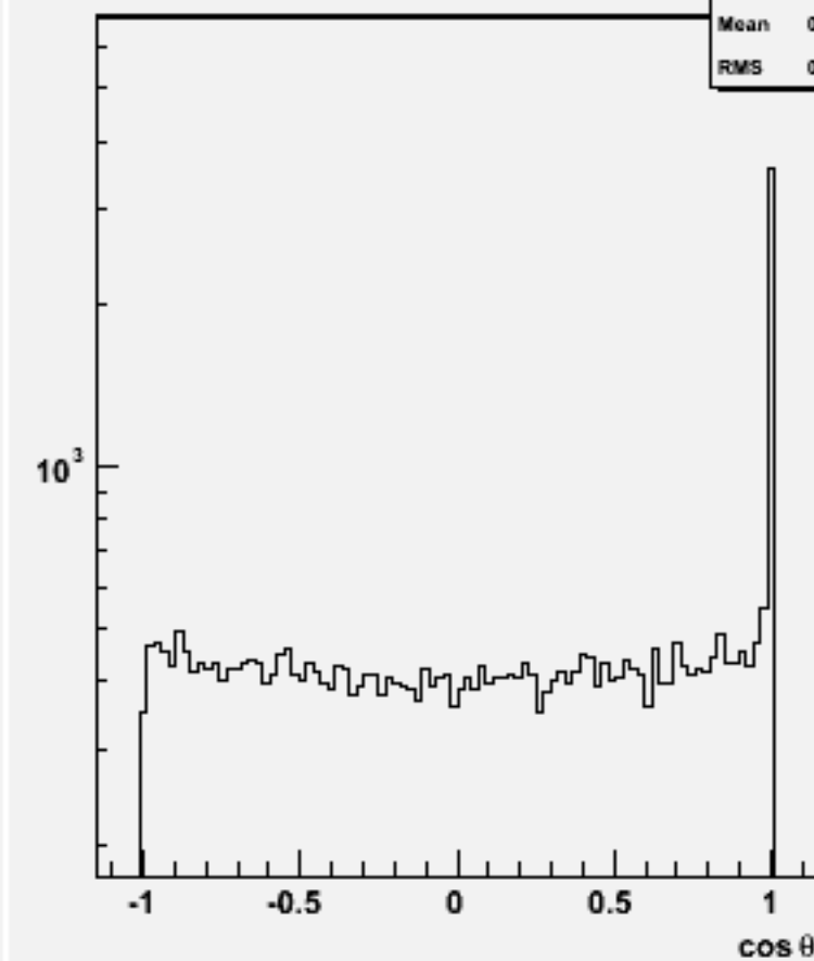
Jet cos \theta (All jets)w102252 n2n2dddd_o
