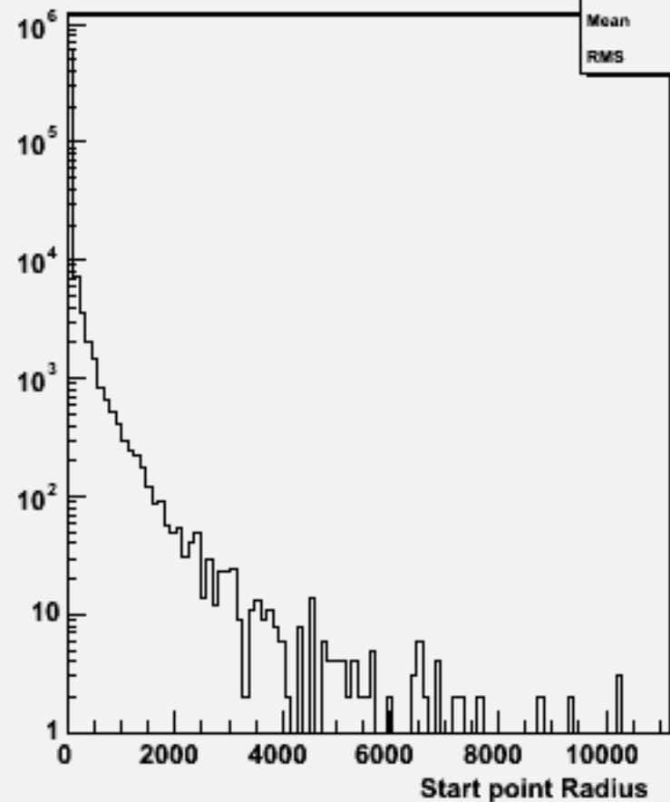
Start point R : w102249 n2n2e3e3bb_o
