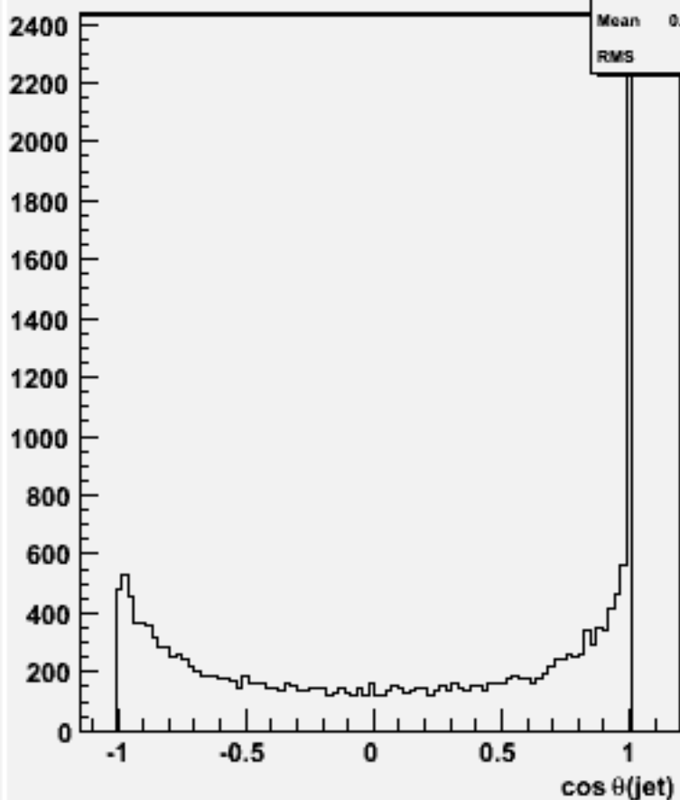
cos \theta for 2-jets :w102249 n2n2e3e3bb_o
