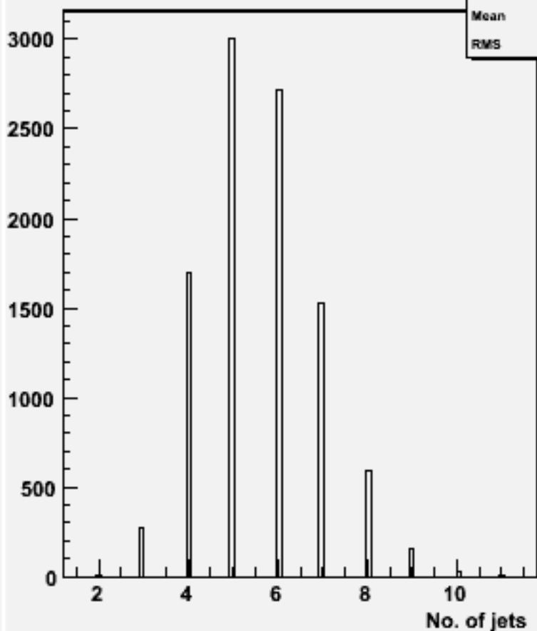
No. jets (ycut=0.001) : w102249 n2n2e3e3bb_o
