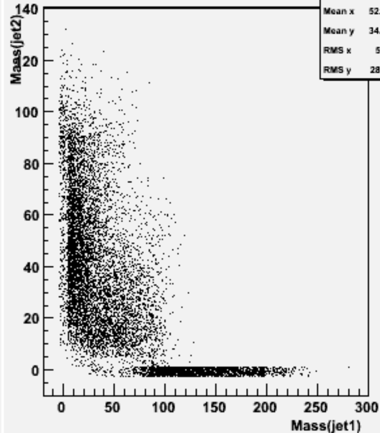
Jet mass for forced 2-jets : w102249 n2n2e3e3bb_o
