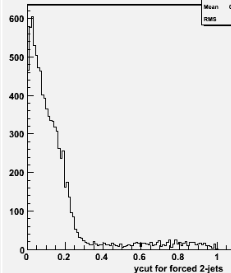
Ycut for 2-jets :w102249 n2n2e3e3bb_o
