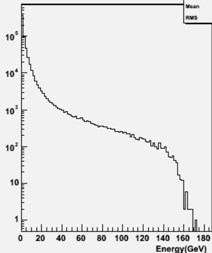
Particle Energy : w102249 n2n2e3e3bb_o
