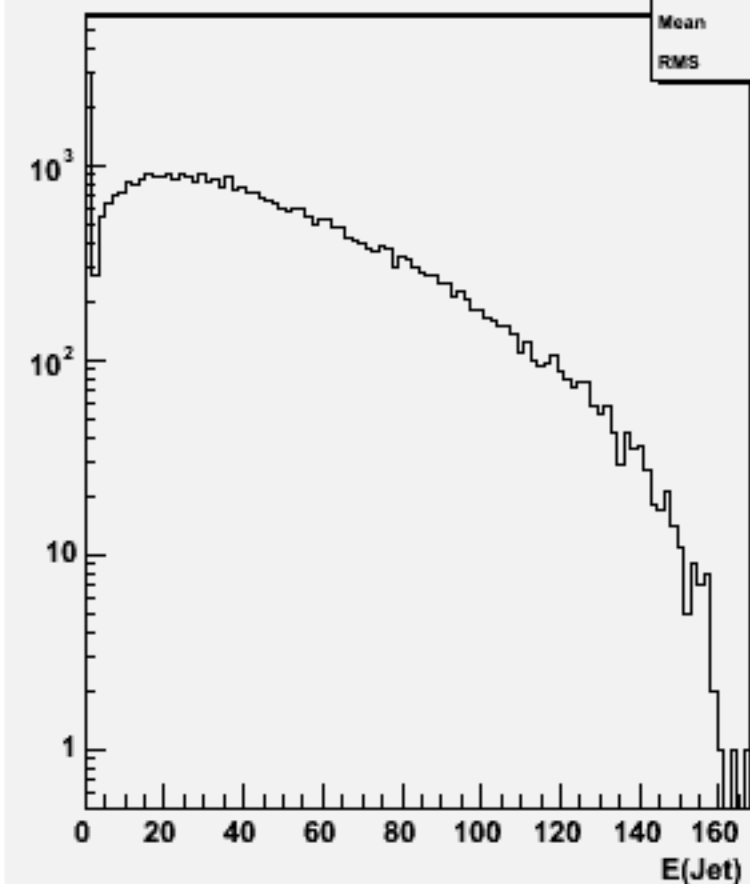
Jet energies(All jets)w102249 n2n2e3e3bb_o
