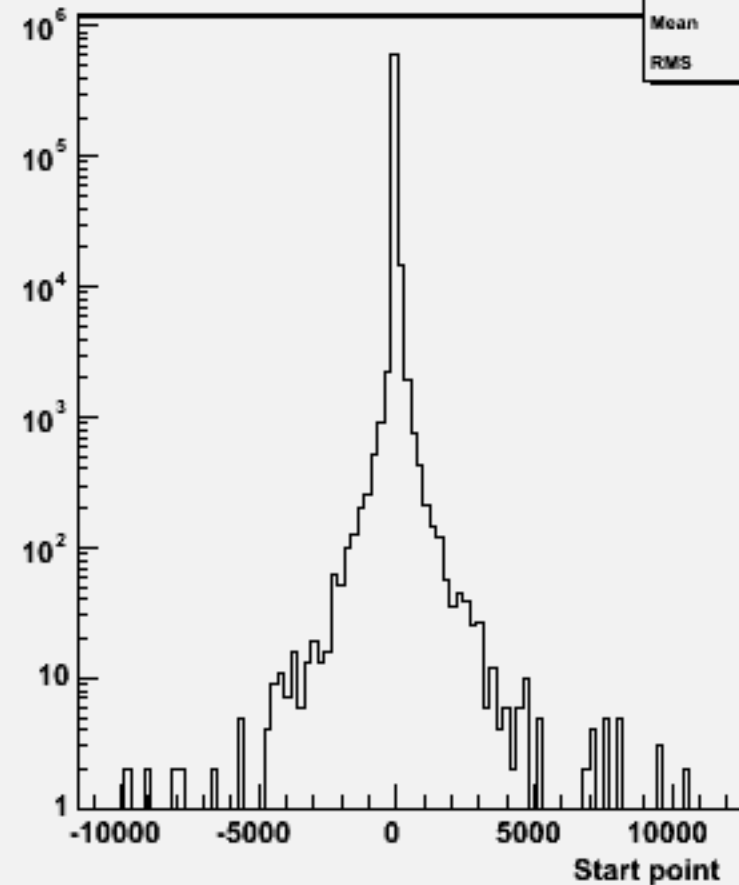
Start point Z : w102249 n2n2e3e3bb_o
