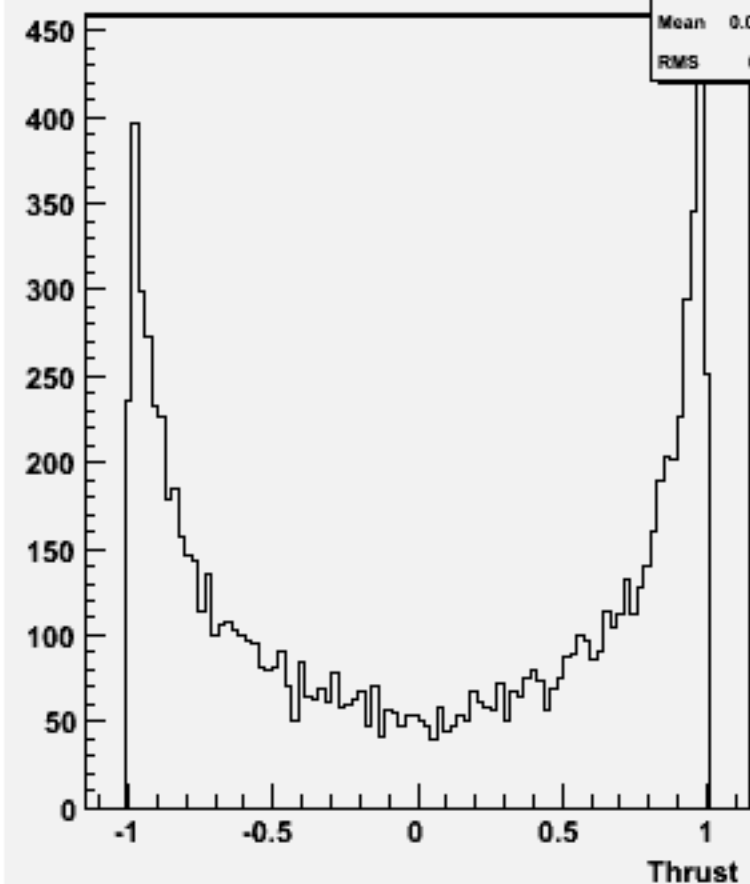
cos \Theta (thrust) w102249 n2n2e3e3bb_o
