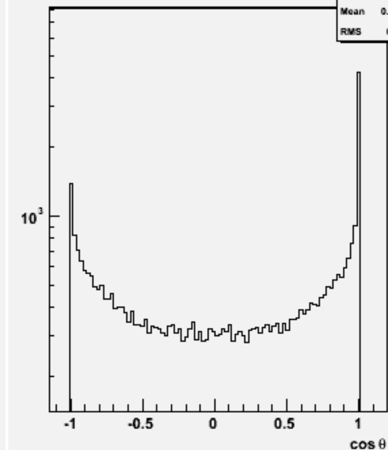
Jet cos \theta (All jets)w102249 n2n2e3e3bb_o
