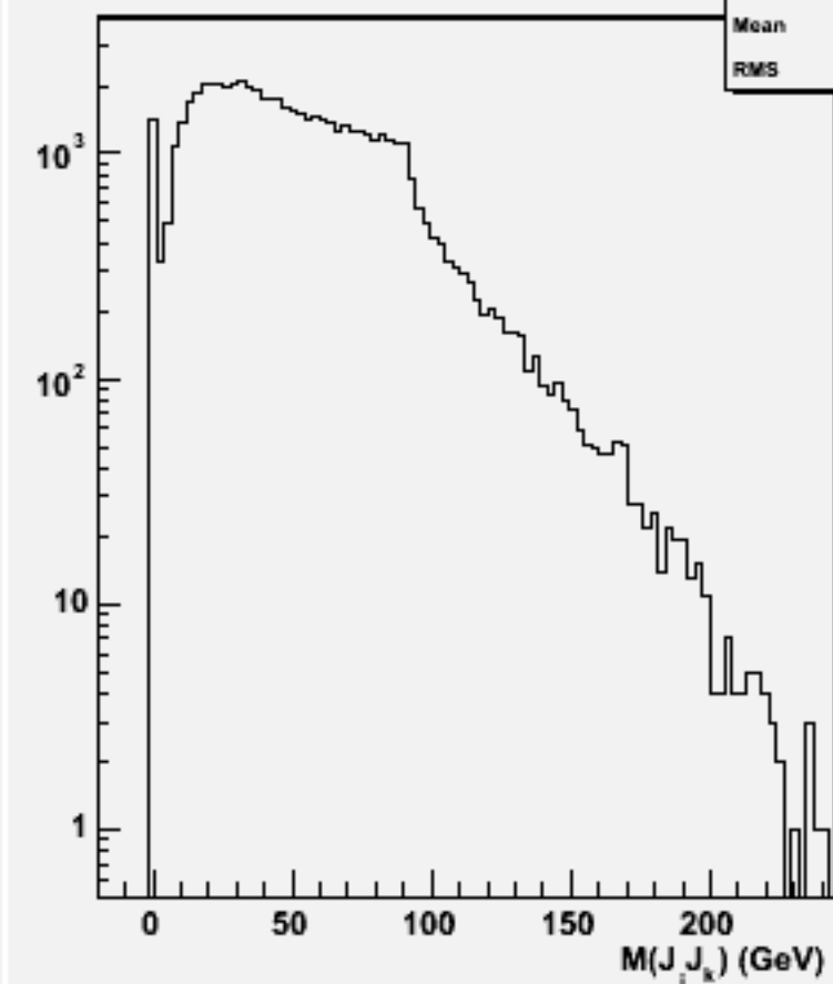
2jets mass(All comb)w102249 n2n2e3e3bb_o
