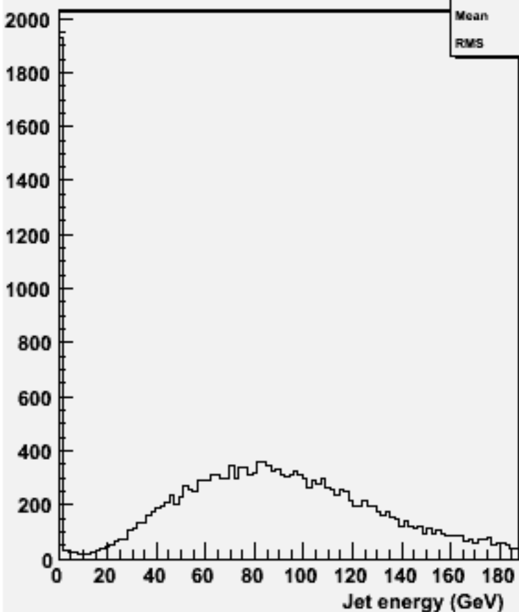
energy for 2-jets :w102249 n2n2e3e3bb_o
