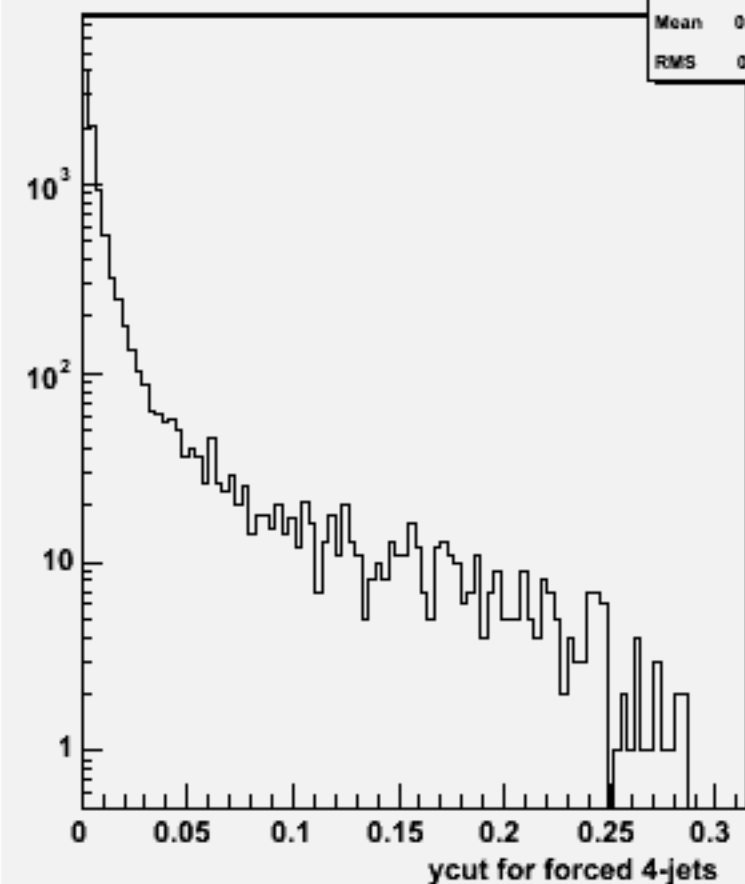
Ycut for 4-jets :w102248 n2n2e3e3bb_o
