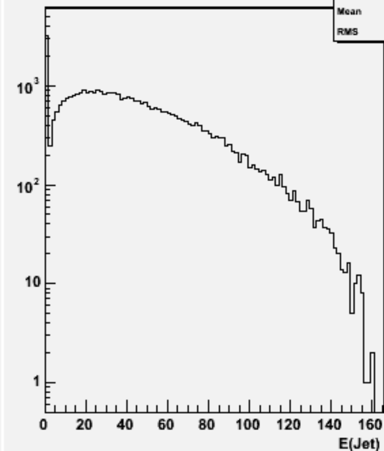
Jet energies(All jets)w102248 n2n2e3e3bb_o
