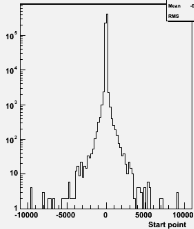
Start point Z : w102248 n2n2e3e3bb_o
