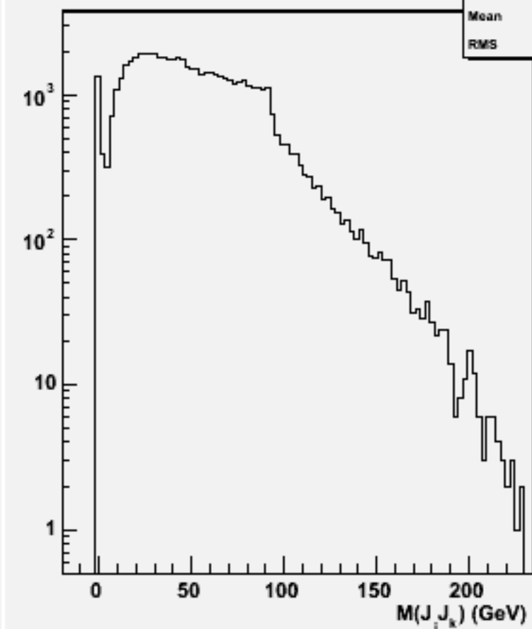
2jets mass(All comb)w102248 n2n2e3e3bb_o
