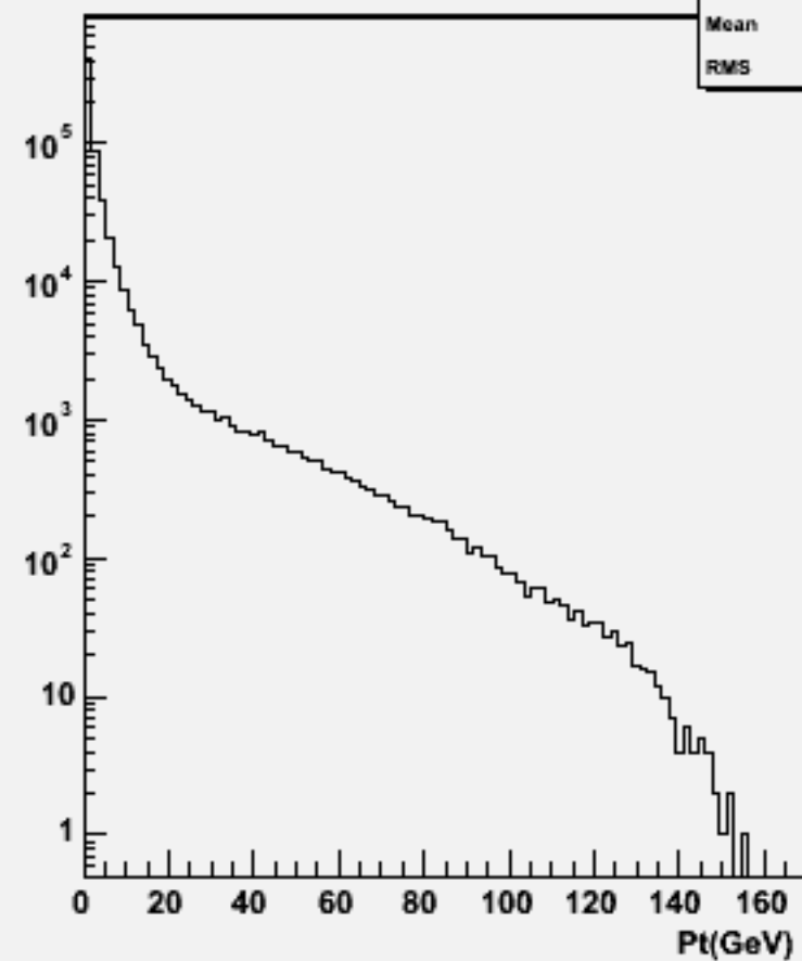
Start point Z : w102248 n2n2e3e3bb_o
