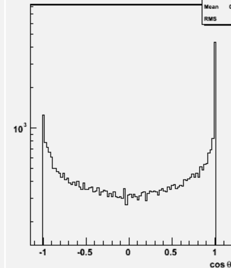
Jet cos \theta (All jets)w102248 n2n2e3e3bb_o
