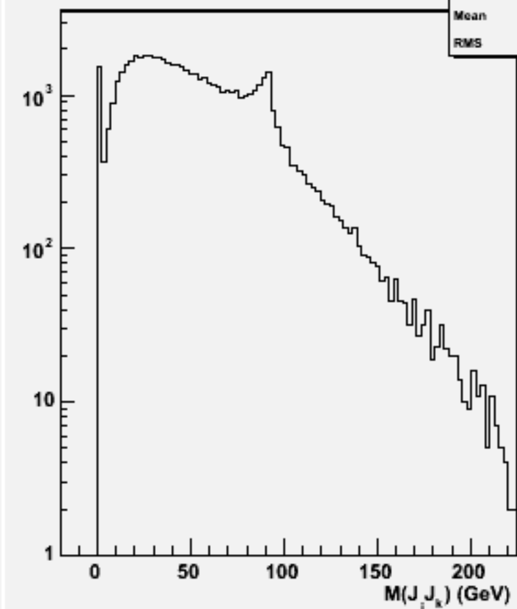
2jets mass(All comb)w102245 n2n2e3e3ss_o
