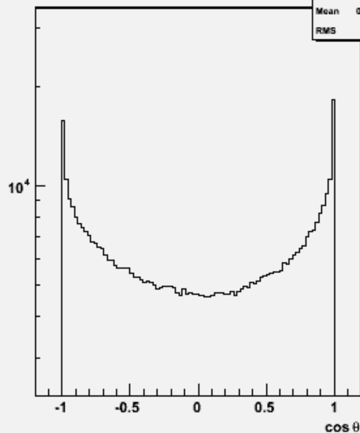
Particle cosθ : w102245 n2n2e3e3ss_o
