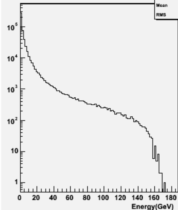
Particle Energy : w102245 n2n2e3e3ss_o
