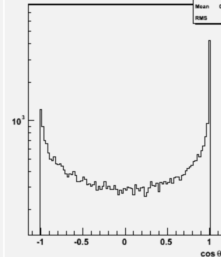
Jet cos \theta (All jets)w102245 n2n2e3e3ss_o
