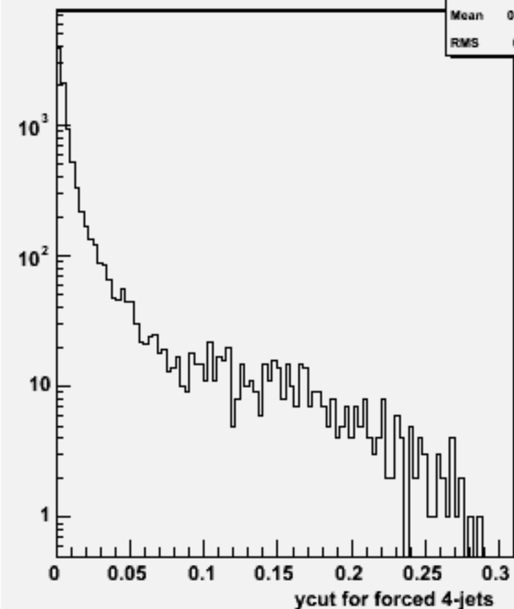
Ycut for 4-jets :w102245 n2n2e3e3ss_o
