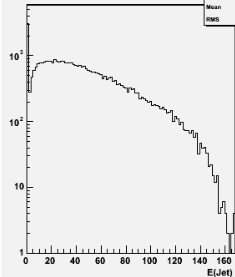
Jet energies(All jets)w102245 n2n2e3e3ss_o
