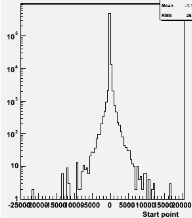
Start point Z : w102245 n2n2e3e3ss_o
