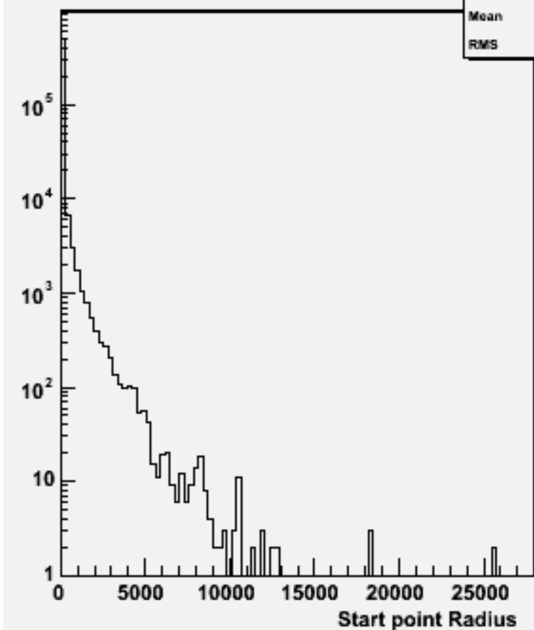
Start point R : w102245 n2n2e3e3ss_o
