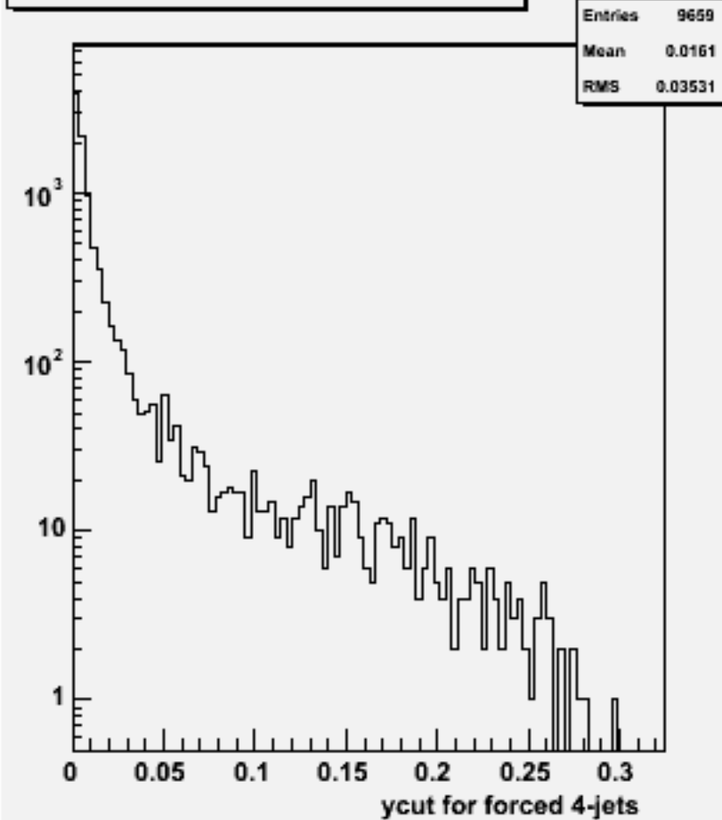
Ycut for 4-jets :w102244 n2n2e3e3ss_o
