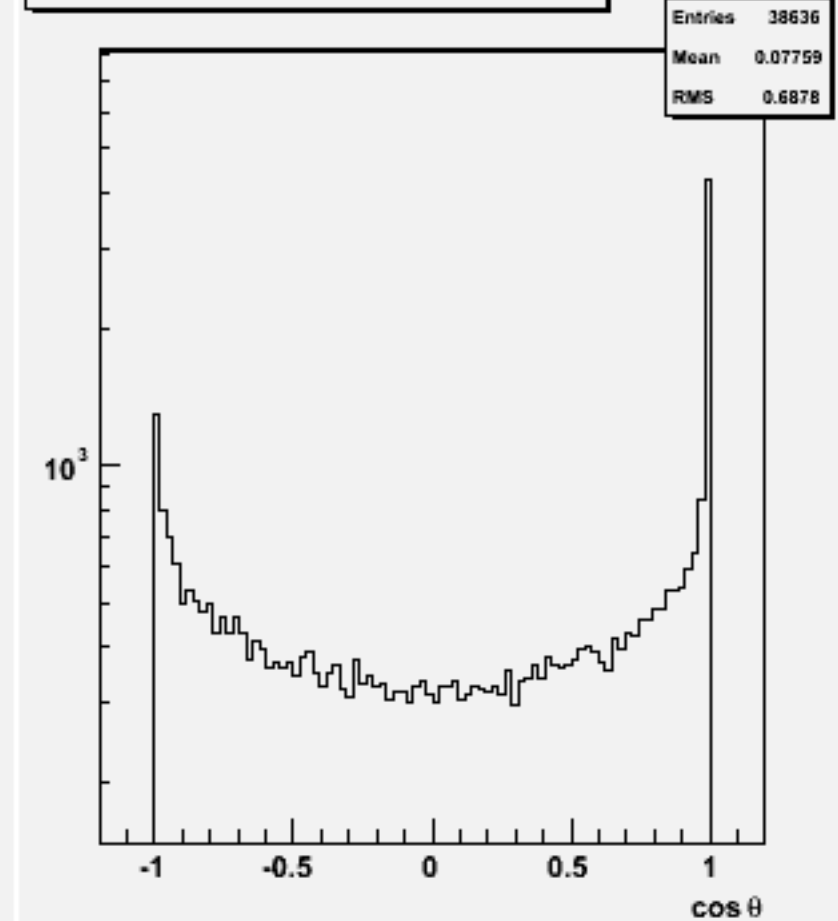
Jet cos \theta (All jets)w102244 n2n2e3e3ss_o
