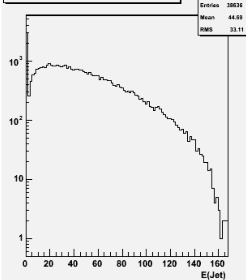
Jet energies(All jets)w102244 n2n2e3e3ss_o
