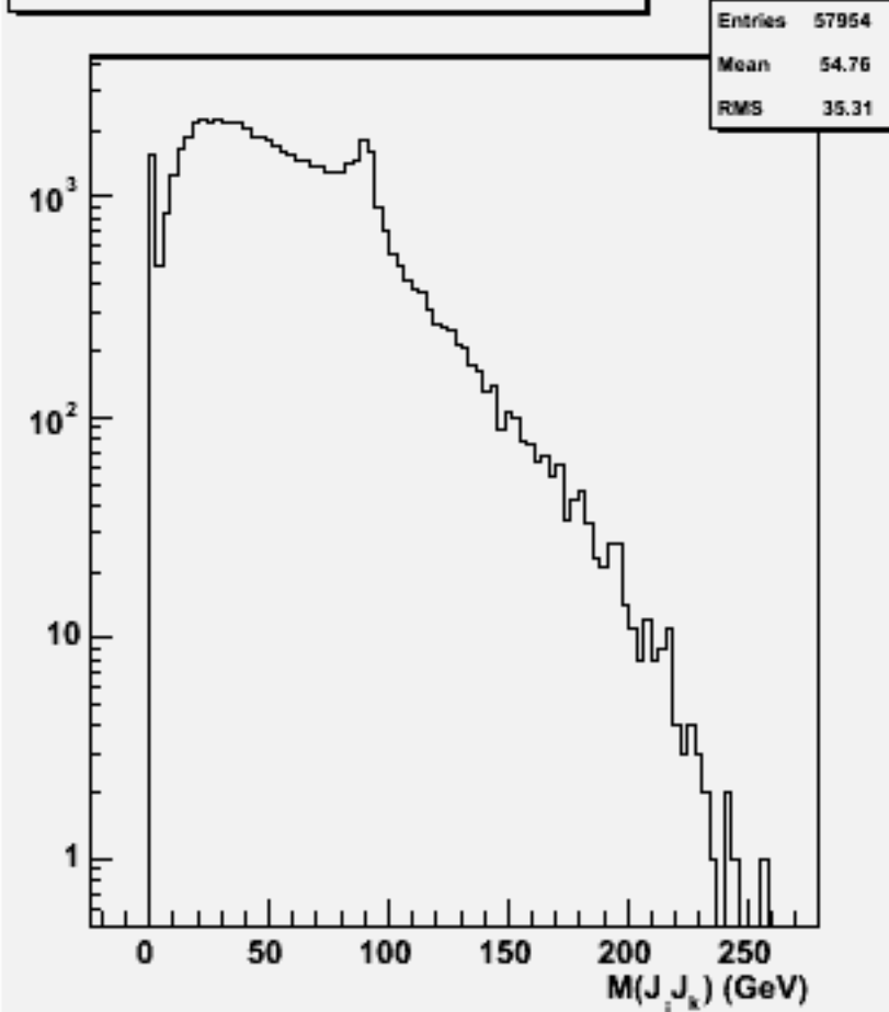
2jets mass(All comb)w102244 n2n2e3e3ss_o
