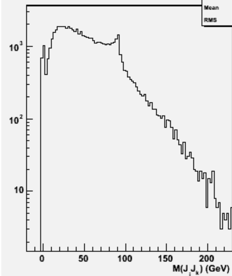
2jets mass(All comb)w102241 n2n2e3e3dd_o
