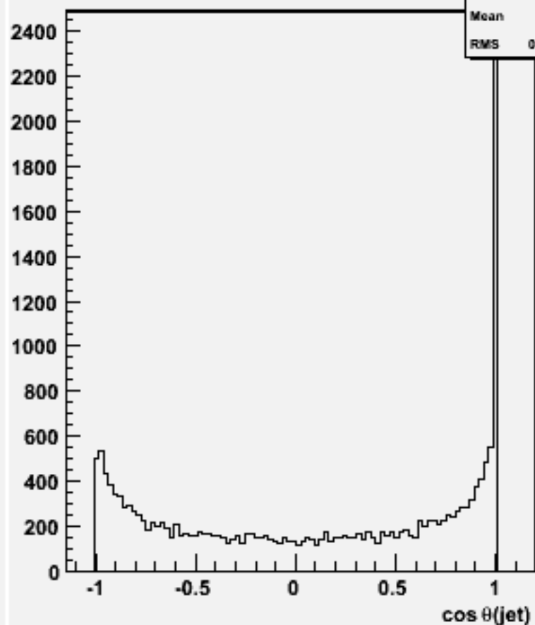
cos \theta for 2-jets :w102241 n2n2e3e3dd_o
