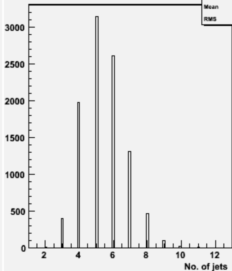
No. jets (ycut=0.001) : w102241 n2n2e3e3dd_o
