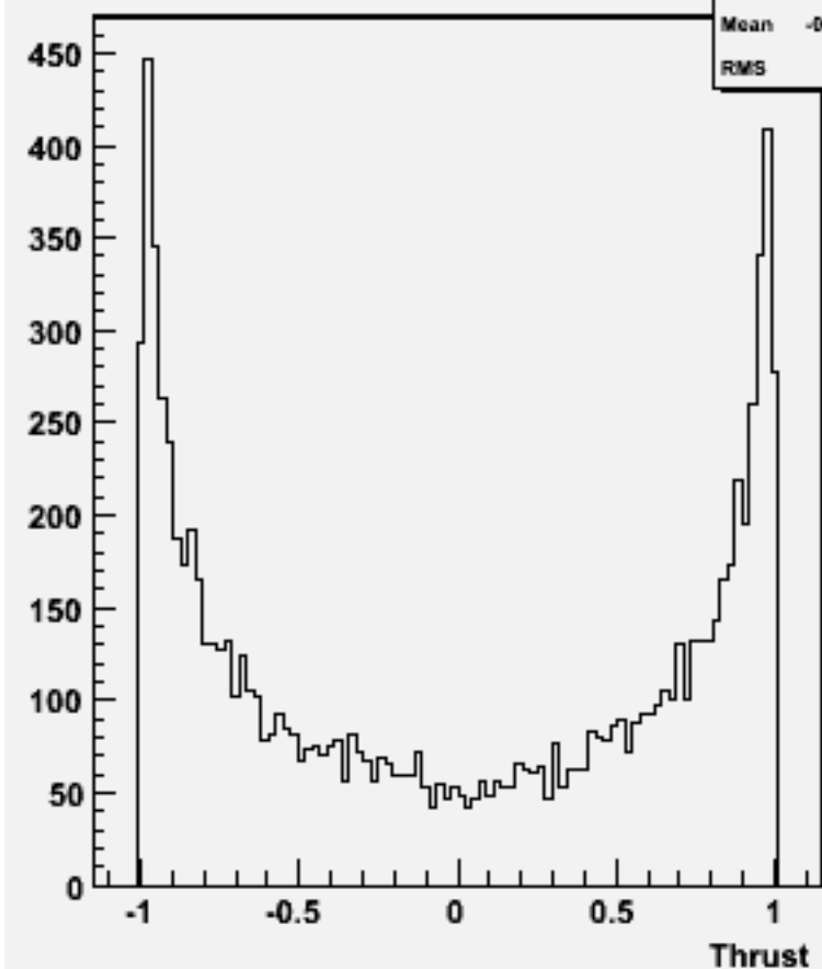
cos \Theta (thrust) w102241 n2n2e3e3dd_o
