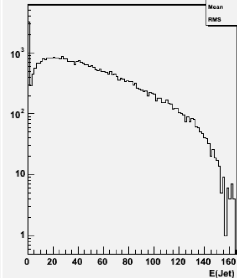
Jet energies(All jets)w102241 n2n2e3e3dd_o
