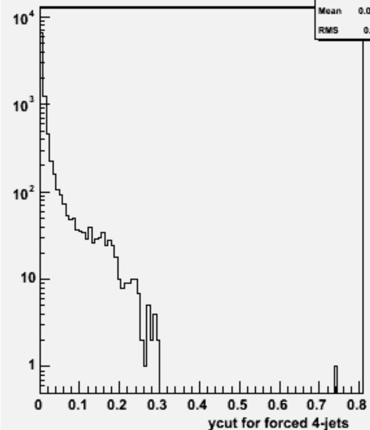
Ycut for 4-jets :w102241 n2n2e3e3dd_o
