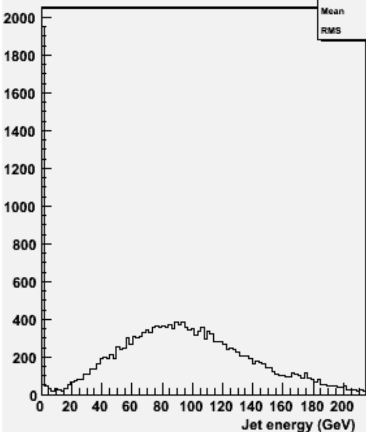
energy for 2-jets :w102241 n2n2e3e3dd_o
