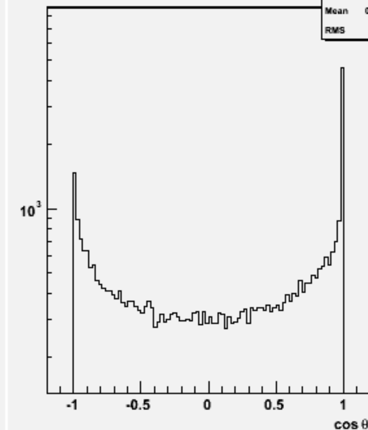
Jet cos \theta (All jets)w102241 n2n2e3e3dd_o
