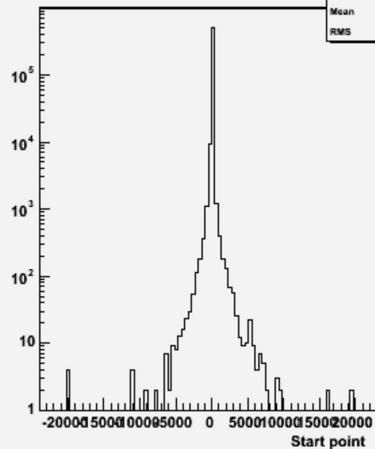
Start point Z : w102241 n2n2e3e3dd_o
