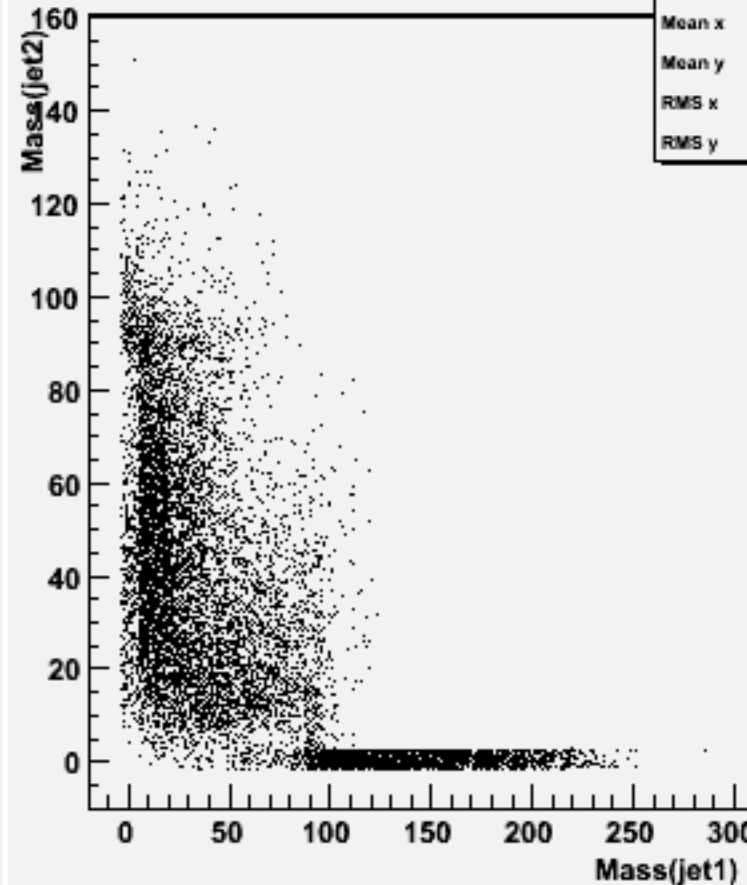
Jet mass for forced 2-jets : w102241 n2n2e3e3dd_o
