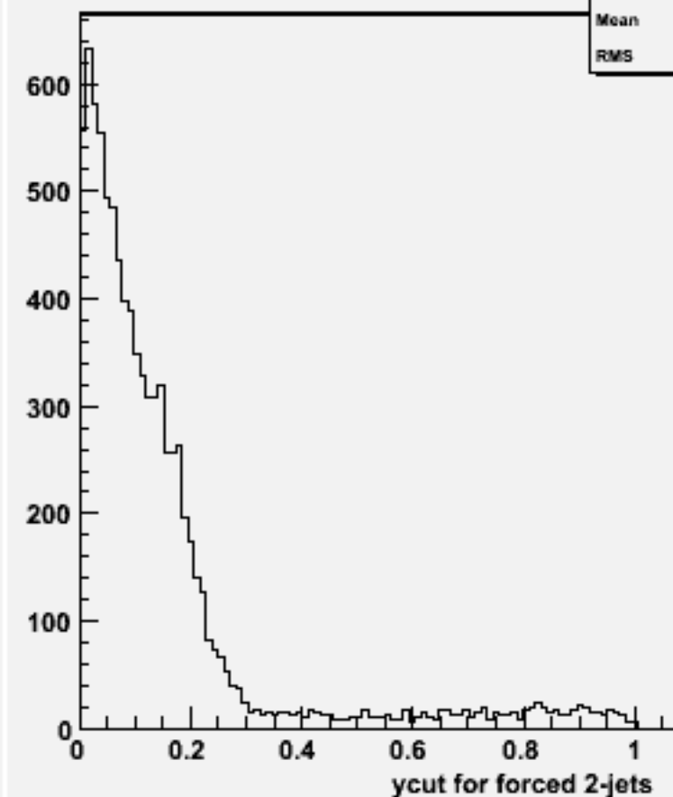
Ycut for 2-jets :w102241 n2n2e3e3dd_o
