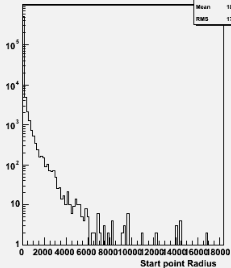
Start point R : w102241 n2n2e3e3dd_o
