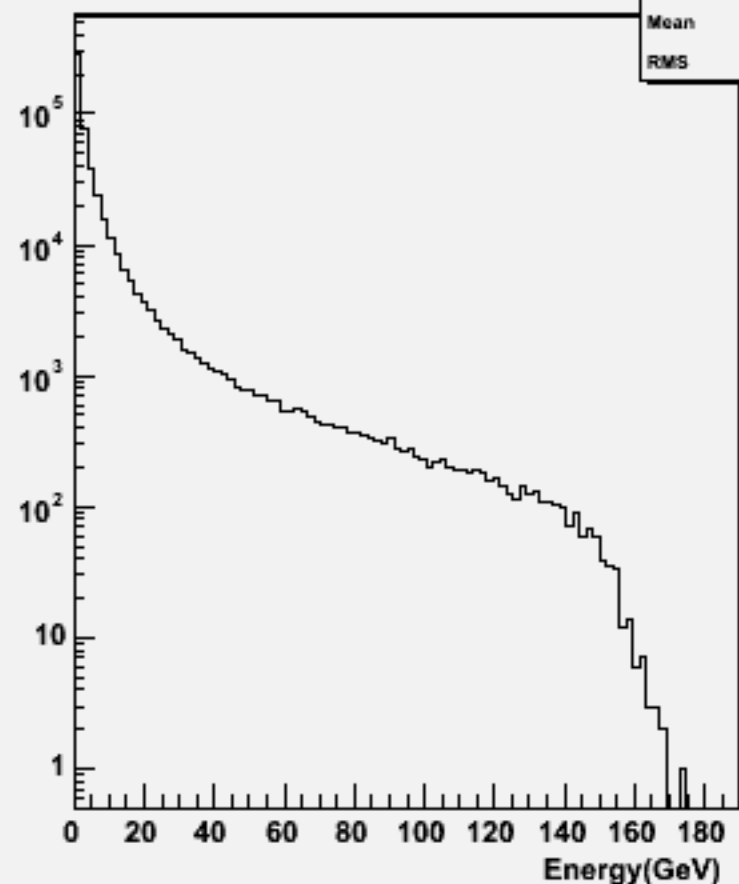
Particle Energy : w102241 n2n2e3e3dd_o
