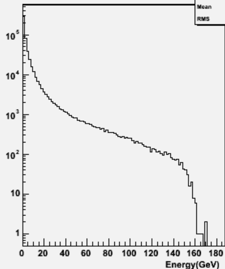
Particle Energy : w102240 n2n2e3e3dd_o
