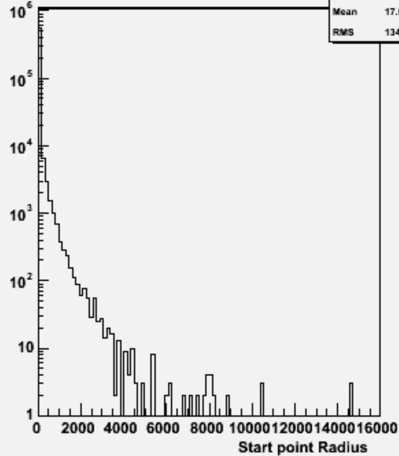
Start point R : w102233 n2n2e1e1bb_o
