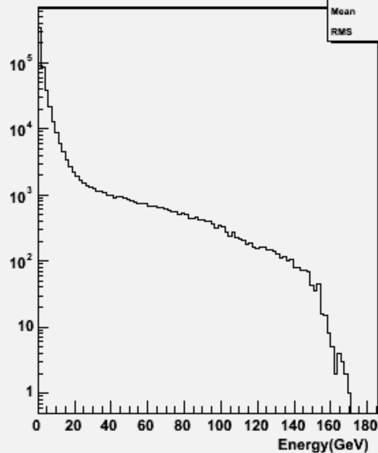
Particle Energy : w102233 n2n2e1e1bb_o
