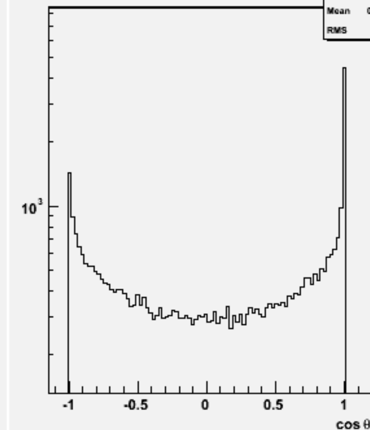
Jet cos \theta (All jets)w102233 n2n2e1e1bb_o
