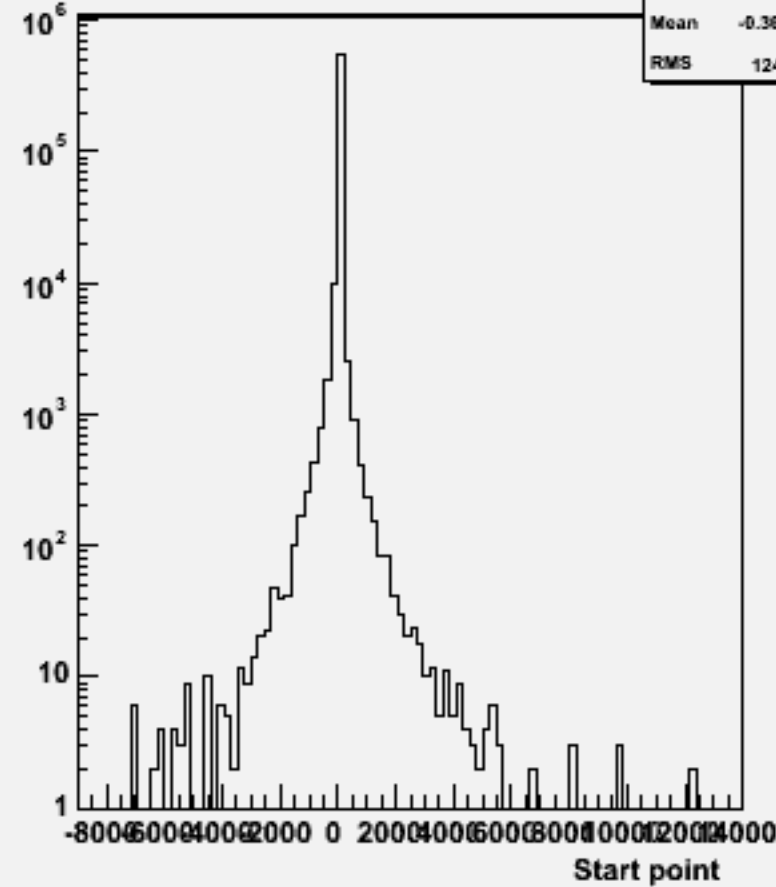
Start point Z : w102233 n2n2e1e1bb_o
