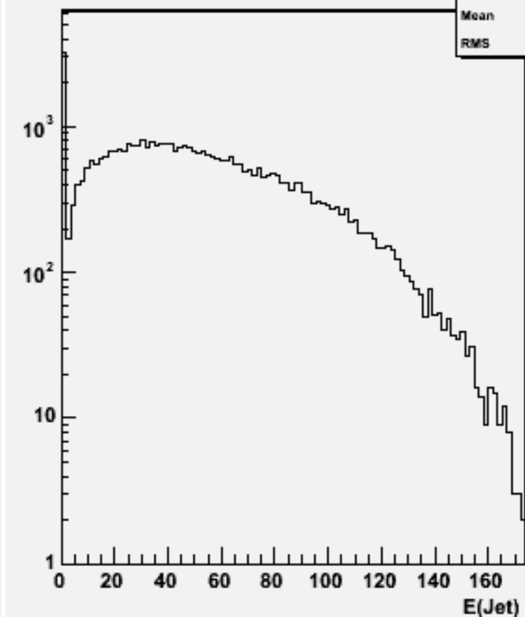
Jet energies(All jets)w102233 n2n2e1e1bb_o
