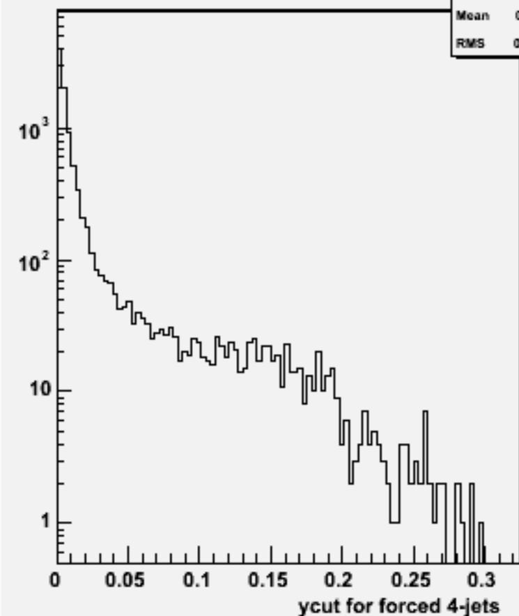
Ycut for 4-jets :w102233 n2n2e1e1bb_o
