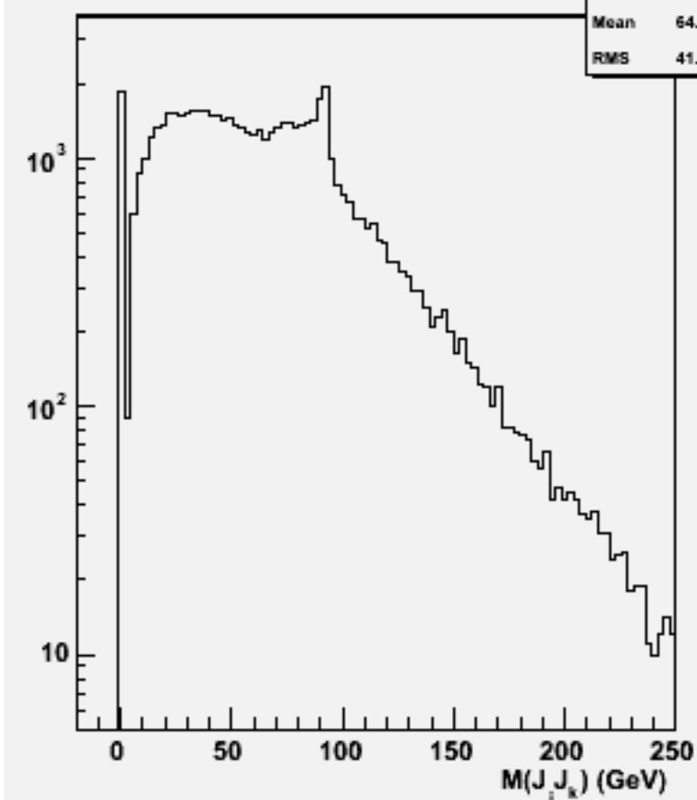
2jets mass(All comb)w102233 n2n2e1e1bb_o
