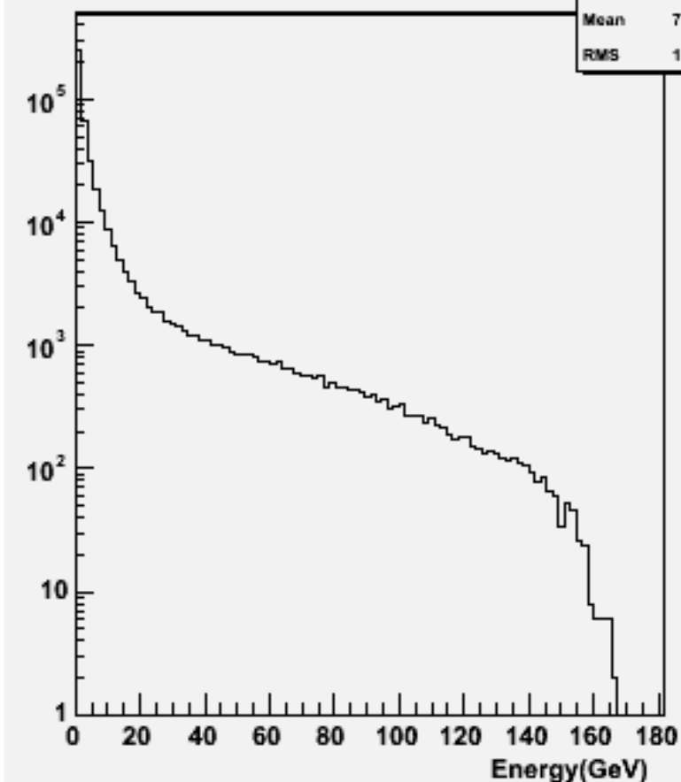
Particle Energy : w102229 n2n2e1e1ss_o
