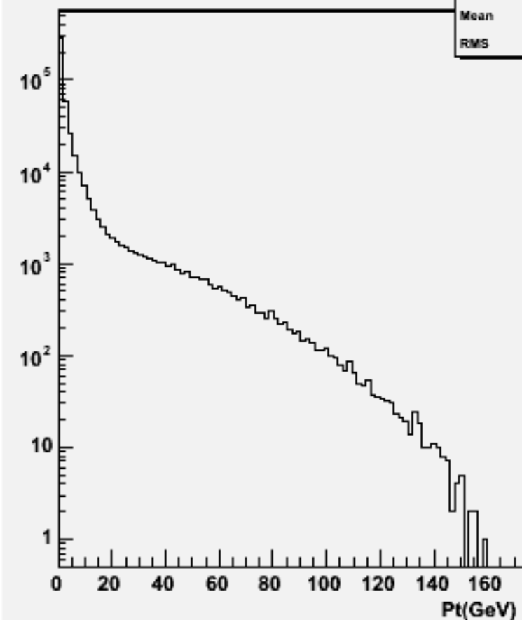
Particle Pt : w102229 n2n2e1e1ss_o
