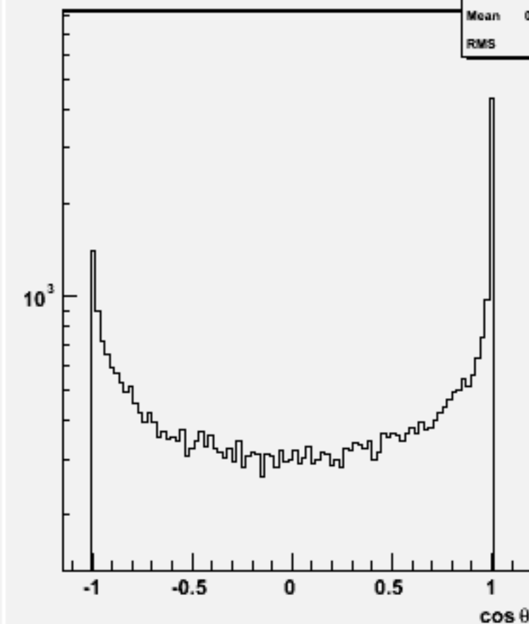
Jet cos \theta (All jets)w102229 n2n2e1e1ss_o
