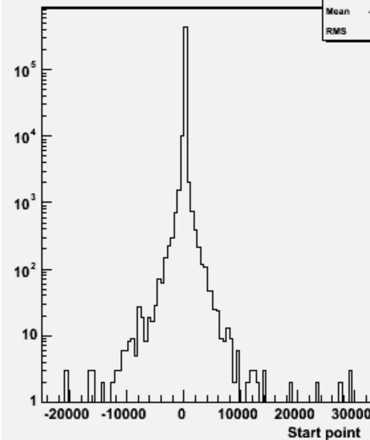
Start point Z : w102229 n2n2e1e1ss_o
