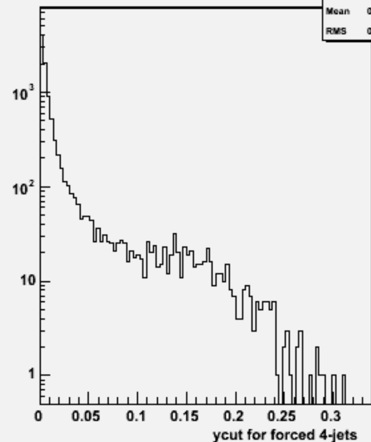
Ycut for 4-jets :w102229 n2n2e1e1ss_o
