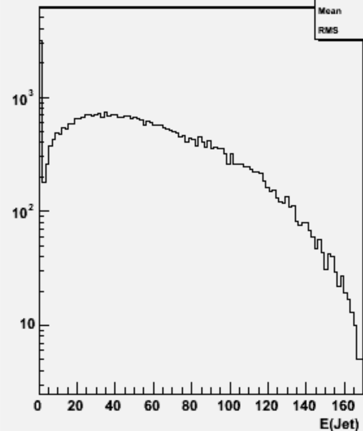
Jet energies(All jets)w102229 n2n2e1e1ss_o
