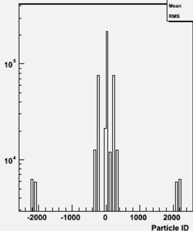
Particle ID : w102229 n2n2e1e1ss_o
