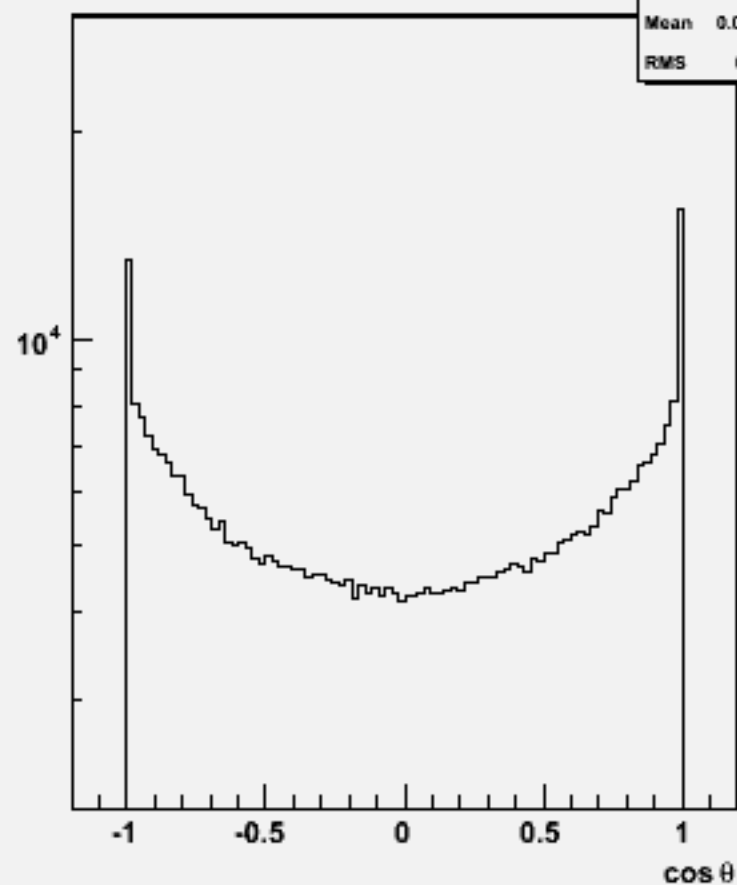
Particle cos \theta : w102229 n2n2e1e1ss_o
