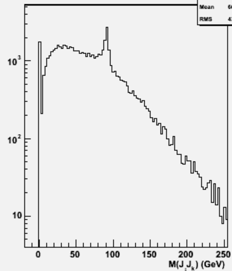
2jets mass(All comb)w102229 n2n2e1e1ss_o
