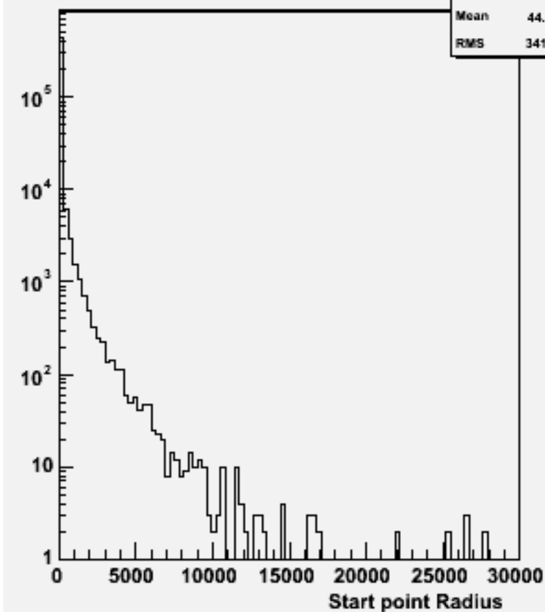
Start point R : w102229 n2n2e1e1ss_o
