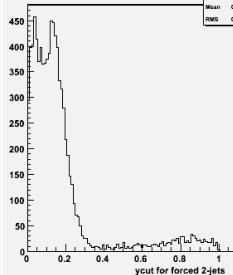
Ycut for 2-jets :w102228 n2n2e1e1ss_o
