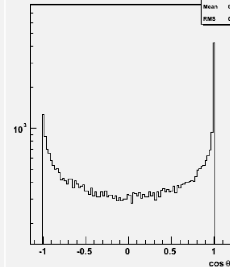
Jet cos \theta (All jets)w102228 n2n2e1e1ss_o
