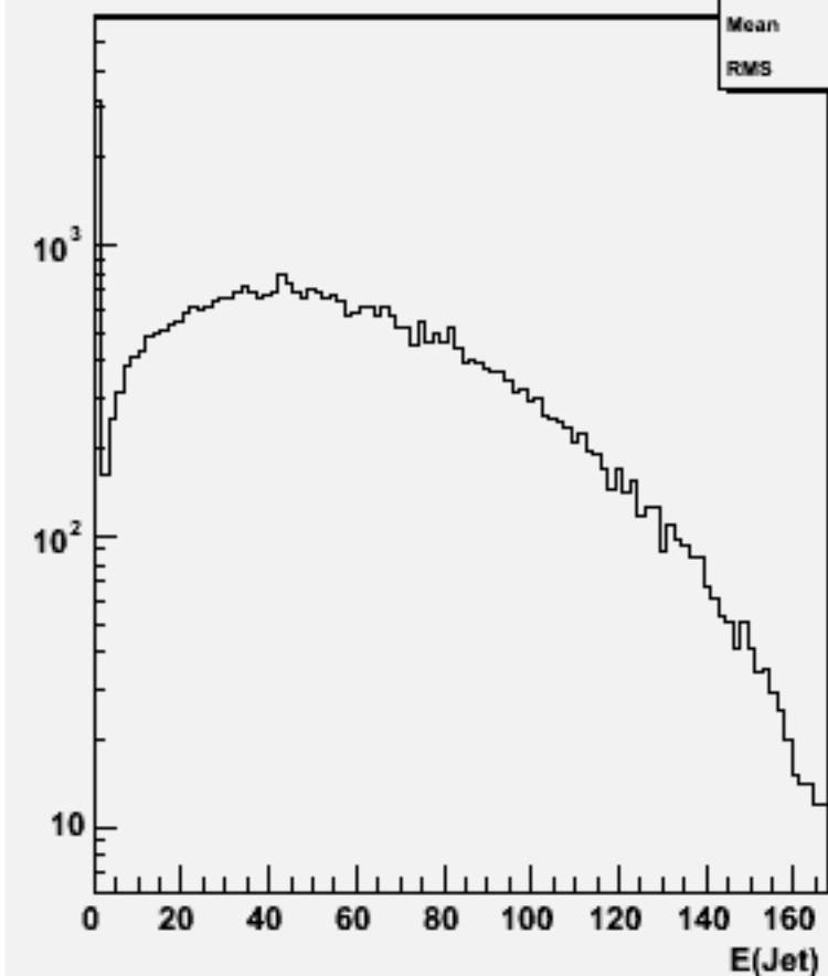
Jet energies(All jets)w102228 n2n2e1e1ss_o
