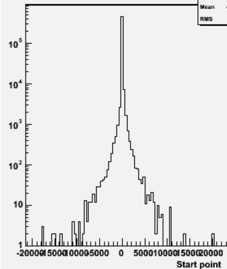
Start point Z : w102228 n2n2e1e1ss_o
