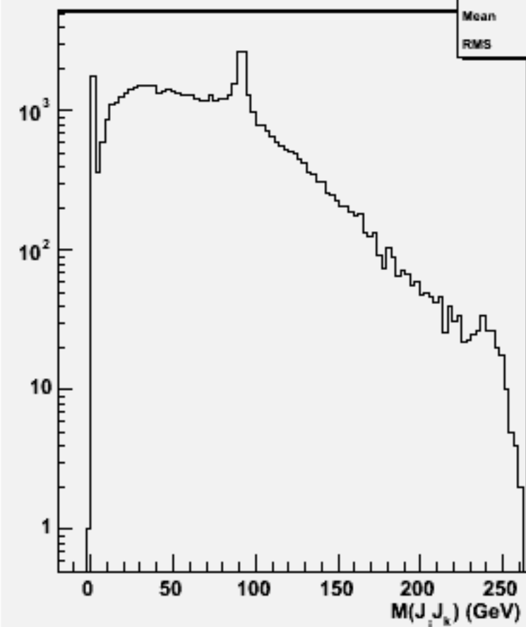
2jets mass(All comb)w102228 n2n2e1e1ss_o
