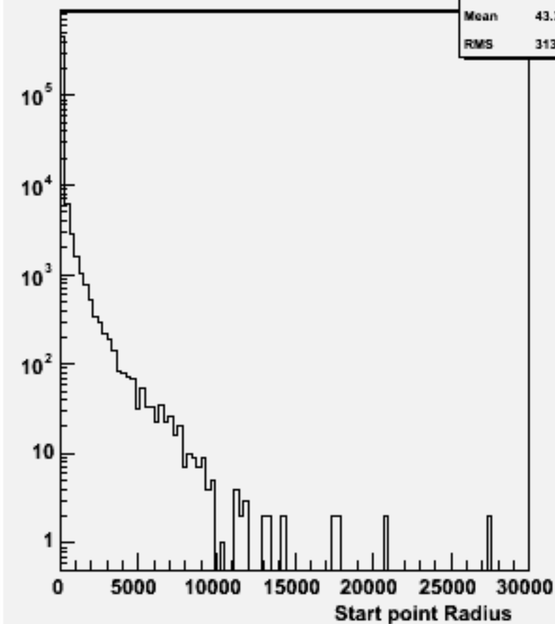
Start point R : w102228 n2n2e1e1ss_o
