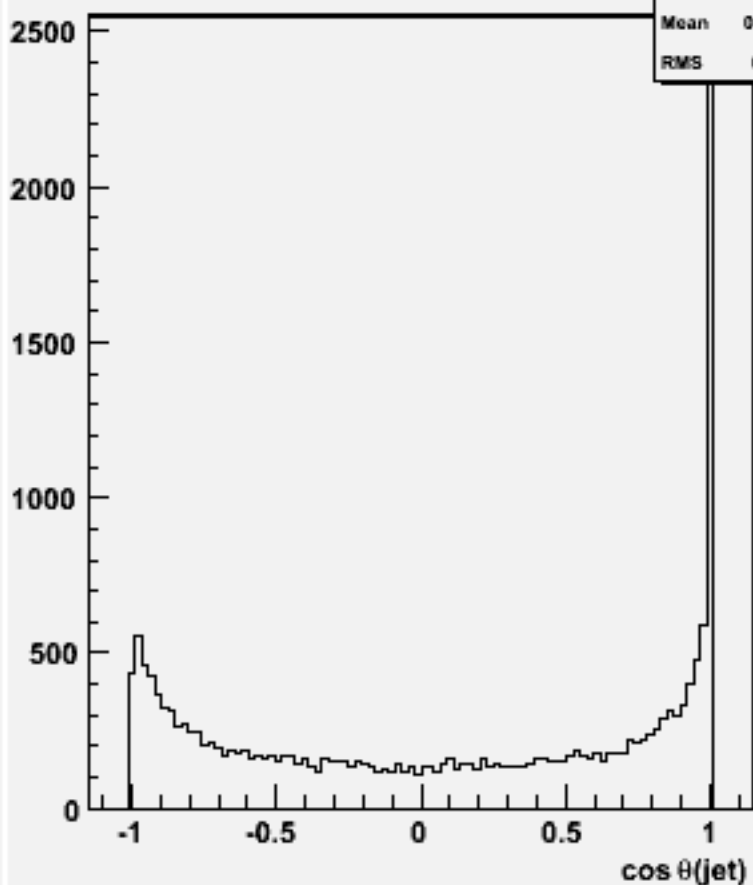
cos \theta for 2-jets :w102228 n2n2e1e1ss_o
