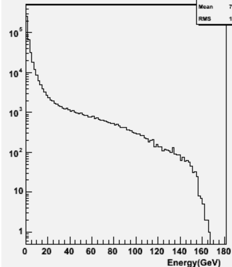
Particle Energy : w102228 n2n2e1e1ss_o
