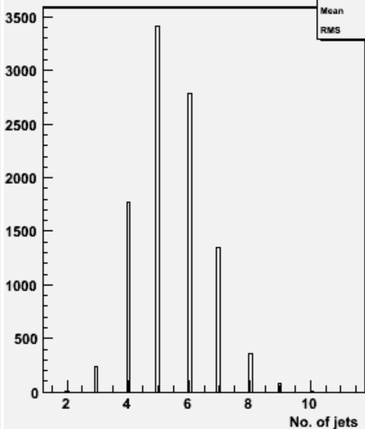
No. jets (ycut=0.001) : w102228 n2n2e1e1ss_o
