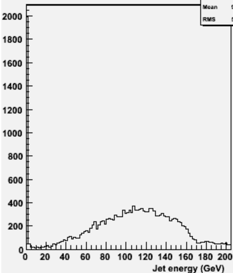
energy for 2-jets :w102228 n2n2e1e1ss_o
