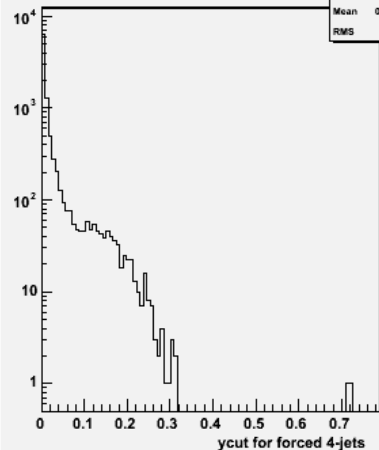
Ycut for 4-jets :w102228 n2n2e1e1ss_o
