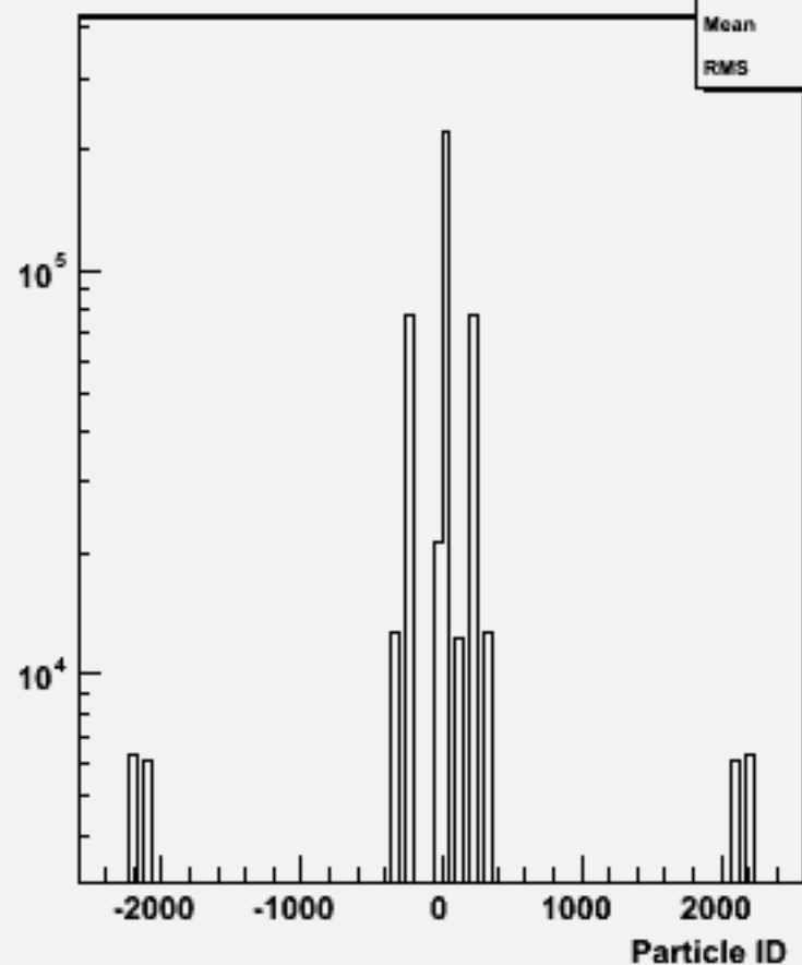
Particle ID : w102228 n2n2e1e1ss_o
