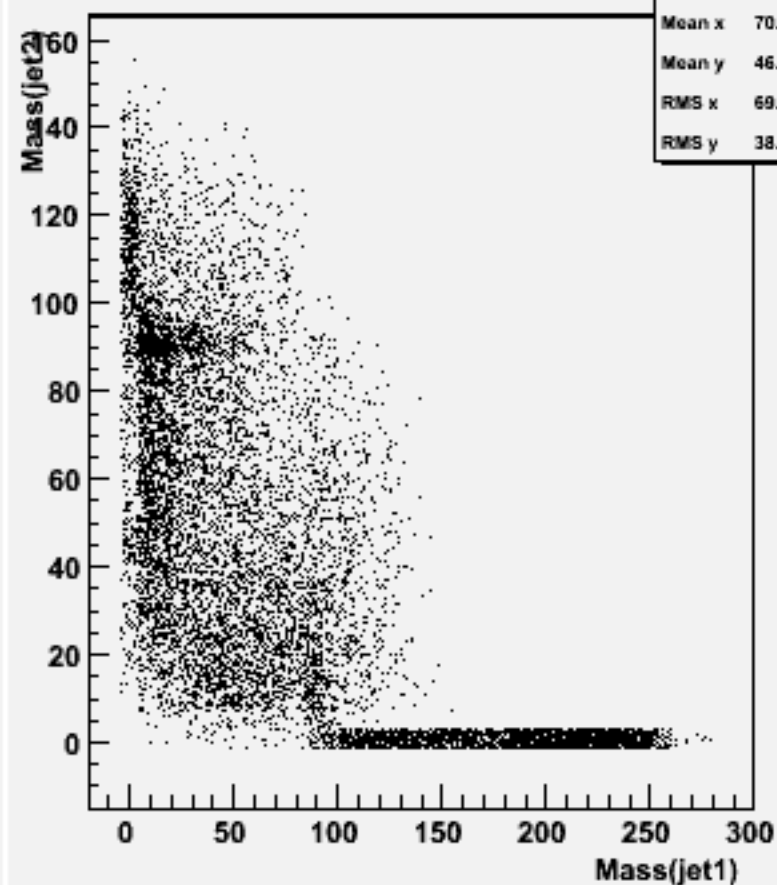
Jet mass for forced 2-jets : w102228 n2n2e1e1ss_o
