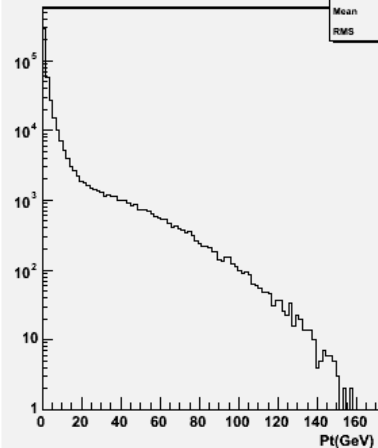
Particle Pt : w102228 n2n2e1e1ss_o
