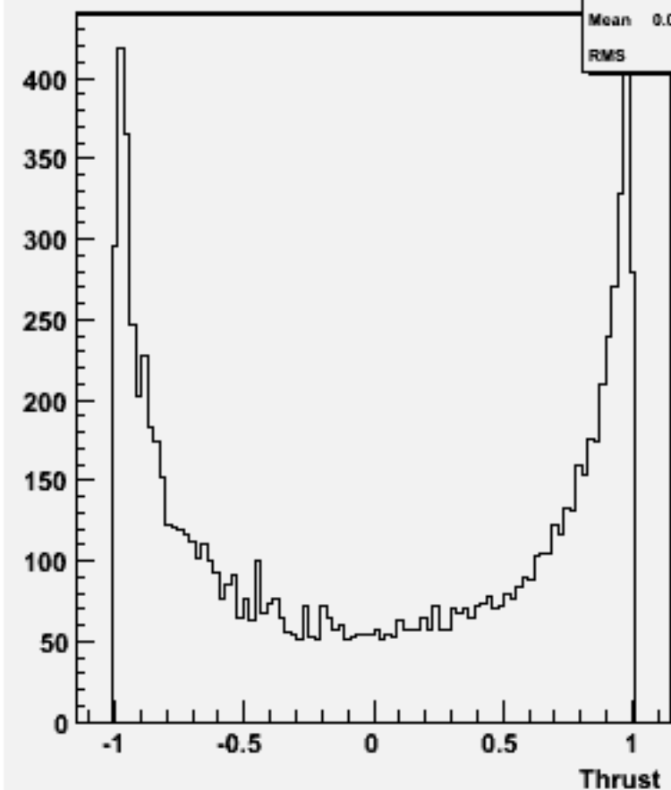
cos \Theta (thrust) w102228 n2n2e1e1ss_o
