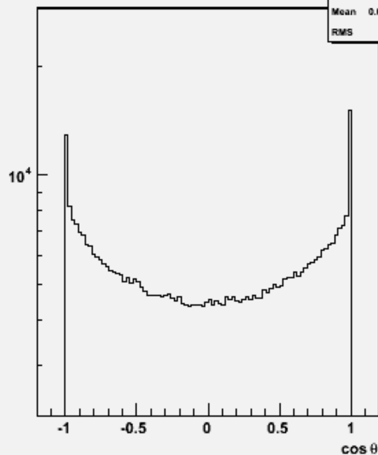
Particle cosθ : w102228 n2n2e1e1ss_o
