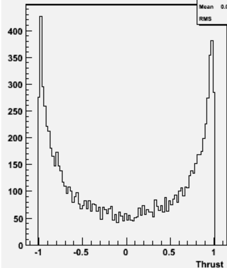
cos \Theta (thrust) w102224 n2n2e1e1dd_o
