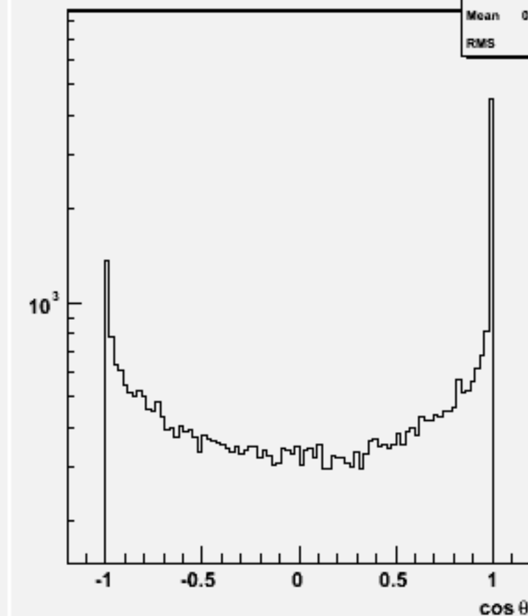
Jet cos \theta (All jets)w102224 n2n2e1e1dd_o
