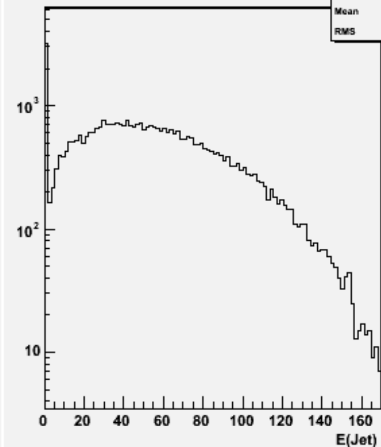
Jet energies(All jets)w102224 n2n2e1e1dd_o
