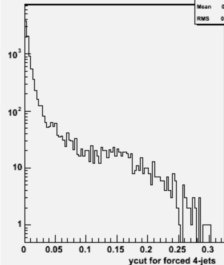
Ycut for 4-jets :w102224 n2n2e1e1dd_o
