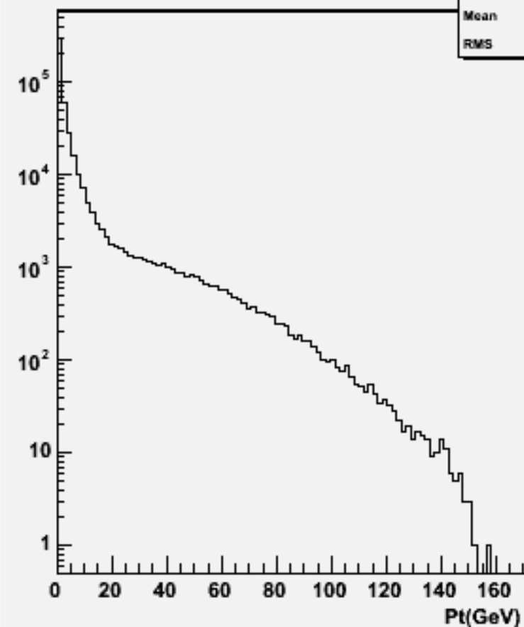
Start point Z : w102224 n2n2e1e1dd_o
