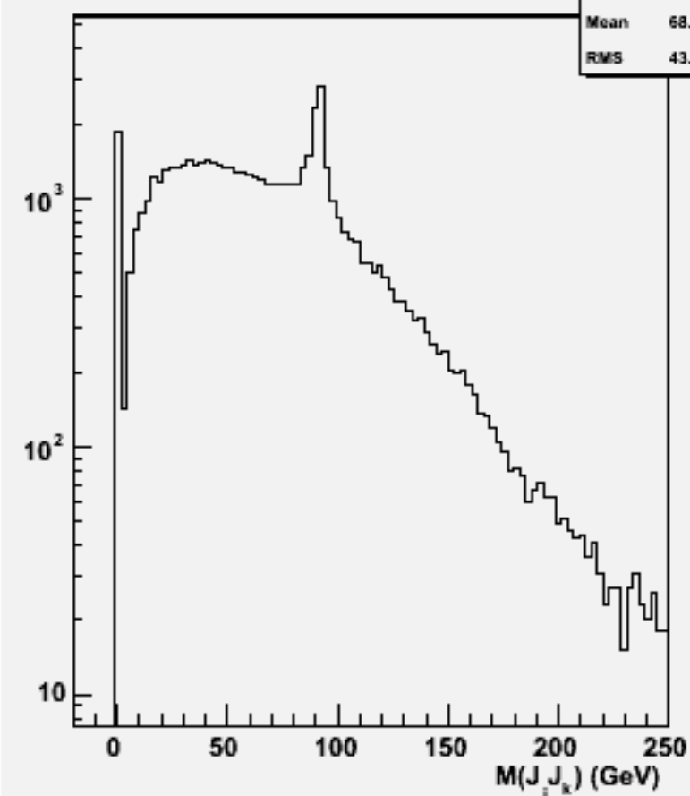
2jets mass(All comb)w102224 n2n2e1e1dd_o
