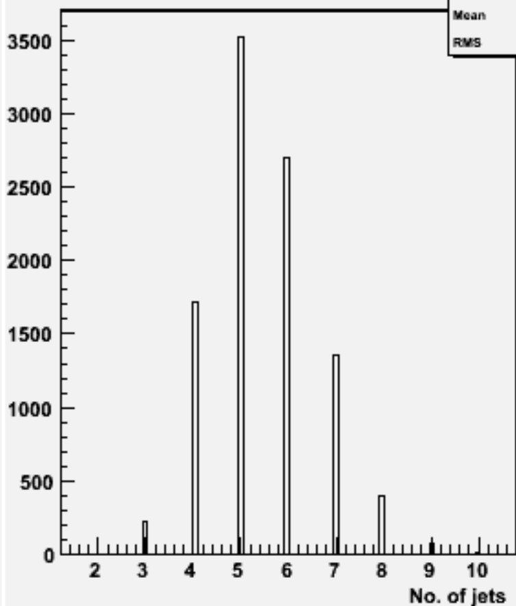
No. jets (ycut=0.001) : w102224 n2n2e1e1dd_o
