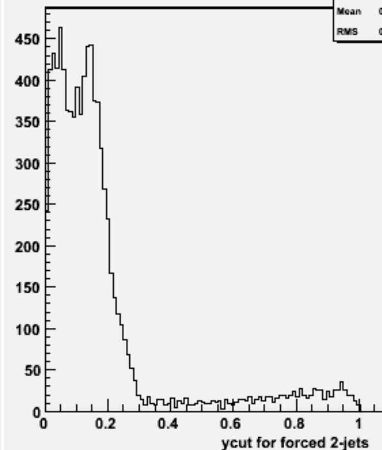
Ycut for 2-jets :w102224 n2n2e1e1dd_o
