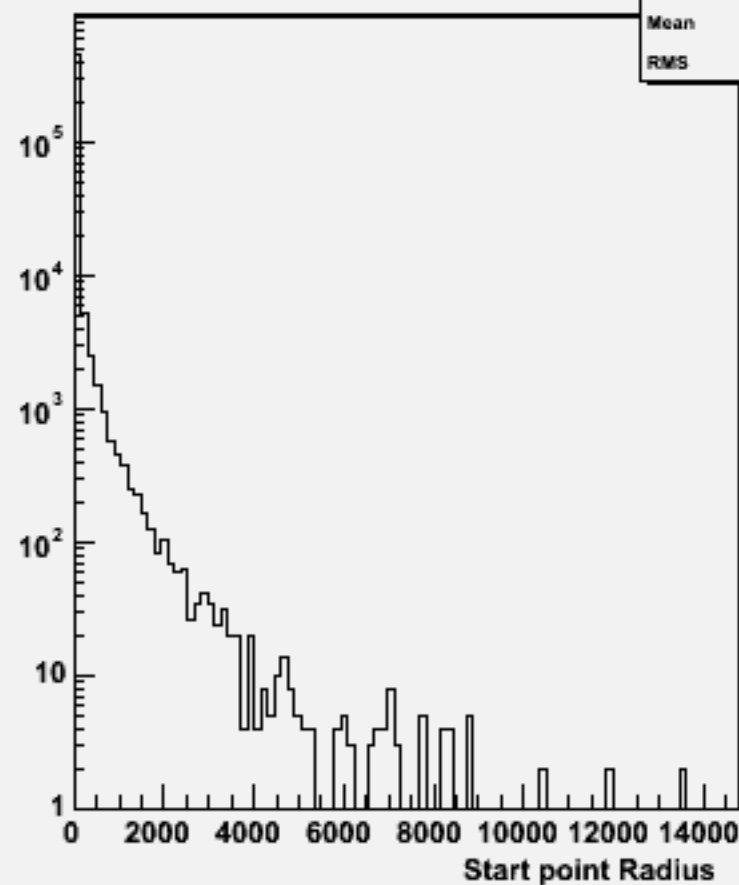
Start point R : w102224 n2n2e1e1dd_o
