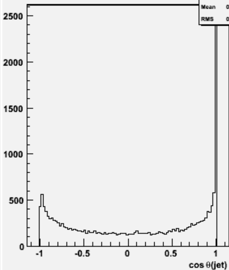
cos \theta for 2-jets :w102224 n2n2e1e1dd_o
