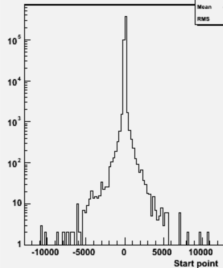
Start point Z : w102224 n2n2e1e1dd_o
