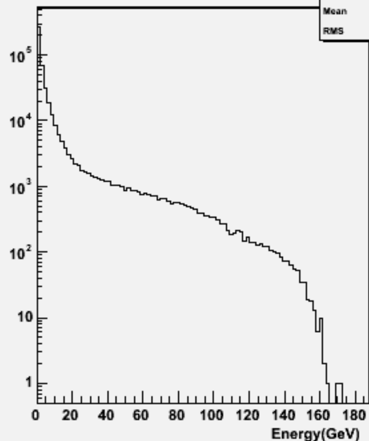
Start point R : w102224 n2n2e1e1dd_o
