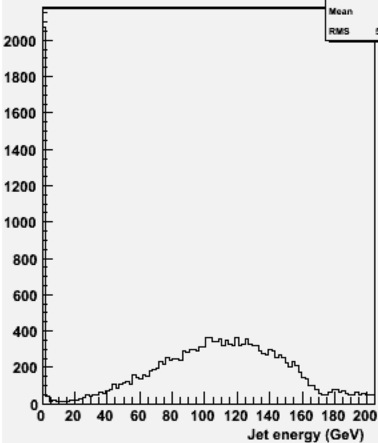
energy for 2-jets :w102224 n2n2e1e1dd_o
