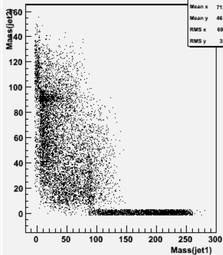
Jet mass for forced 2-jets : w102224 n2n2e1e1dd_o
