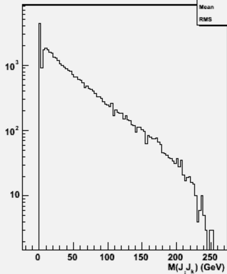
2jets mass(All comb)w102222 n2n2e1e1e3e3_o
