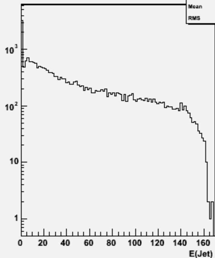
Jet energies(All jets)w102222 n2n2e1e1e3e3_o
