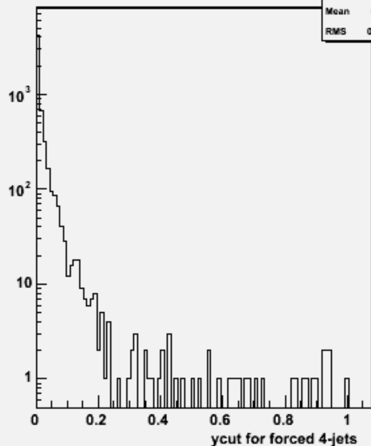
Ycut for 4-jets :w102222 n2n2e1e1e3e3_o
