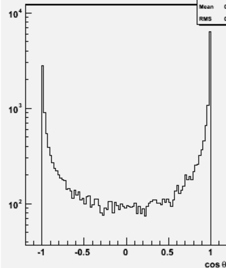
Jet cos \theta (All jets)w102222 n2n2e1e1e3e3_o
