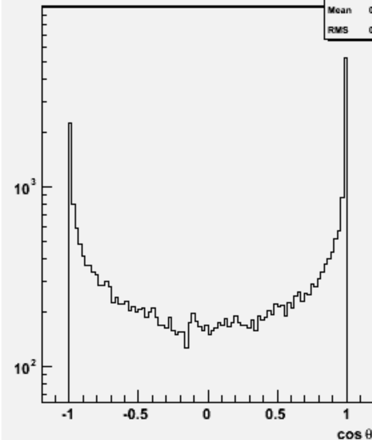
Jet cos \theta (All jets)w102221 n2n2e1e1e3e3_o
