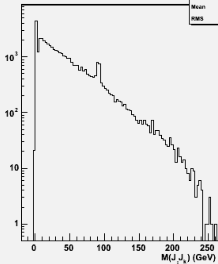
2jets mass(All comb)w102221 n2n2e1e1e3e3_o
