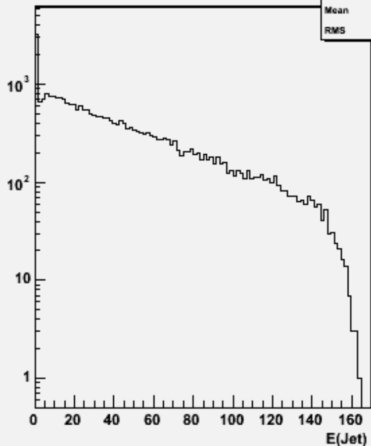
Jet energies(All jets)w102221 n2n2e1e1e3e3_o
